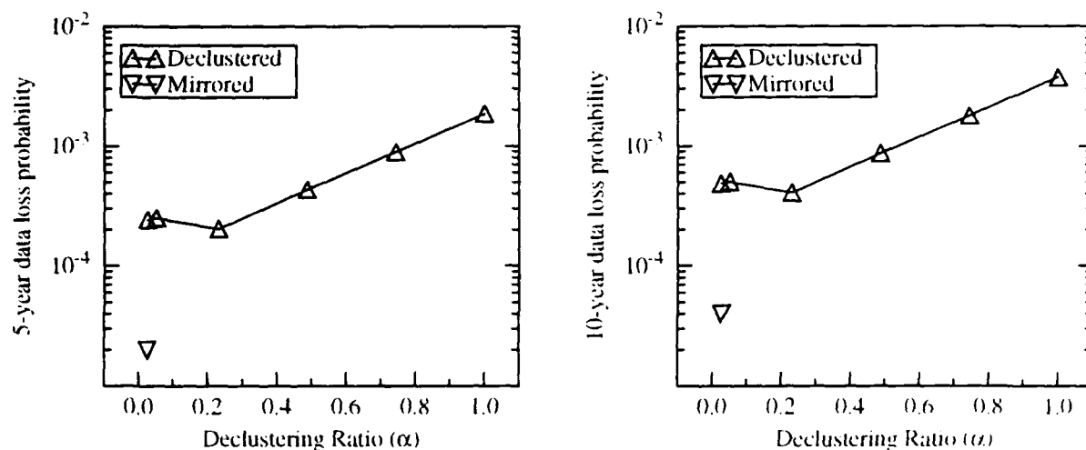
Figure 19: Varying the declustering ratio: probability of data loss within (a) 5 years and (b) 10 years. Note that the Y-axis is log-scaled.
