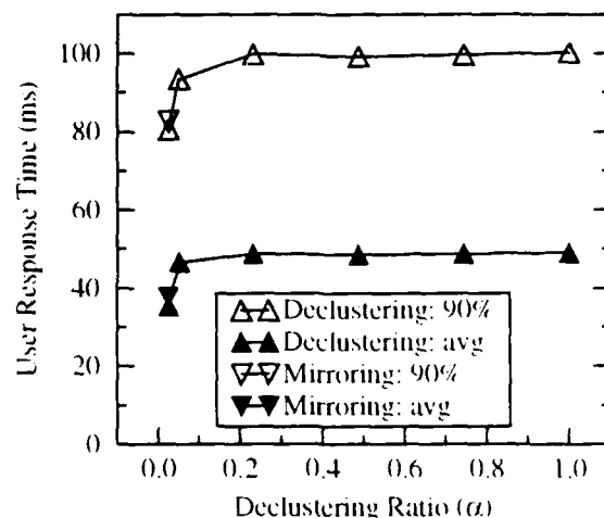
Figure 16: Varying the declustering ratio: user response time in fault-free mode.
