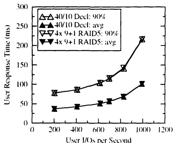
Figure 11: Comparing RAID Level 5 to parity declustering: fault-free performance.
