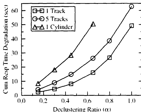
Figure 10: Cumulative response time degradation during reconstruction.
