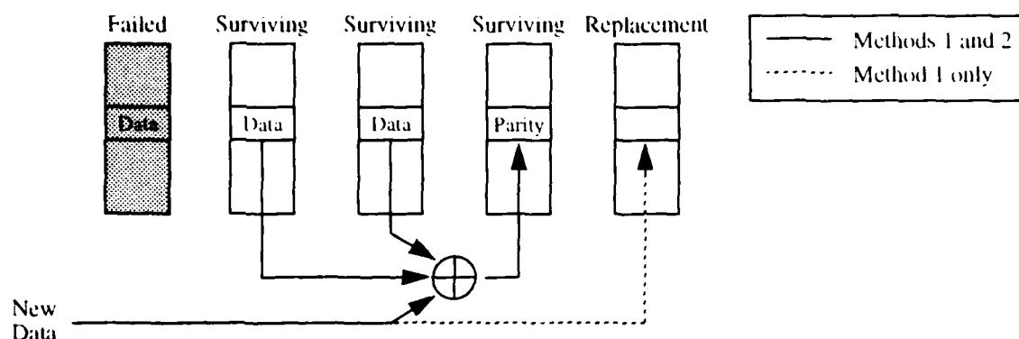
Figure 20: Two methods for servicing a user write to as-yet unreconstructed data.
