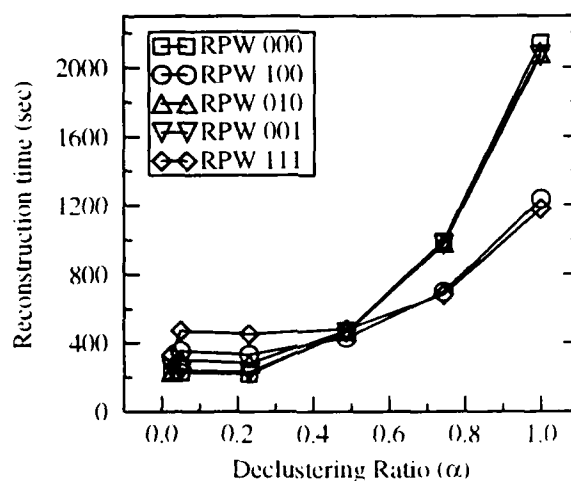
Figure 22: Reconstruction time for five combinations of reconstruction options.
