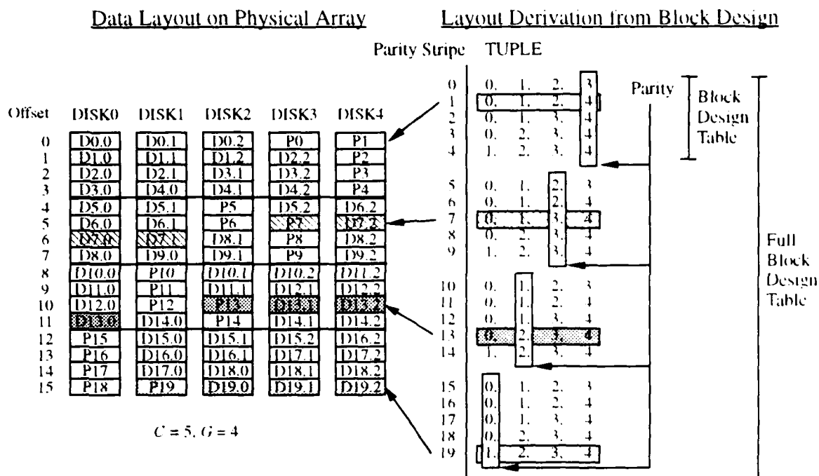
Figure 5: Full block design table for a parity declustering organization.
