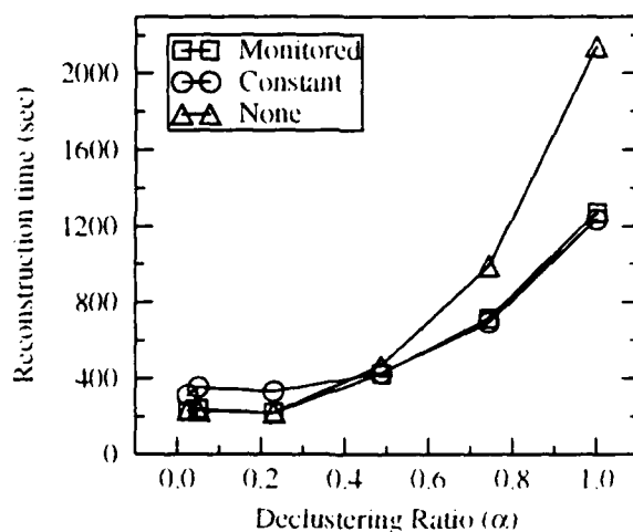
Figure 24: Evaluating monitored redirection of reads: reconstruction time.
