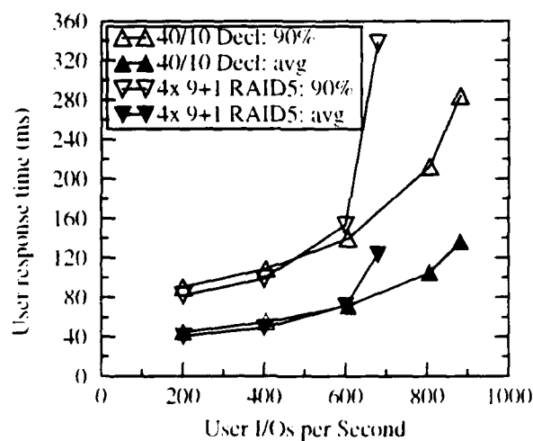
Figure 13: Comparing RAID Level 5 to parity declustering: response time during reconstruction.
