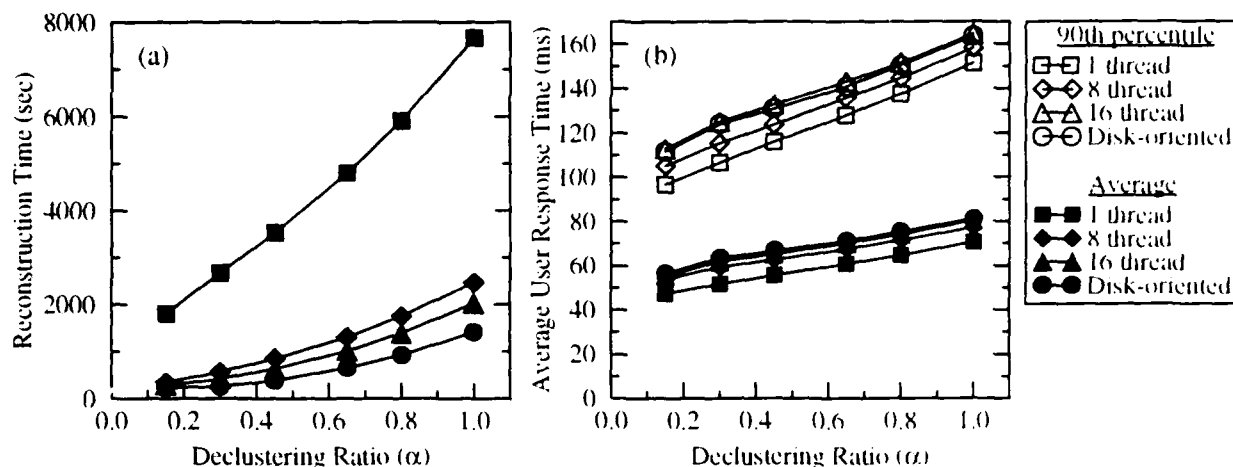
Figure 8: Comparing reconstruction algorithms: (a) reconstruction time and (b) average user response time during reconstruction.
