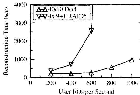
Figure 14: Comparing RAID Level 5 to parity declustering: reconstruction time.
