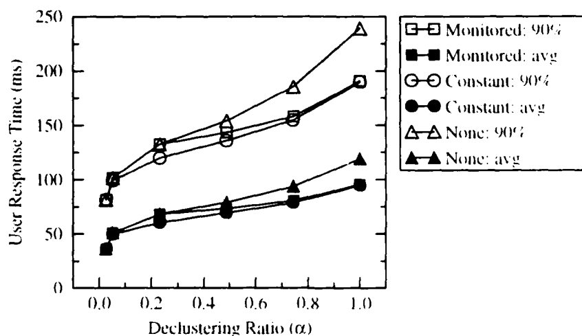
Figure 23: Evaluating monitored redirection of reads: response time.
