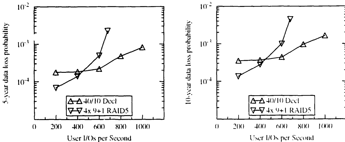
Figure 15: Comparing RAID Level 5 to parity declustering: probability of data loss within (a) 5 years and (b) 10 years. Note that the Y-axis is log-scaled.
