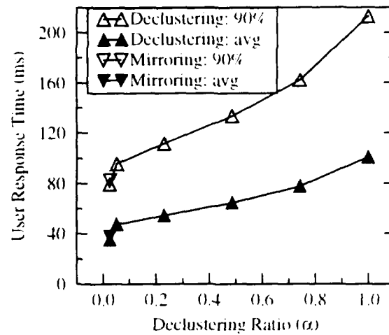
Figure 17: Varying the declustering ratio: user response time in degraded mode.
