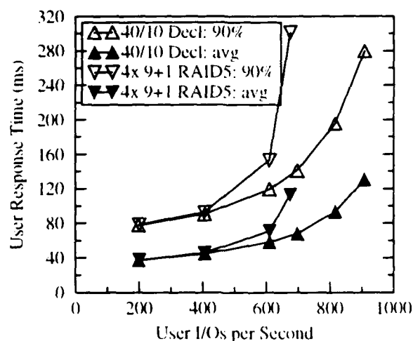
Figure 12: Comparing RAID Level 5 to parity declustering: degraded-mode performance.
