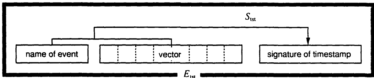
Figure 5 A sealed timestamp consists of the encryption of the name of an event, its timestamp vector, and a signature on this pair. The signature certifies that this vector belongs to this event, and also protects against guessing the plaintext: verifying a guessed vector requires guessing the correct signature.
