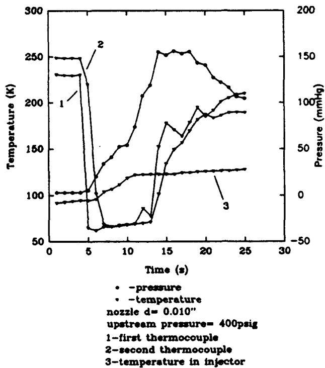
Figure A.7 Temperature and Pressure in Blow-Down Tube
