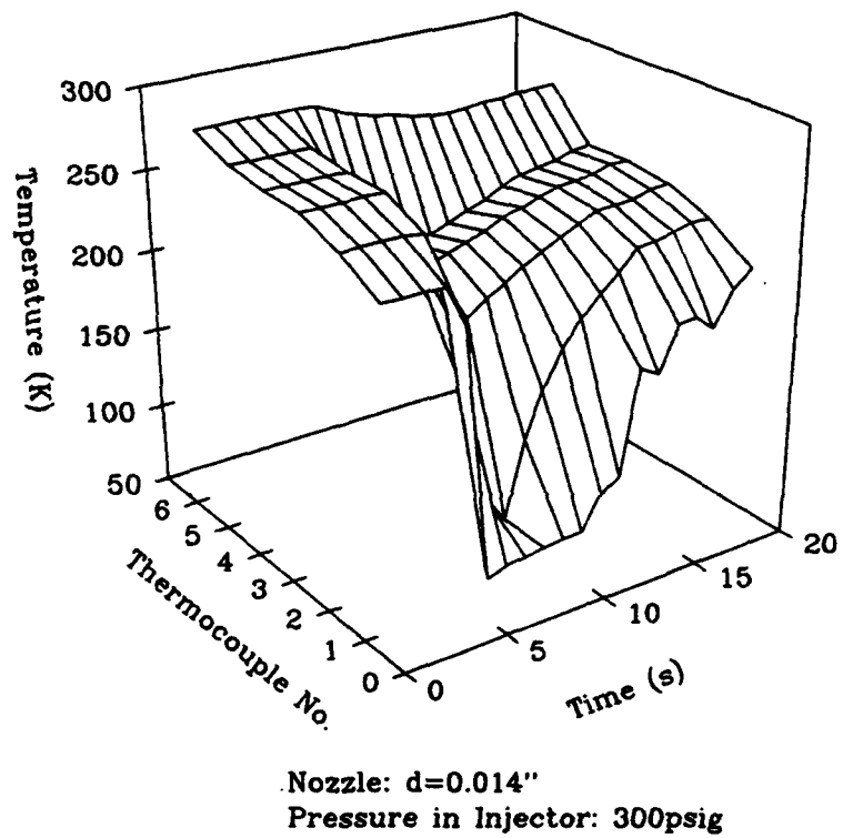
Figure A.16 Transient Temperature Field
