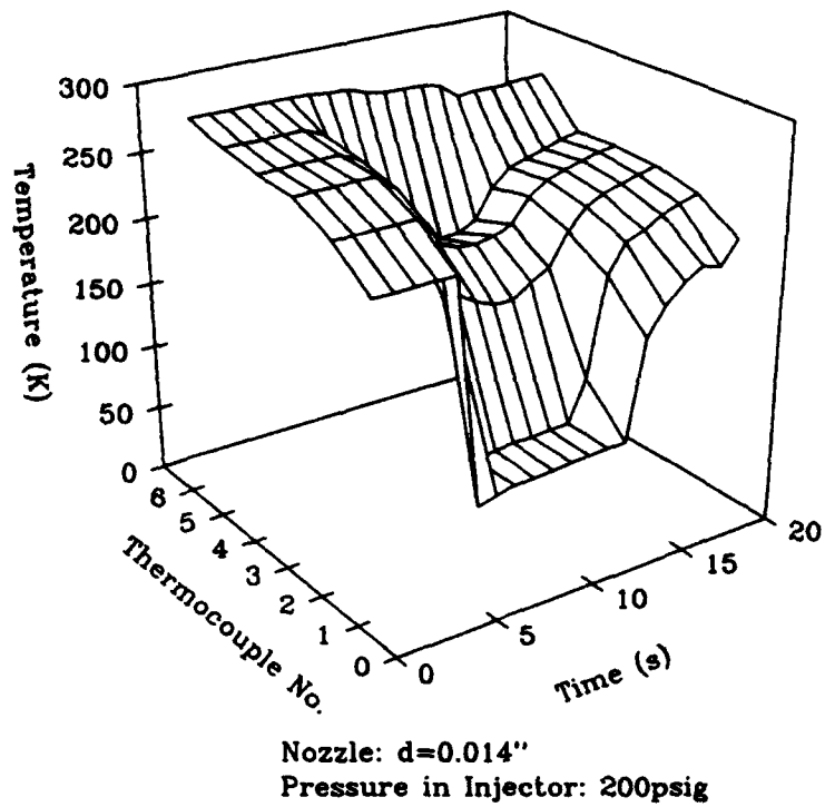
Figure A.15 Transient Temperature Field
