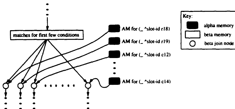
Figure 2: Part of the Rete network for Assembler.
