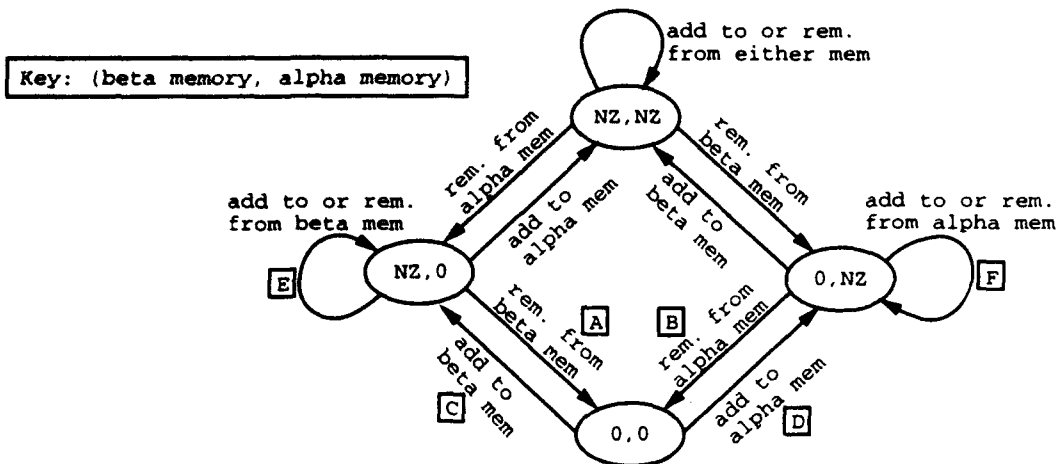
Figure 3: Possible states of a join node and its alpha and beta memories.
