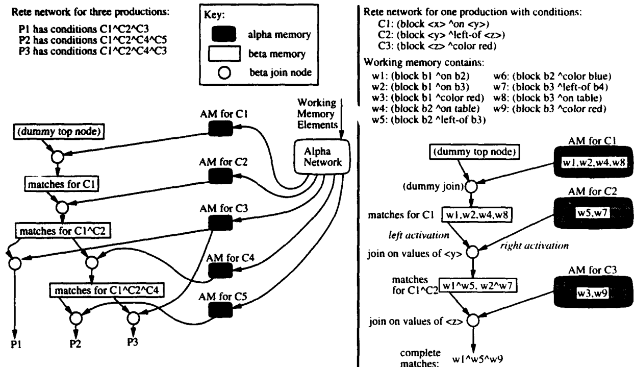
Figure 1: Example network used by Rete for several productions (left) and instantiated network for one production (right).
