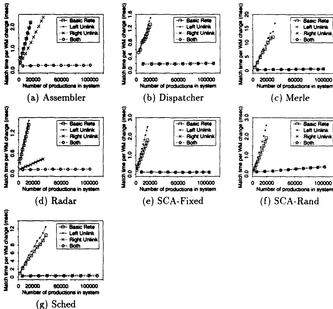
Figure 4: Performance of the matcher on each of the systems.
