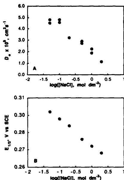
Figure 3. Effect of the ionic strength on the electron diffusion coefficient (A) and the half-wave potential of the POs-EA polymer (B). The conditions are the same as in Figure 2.
