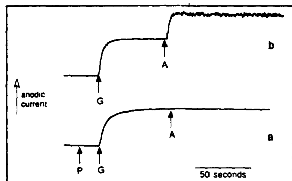
Figure 10. Effect of adding hydrogen peroxide on the current of a three layers electrode: additions of glucose (5 mM final concentration) "G" and ascorbate (0.1 mM final concentration) "A" (a) in the presence of and (b) in the absence of H_2O_2 ("P"). 0.4 V (SCE).
