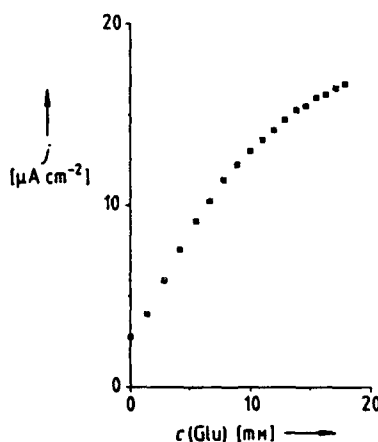
Fig. 3. Glucose concentration dependence of the current density at 0.45 V for the glucose oxidase/1 graphite electrode system in 0.15 M NaHEPES at pH 7 and 9.9 units catalase mL -1 .
