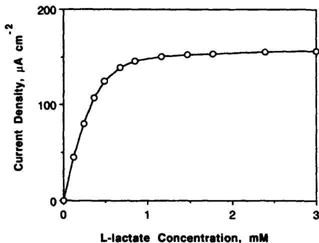
FIGURE 4. Dependence of the current density on lactate concentration for a lactate oxidase bilayer cathode. The lactate oxidase loading in the outer layer is 100 \mu\text{g} . pH 7.4, 0.0 mV versus SCE, 1000 rpm.
