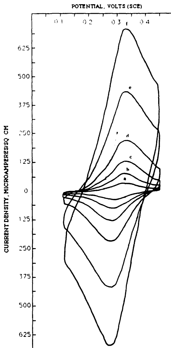
FIGURE 9 (a) Cyclic voltammograms at different scan rates for nonquaternized POs · NH 2 adsorbed on abraded graphite (electrode surface area 0.008 cm 2 ). Scan rates: a) 2 mV/s, b) 5 mV/s, c) 10 mV/s, d) 20 mV/s, e) 50 mV/s, and f) 100 mV/s. 0.15 M NaHEPES, pH 7. (b) Cyclic voltammograms at different scan rates for nonquaternized POs · NH 2 adsorbed on gold (electrode surface area 0.002 cm 2 ). Scan rates: a) 5 mV/s, b) 10 mV/s, c) 20 mV/s, d) 50 mV/s, e) 100 mV/s, and f) 200 mV/s. 0.15 M NaHEPES, pH 7.
