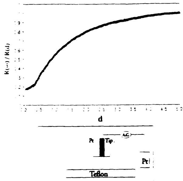
Figure 5. Conductance-distance curve for a 25- \mu m-diameter platinum UME over a Teflon surface in 1 mM KCl. Filled triangles are experiment and line is theory.
