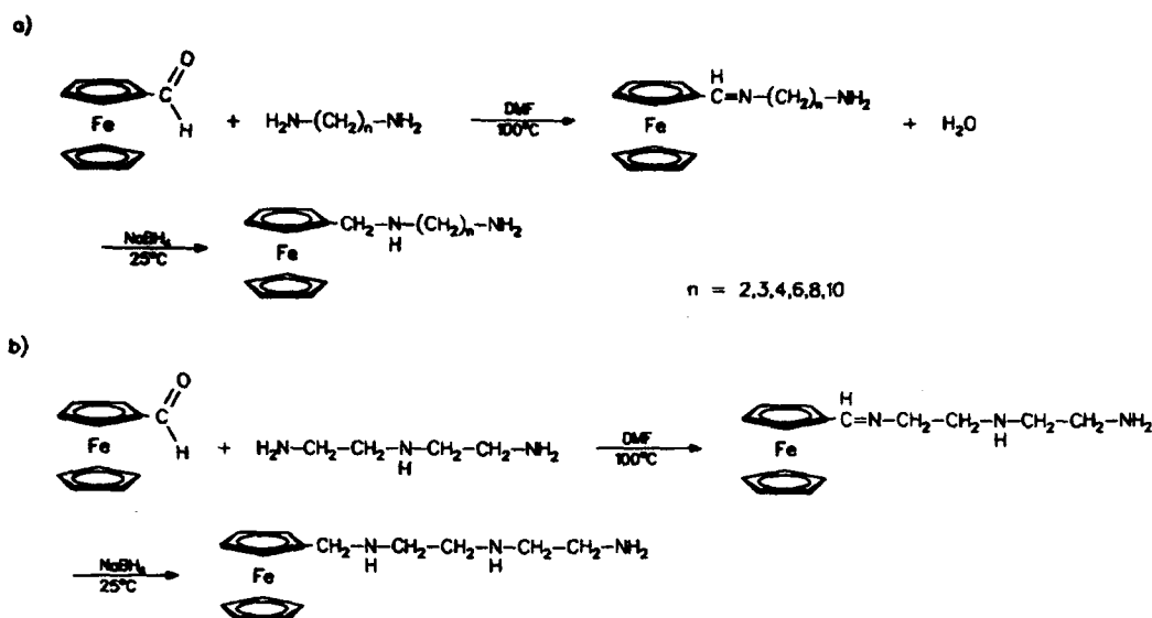
Figure 1. Synthesis of ferrocene amines with spacer chains separating the redox and amine functions.
