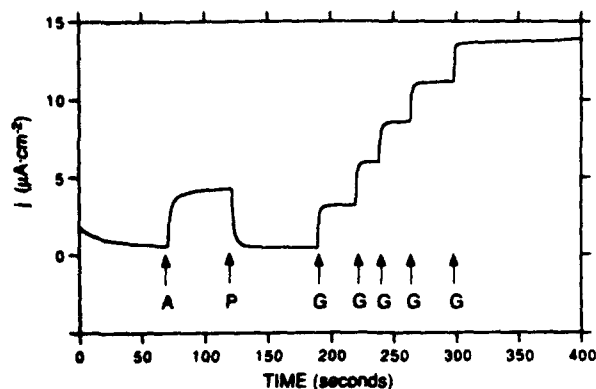
Figure 9. Elimination of interferants in a two-layer electrode. "A" denotes injection of ascorbate (0.1 mM final concentration); "P" denotes injection of hydrogen peroxide (0.2 mM final concentration); "G" denotes injection of glucose, increasing its concentration in 1.0 mM steps. 0.5 V (SCE).
