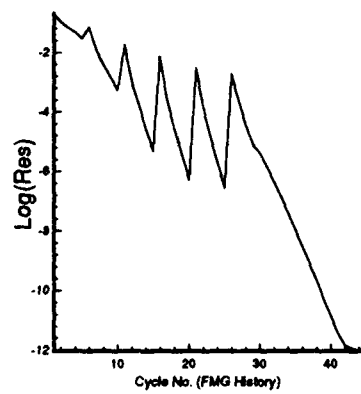
Figure 5: Residuals History
