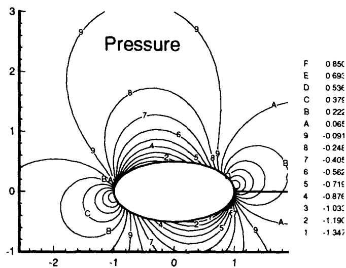
Figure 4: M_\infty = .1 , \alpha = 10 , 128 \times 64 , grid
