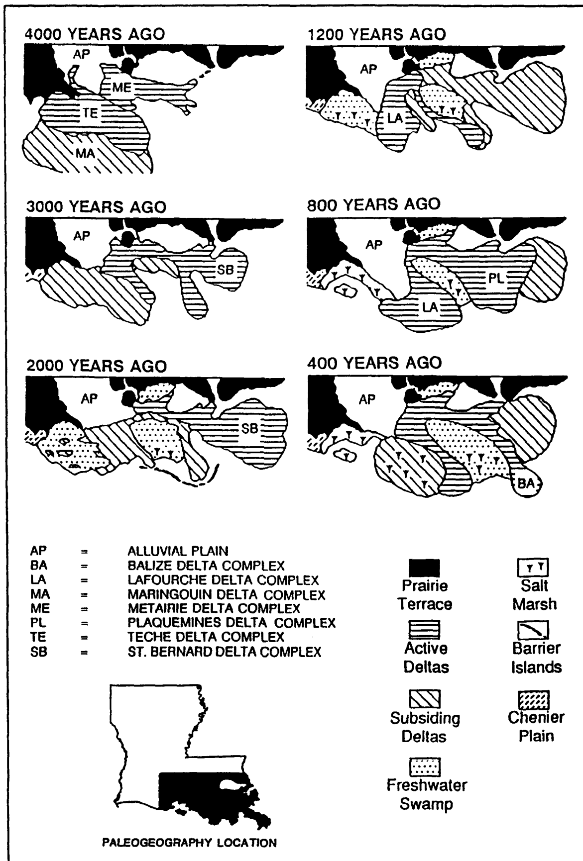
Figure 6. Paleogeography of the Mississippi River Delta (adapted and redrawn from Kusters 1987).
