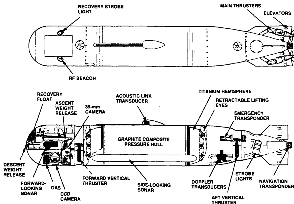
Figure 2. AUSS vehicle.
