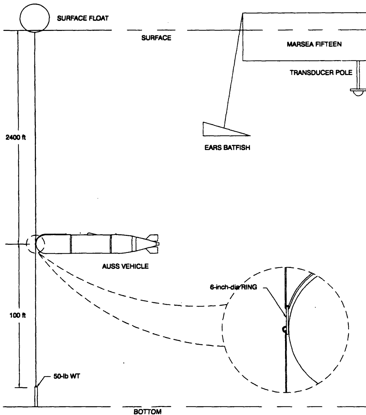
Figure C-2. Ocean bottom at 2500-ft configuration.
