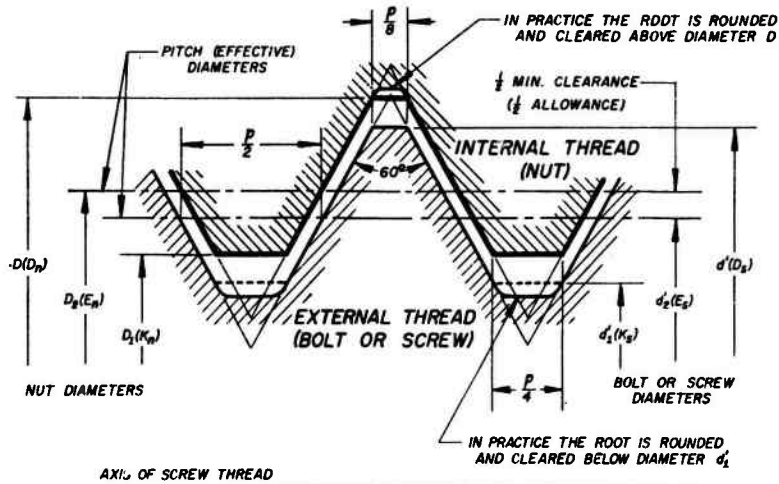
FIGURE 14.2.—ISO design profile of external and internal threads with an allowance for inch and metric screw threads.
