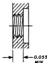
FIGURE XVIII.11.—Open type shutter cable socket with straight (American) thread.
