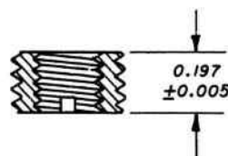
FIGURE XVIII.6.—Adapter; 3/8-16 UNC-1A external thread, 1/4-20 UNC-1B internal thread.
