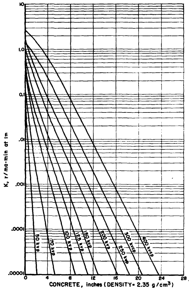
FIGURE 4. Attenuation in concrete of X-rays produced by potentials of 50 to 400 kilovolts
