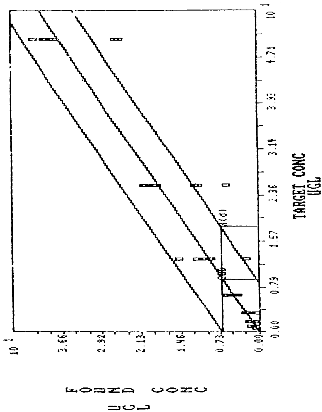
RDX
