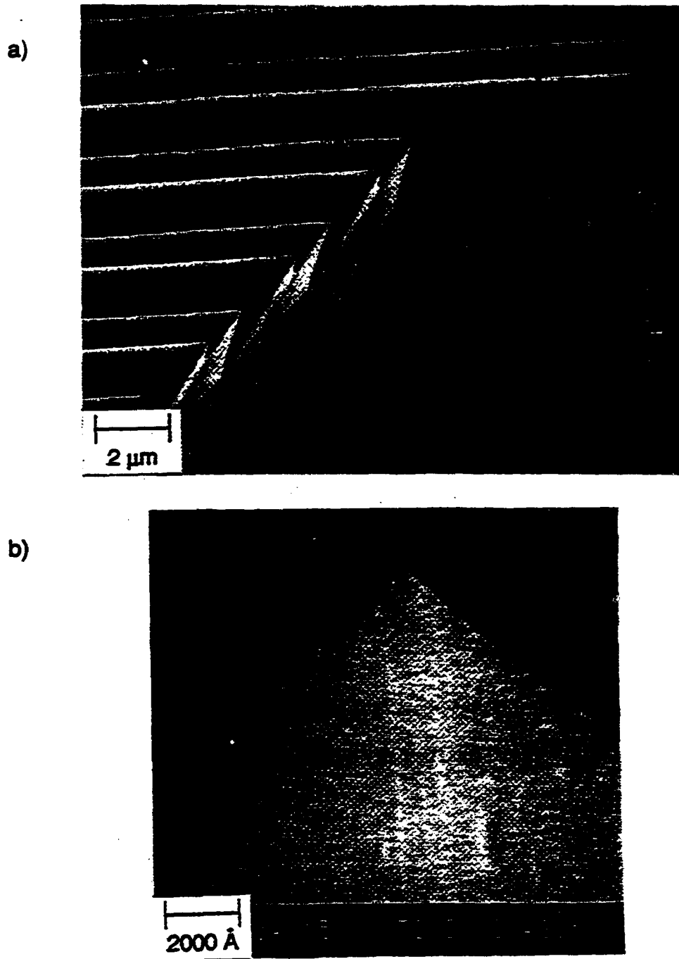
Figure 2.17 a) The truncated blade tips are highly reproducible. b) The radius of curvature of this tip is 170 Å even after being covered with 100 Å of sputtered gold for SEM imaging.
