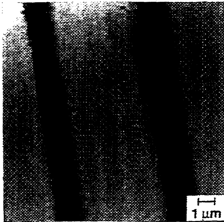
Figure 6.7 A conical tip integrally fabricated with a 200 µm transducer was used to obtain this image of the 6.5 µm silicon grating. The acoustic frequency was 815 MHz.
