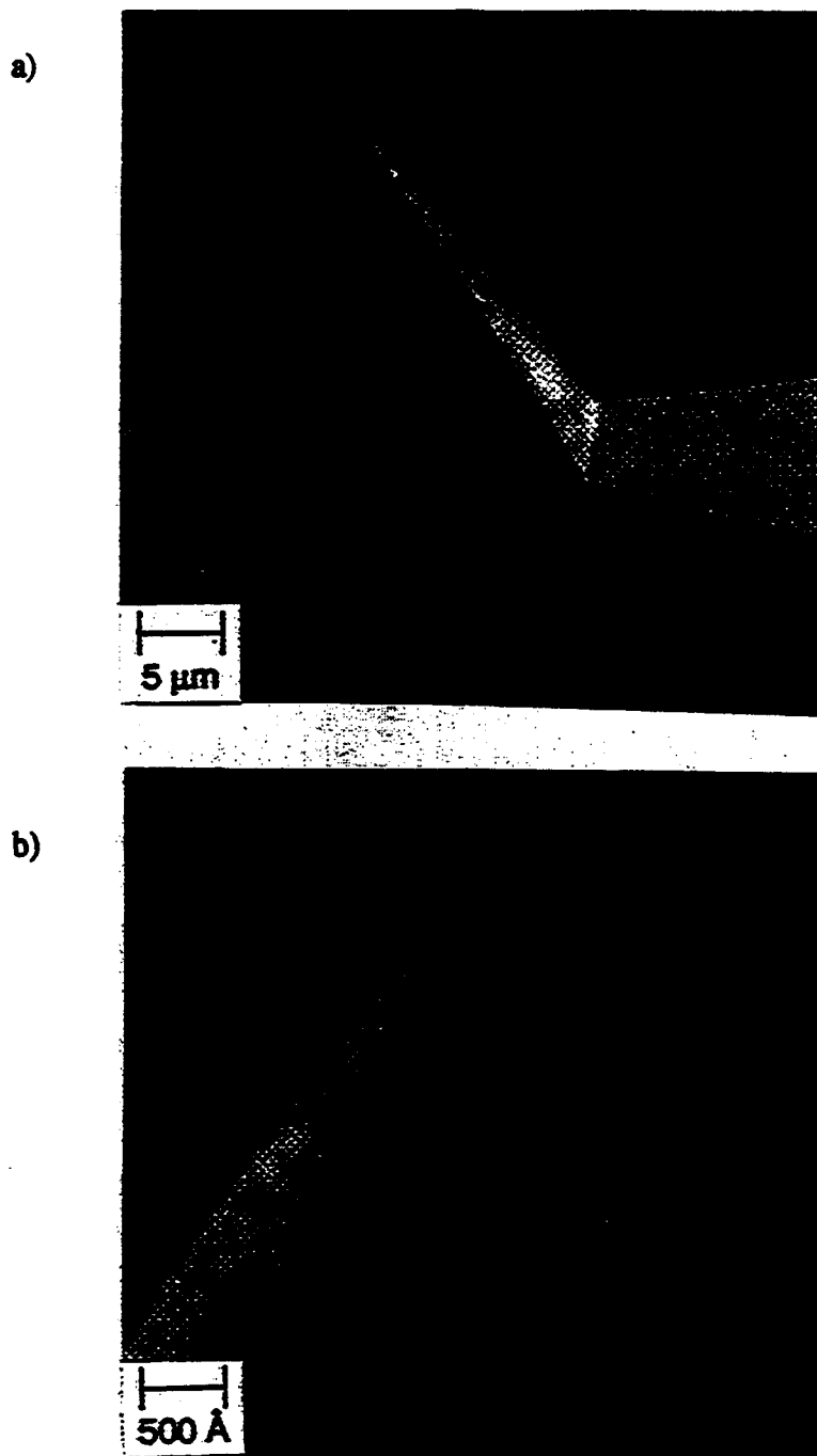
Figure 3.3 a) Since the tetrahedral tip is made of single crystal silicon it can also be oxidation sharpened. b) This photo shows a sharpened tip with less than 100 Å radius of curvature.
