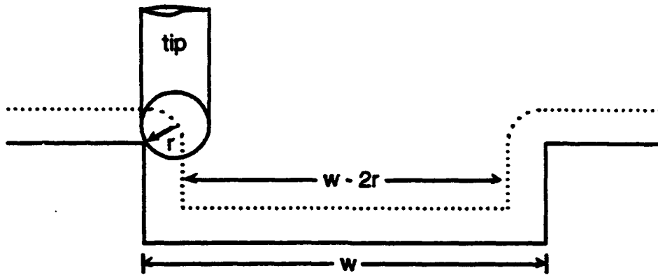
Figure 2.3 When a tip with finite radius is used to image a rough sample, the apparent topography is a convolution of the sample topography and the tip shape.
