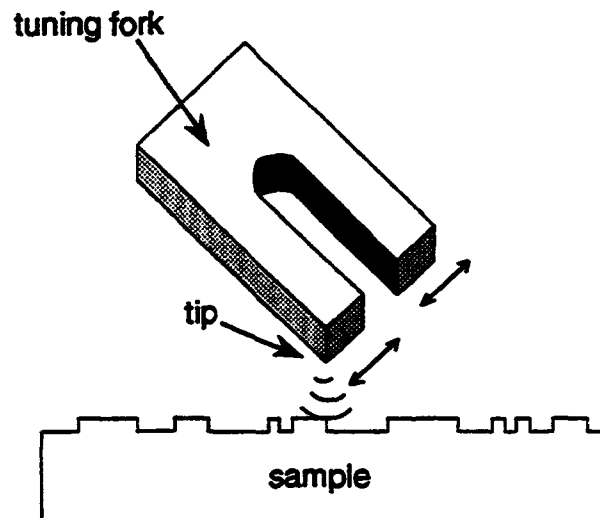
Figure 4.2 G \ddot{u} thner and coworkers use one leg of a quartz oscillator as a tip to probe a sample acoustically. The image is obtained by monitoring the amplitude of the oscillator's vibration.
