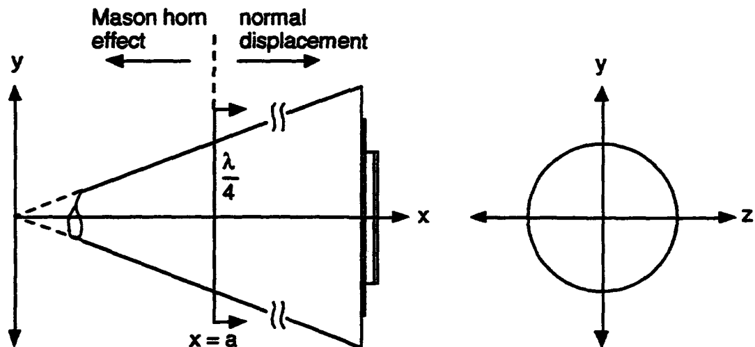
Figure 5.9 The particle motion in the tip is a function of the location of the particle in the tip. The figure above after Graff [3] indicates the axes which will be used in the analysis of the particle motion.
