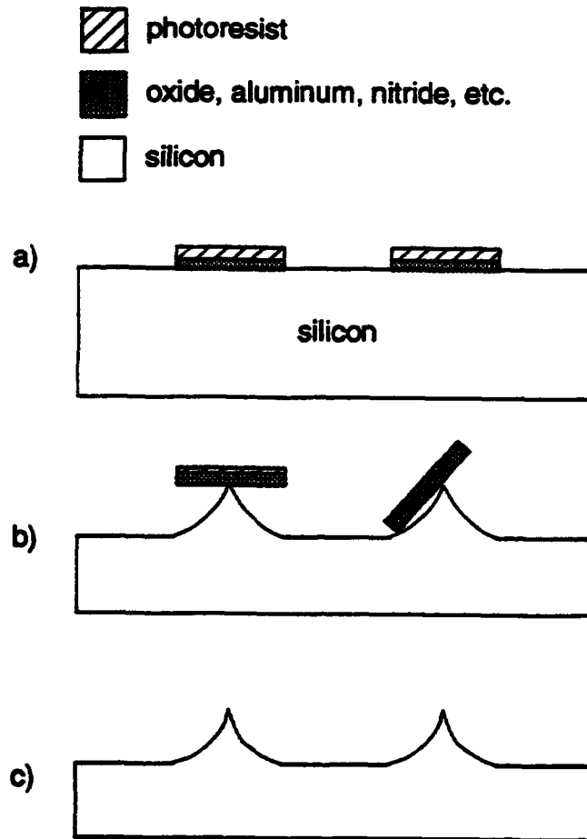
Figure 2.5 To fabricate conical tips a) a masking material such as oxide is patterned into circles. b) Dry or wet etching of the silicon undercuts the masking material and yields conical tips. c) To fully expose the tips, the masking material is selectively removed.
