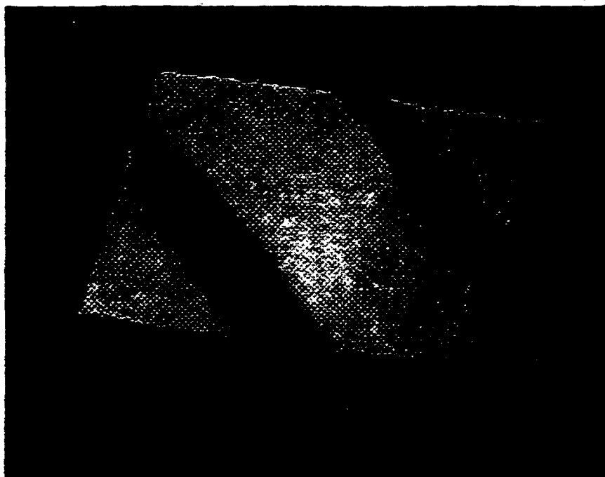
Figure 6.5 The scan direction was rotated to yield this 3-dimensional transmission NSAM image of a 6.5\ \mu\text{m} period silicon grating with 940\ \text{\AA} step height. The image was taken using a tetrahedral tip and an acoustic frequency of 135 MHz.
