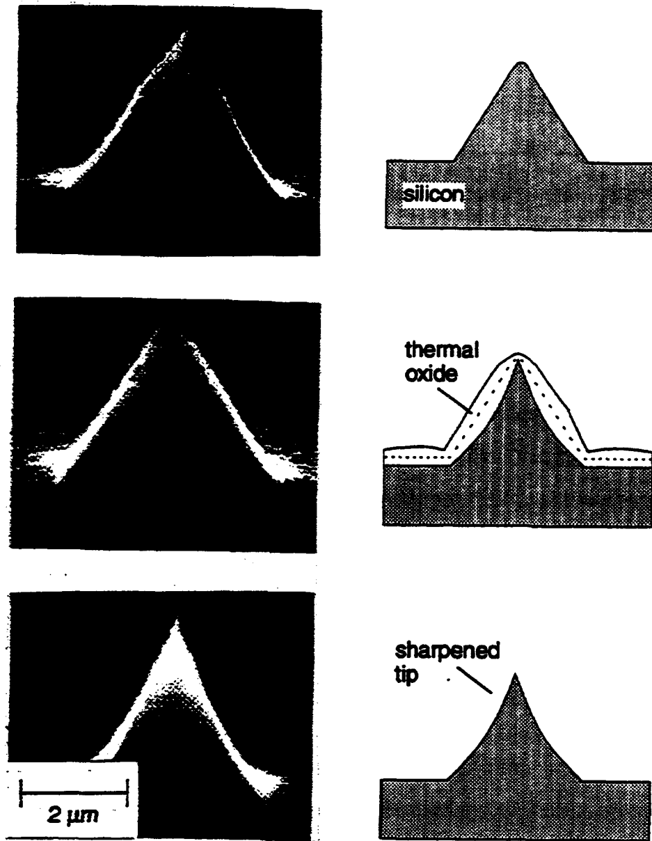
Figure 2.6 a) Conical tips after initial fabrication vary in sharpness across the wafer and have typical radii of curvature of approximately 500\ \text{\AA} . b) When the tip are oxidized at 950\ ^\circ\text{C} to yield several thousands of angstroms of oxide, the oxide growth is non-uniform. c) When the non-uniform oxide is selectively removed, the resulting silicon tips can have radii of curvature less than 100\ \text{\AA} .
