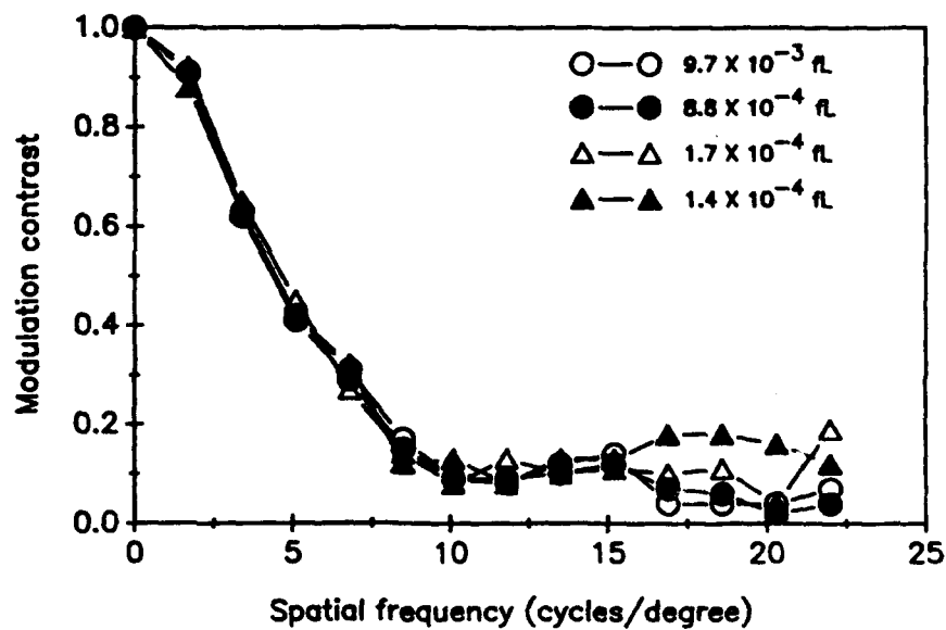
Figure 2. The ANVIS spatial modulation transfer function under varying levels of ambient luminance (Kotulak and Morse, 1994).
