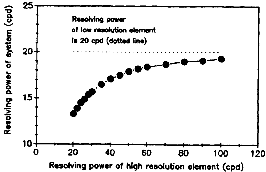
Figure 1. The relationship between the resolving power of the high resolution element and the combined system, given that the resolving power of the low resolution element is held constant. This model was derived from experiments with photographic systems (Farrell and Booth, 1984).
