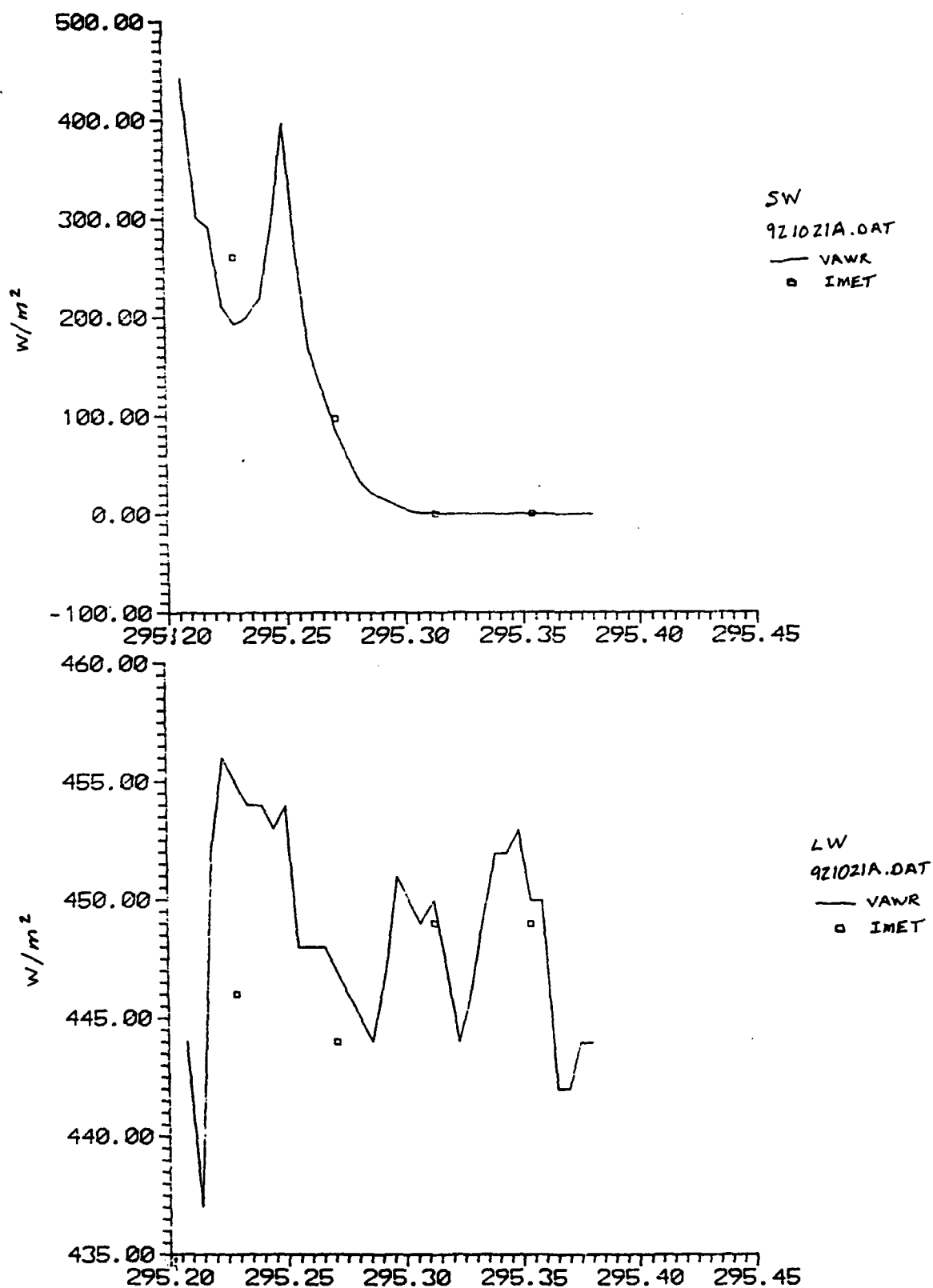
Figure 1-5c,d. VAWR, IMET, ship and GTS sensor comparison shortwave and longwave
