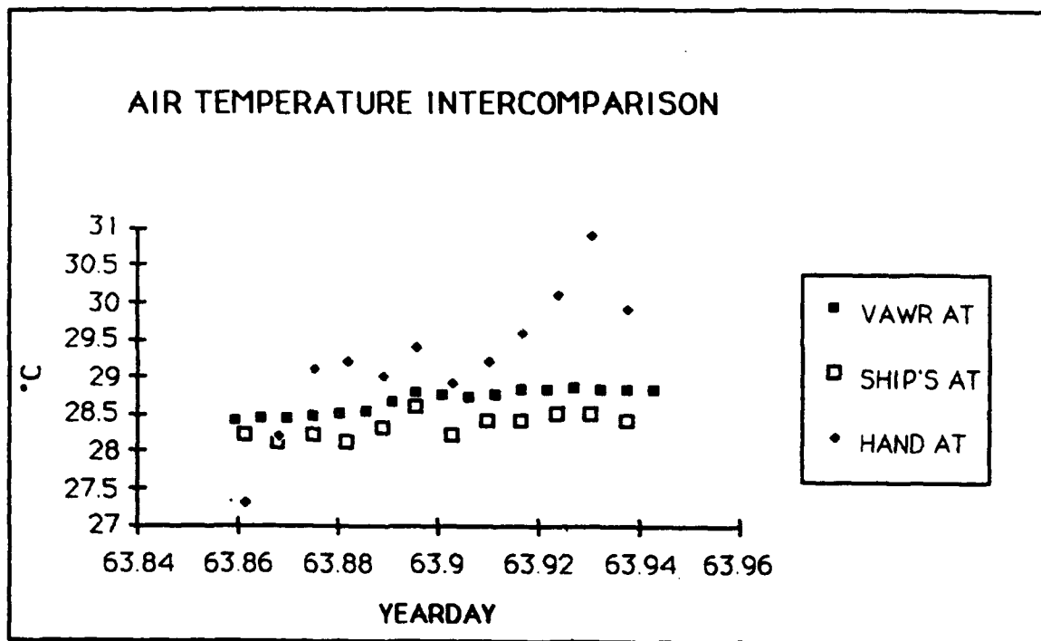
Figure 3-6a, 3-6b. VAWR, Ship and Manual Sensor Comparison Air Temperature and Relative Humidity
