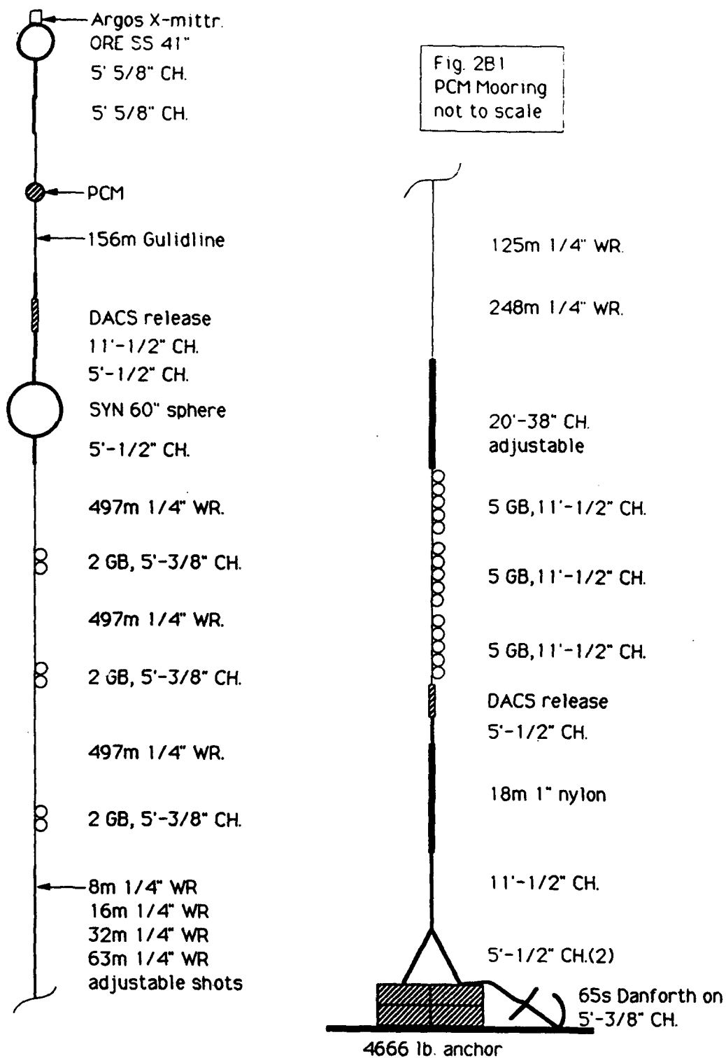
Figure 3-4. PCM Schematic
