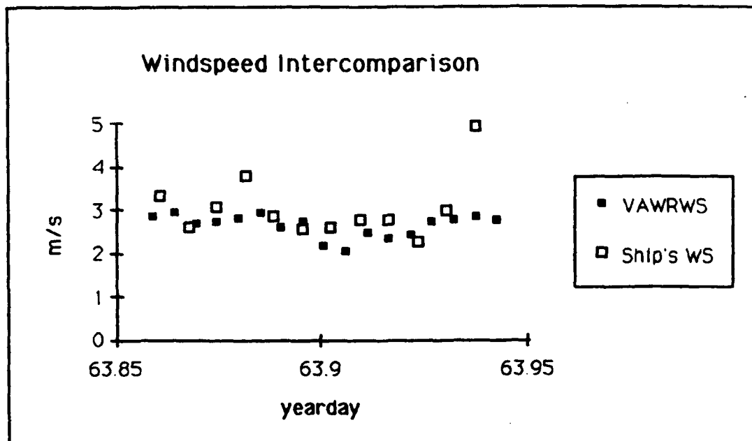
Figure 3-6c, 3-6d. VAWR and Ship Sensor Comparison Wind Speed and Wind Direction
