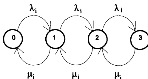
Figure 2.4 - Event Synchronous State Diagram M/M/1/3.
