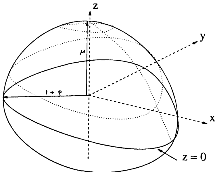
Figure 4. Sketch of a typical V-state
