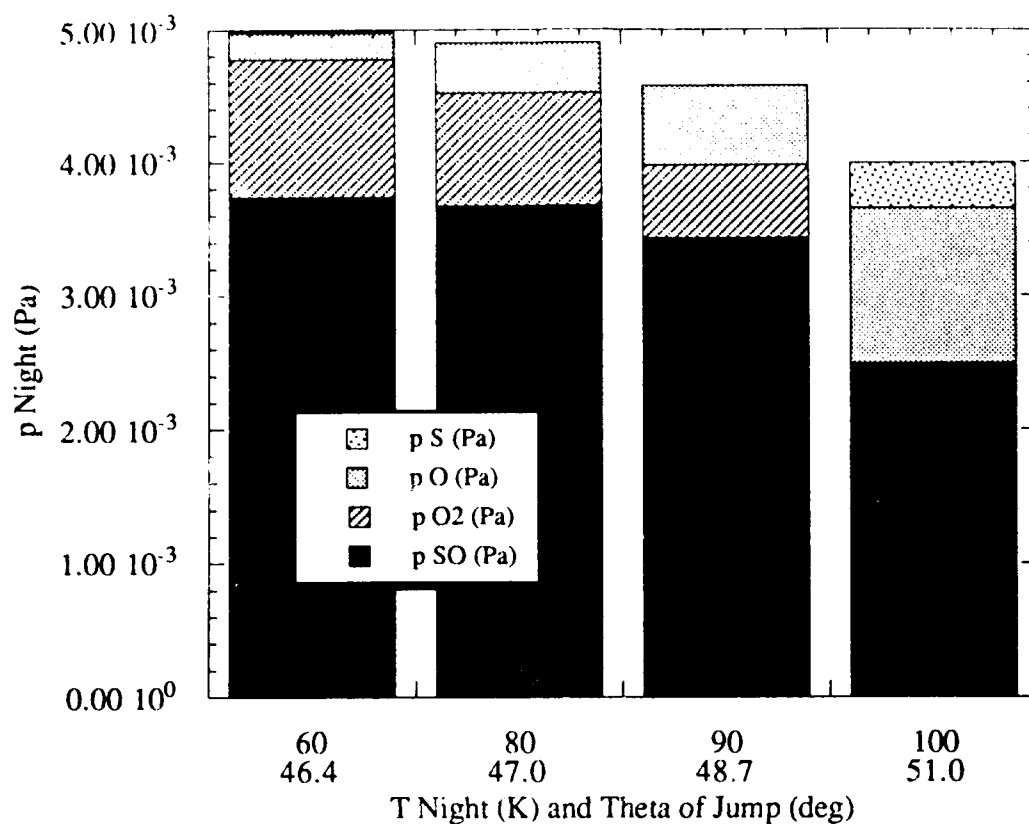
Figure 3.2: Nightside Atmosphere Case 1 ( T_{ss} = 130 K, T_{as} = 50 K)
