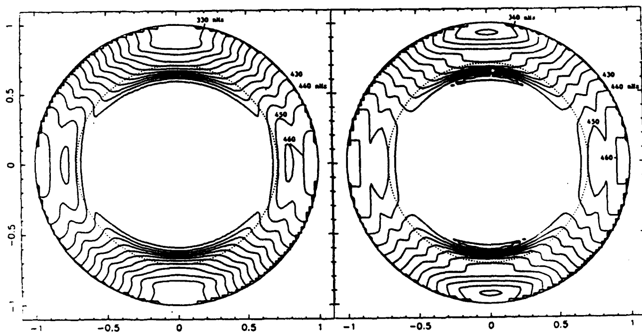
Figure 2: Contour plots showing variations of the solar interior rotation rate from Libbrecht (1988).
