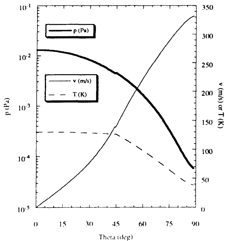
Figure 2.6a: Flow Variables Case 3 ( T_{ss} = 130\text{ K} , T_{as} = 80\text{ K} )
