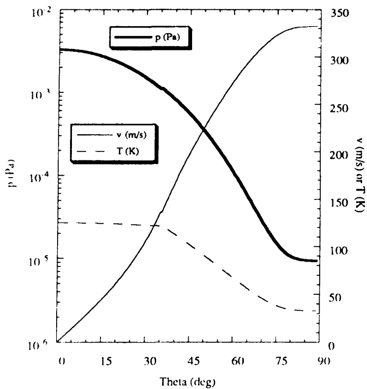
Figure 2.8a: Flow Variables Case 5 ( T_{ss} = 125 K, T_{as} = 50 K)
