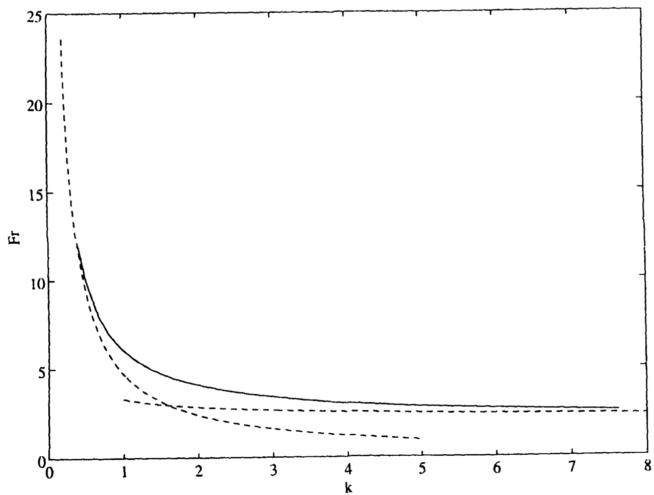
Fig.7 Neutral curve for case II. Solid line indicates the numerical results. Dash line represents the asymptotic behaviours by (49) and (50).
