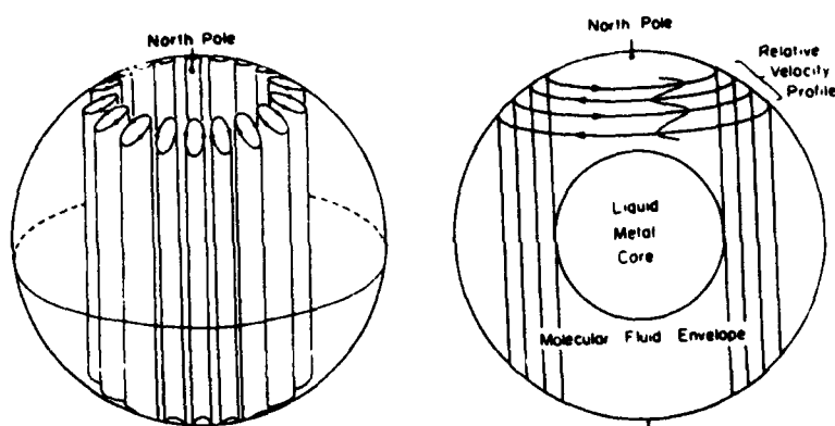
Figure 1: Columnar convection cells (left) and cylindrical zonal flow (right) from Ingersoll & Pollard (1982). Busse (1976) found that the columnar mode is the preferred form of convection in a uniformly rotating, viscous, conducting fluid. The cylindrical mode is the most general form of steady zonal motion in an inviscid, adiabatic fluid.
