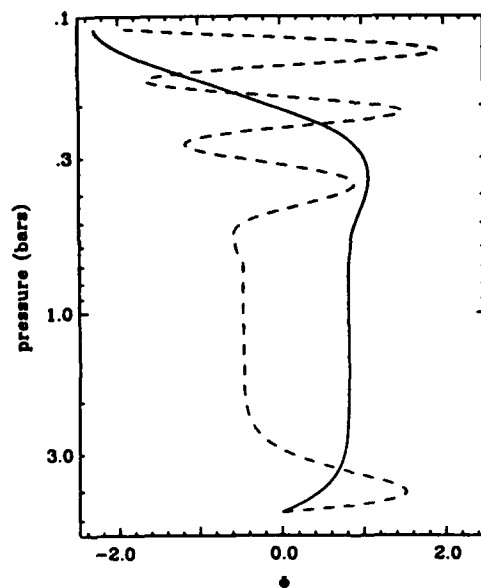
FIG. 4. Vertical structure \Phi , for the first two peaks in the response function in the standard model, shown at the phase when \partial\Phi_i/\partial z|_{z=z_1} is a maximum. The solid line is for \lambda^{-1} = 735 km. The dashed line is for \lambda^{-1} = 155 km.
