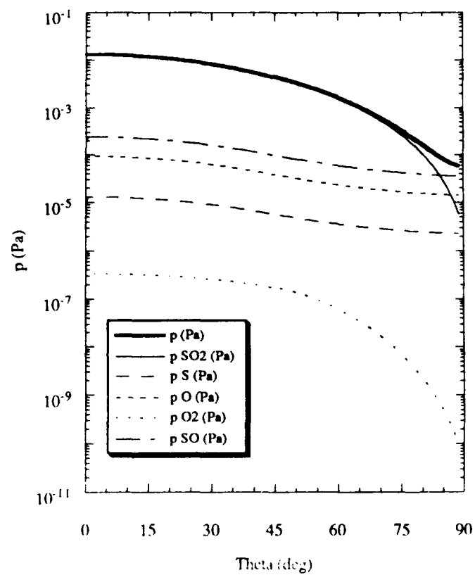
Figure 2.6b: Partial Pressures, Case 3
