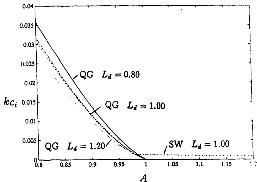
Figure 11: Plot of the quasi-geostrophic and shallow-water growth rates kc_i vs. stability parameter A for different values of L_d . The shallow-water calculations are for a Rossby number \epsilon = -0.20 . It is seen that for all values of L_d the point A = 1 defines neutral stability in the quasi-geostrophic limit and thus violation of Arnol'd's 2nd stability theorem is in fact a sufficient condition for instability for the cosine profile. However, in the shallow-water case the flow is only weakly unstable when A > 1 .
