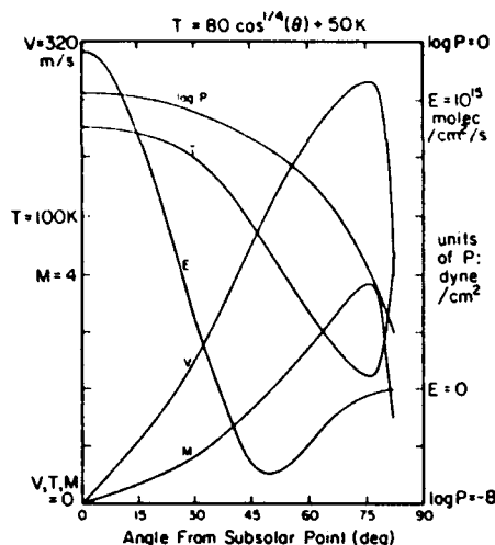
FIG. 2. Solution with subsolar temperature of 130^{\circ}\text{K} . For other parameters, see Table I. The velocity, temperature, and pressure at the top of the boundary layer are V , T , and P , respectively. The Mach number and evaporation rate are M and E . The scales are indicated along the ordinate. Thus, the units of V , T , M , and E are 40 m/sec, 20^{\circ}\text{K} , 1 and 0.2 \times 10^{15} molecules/cm 2 /sec, respectively. The logarithm of P is to the base 10, so that \log P = -8 is a pressure of 10^{-8} dyn/cm 2 .
