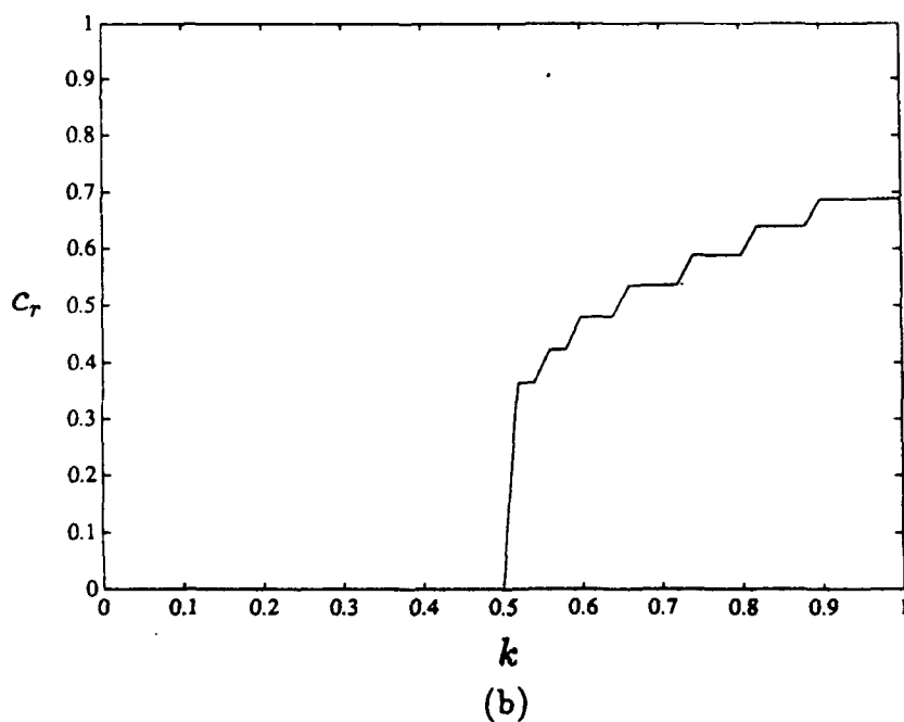
Figure 8: Phase speed c_r against wavenumber k for the shallow-water system with L_d = 1.0 , A = 0.8 and \varepsilon = -0.2 . In (a) the phase speeds of all modes are plotted with the c_r \approx f_0/k behaviour of the gravity waves at small k being evident. (b) Shows the phase speed of the most unstable mode.
