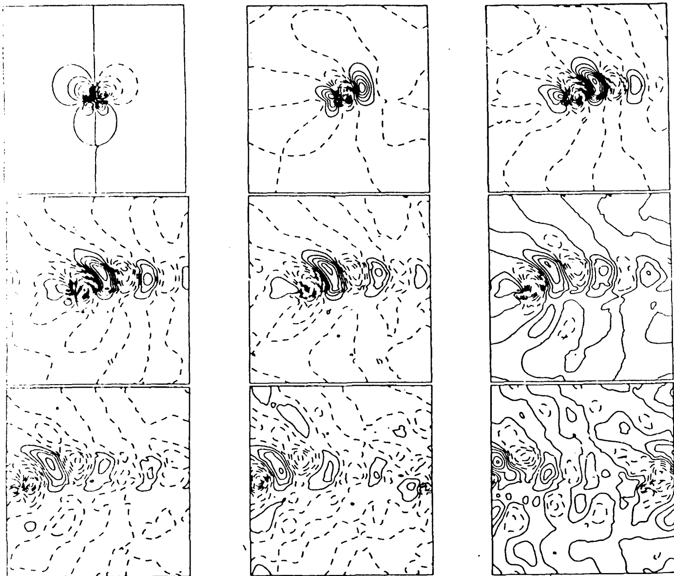
Figure 4b Numerical Simulation, lower layer with finite depth
