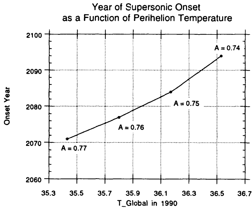
Figure 3. The year of supersonic onset as a function of the temperature at perihelion. The A 's are the Bond albedos corresponding to a given perihelion temperature. This model neglects the thermal inertia of the surface.
