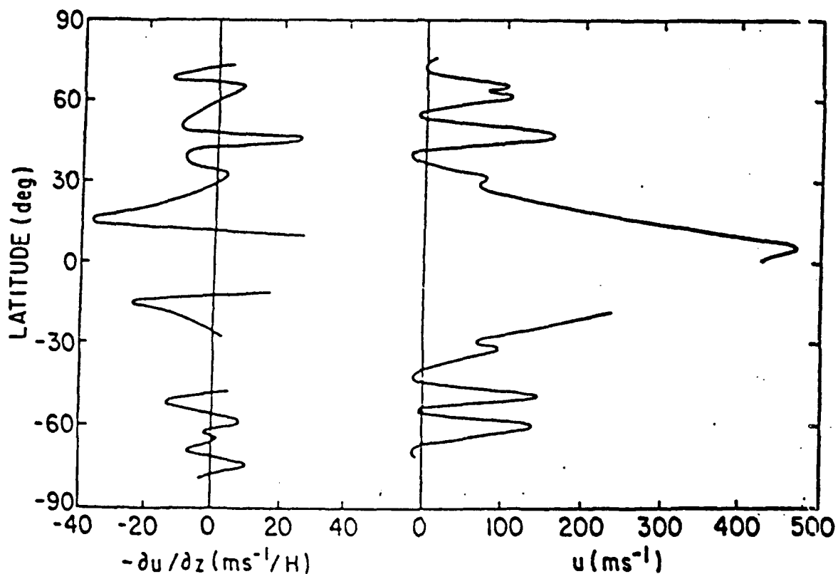
Figures 3, 4 Zonal Wind Shear and Velocity Profiles, Jupiter
