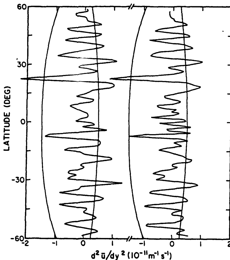
FIG. 4. Curvature or second derivative of Jupiter's zonal velocity profile for the solid curves of Fig. 3. Voyager 1 is on the left and Voyager 2 is on the right. The smooth curve on the right of each profile is \beta , the planetary vorticity gradient for thin spherical shells. The smooth curve to the left of each profile is B \sin^2 \lambda , derived in the text for deep fluid spheres. The B \sin^2 \lambda curve is relevant up to a latitude of about 40 to 45°, where effects of the metallic core become important. The limiting curve (not shown) for deep flow at higher latitudes is infinite at the critical latitude and lies to the right of each profile. Notice that the observed profiles rarely cross the left curve, but often cross the right curve, suggesting that a deep interior flow with the observed curvature might be marginally stable.
