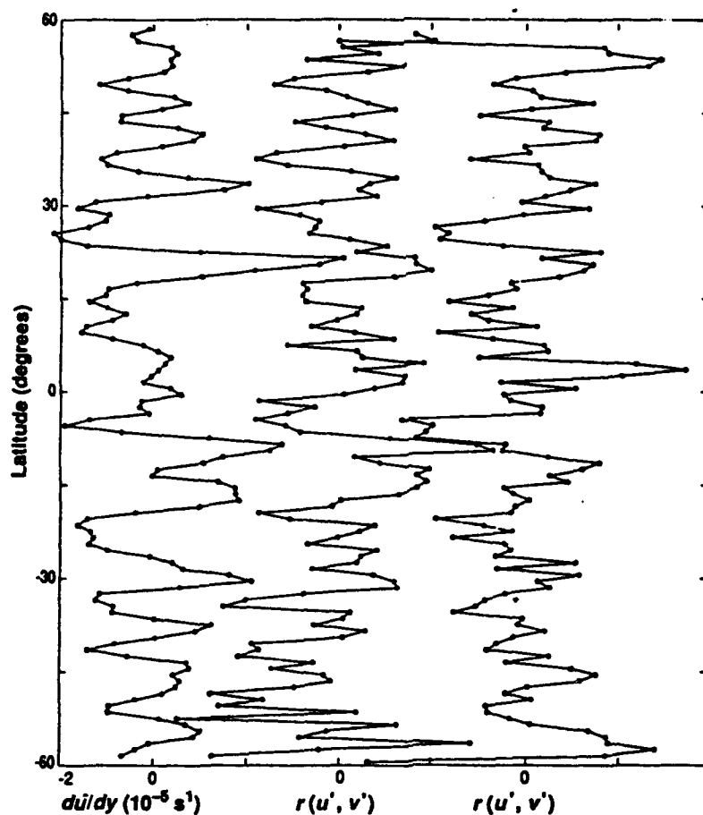
Fig 2.2.1 Comparison of the zonal velocity gradient \bar{u}'\bar{v}' (left) with the eddy correlation coefficient r(u', v') . The center and right curves are from Voyager 1 and Voyager 2, respectively (7). At most latitudes r(u', v') and \bar{u}'\bar{v}' have the same sign, indicating that kinetic energy is being transferred from the eddies to the zonal flow through the Reynolds stress term. [Reprinted from (7) with permission from the American Geophysical Union].
