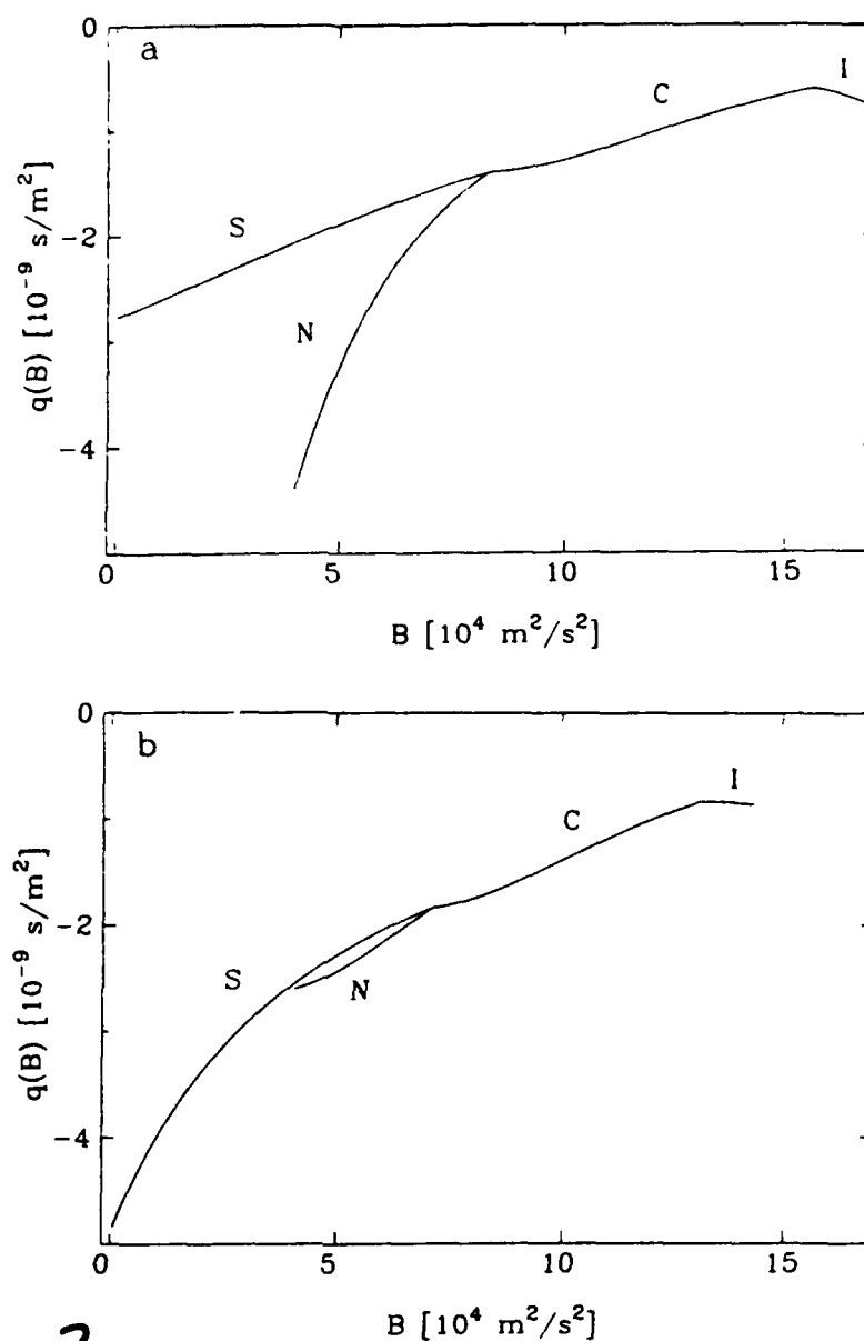
2 Fig. 2. Potential vorticity q versus Bernoulli function B . (a) Model results for the GRS. Different functions q(B) are allowed for the northern and southern open streamline regions, denoted by N and S, respectively. The central closed streamline region is split into two pieces, denoted by C and I. The inner region I is defined by B > 15.6 \times 10^4 \text{ m}^2 \text{ s}^{-2} , the region C is defined by 15.6 \geq B > 8.3 \times 10^4 \text{ m}^2 \text{ s}^{-2} , and the regions N and S are defined by B \leq 8.3 \times 10^4 \text{ m}^2 \text{ s}^{-2} , with latitude greater or less than -23^\circ , respectively. Refer to Fig. 2a for a map of B . The function 1/q(B) is assumed to be piecewise quadratic in each region. The constant term 1/q_0 is specified and equals 1/(-1.40 \times 10^{-9} \text{ s m}^{-2}) in this figure. (b) Same as (a) but for the Oval BC. The region I is defined by B > 13.1 \times 10^4 \text{ m}^2 \text{ s}^{-2} , the region C is defined by 13.1 \geq B > 7.1 \times 10^4 \text{ m}^2 \text{ s}^{-2} , and the regions N and S are defined by B \leq 7.1 \times 10^4 \text{ m}^2 \text{ s}^{-2} , with latitude greater or less than -34.5^\circ , respectively. The specified parameter 1/q_0 equals 1/(-1.84 \times 10^{-9} \text{ s m}^{-2}) .
