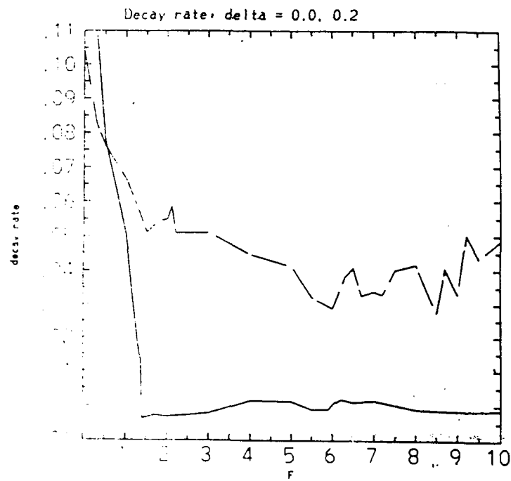
Decay Rate vs. Froude Number
