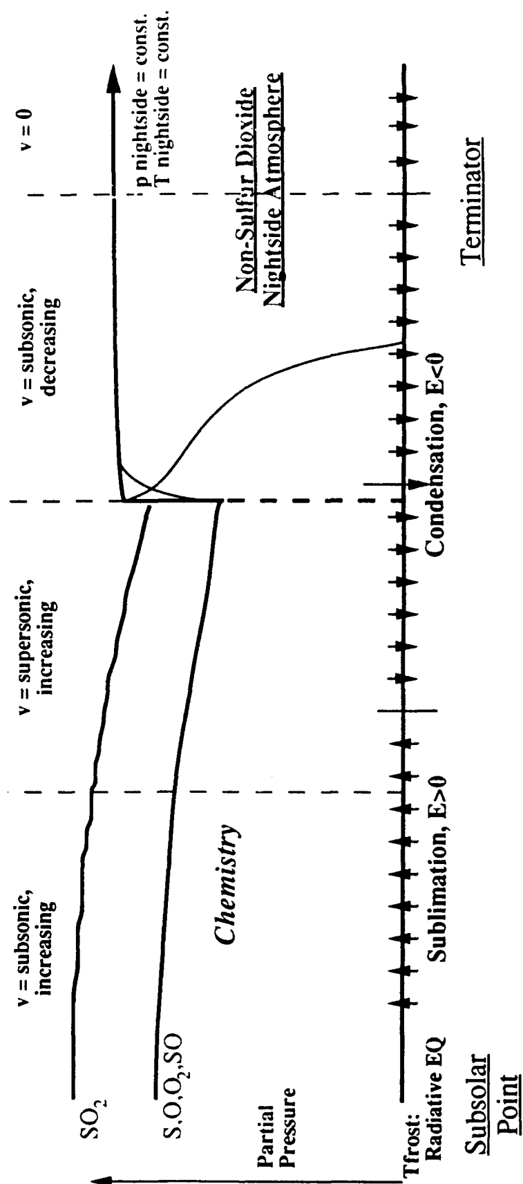
Figure 3.8: First-Order Model, Dayside/Nightside Atmosphere
