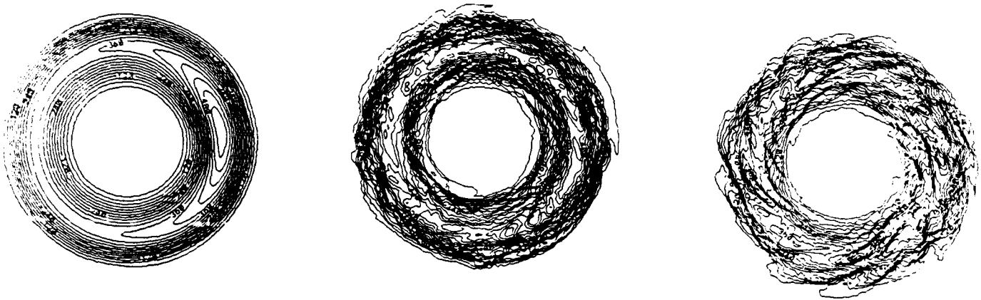
figure 6 weak exponential vortex at r = 1
