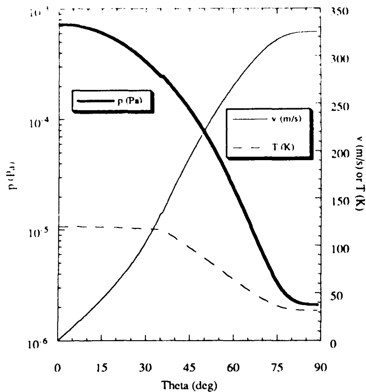
Figure 2.5a: Flow Variables Case 2 ( T_{ss} = 120\text{ K} , T_{as} = 50\text{ K} )
