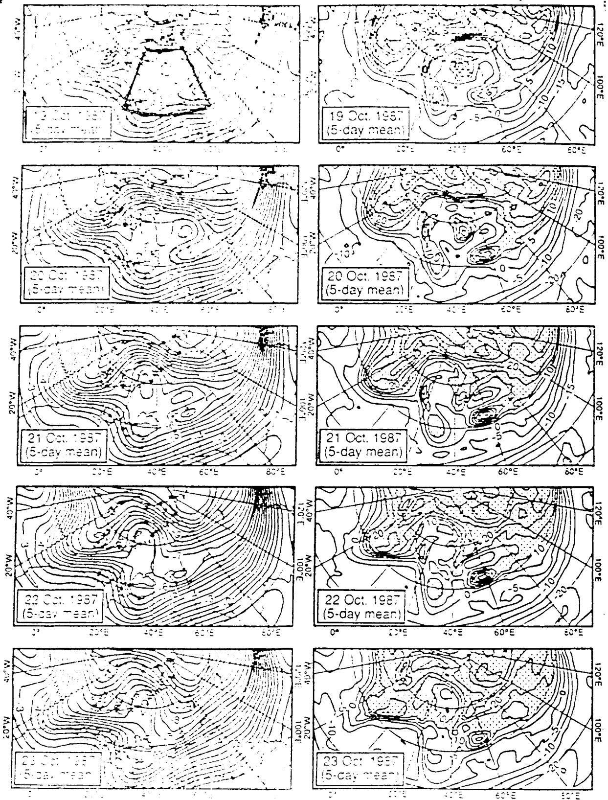
Figure 9 'Blocking High', Stream Function( \psi ) and Potential Vorticity ( q )
