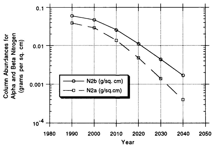
Figure 2. \alpha and \beta N_2 column abundances as a function of time.
