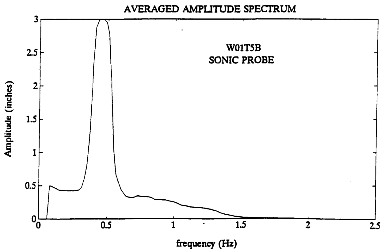
Figure B-9. Wave Averaged Amplitude Spectrum - W01T5A & W01T5B
