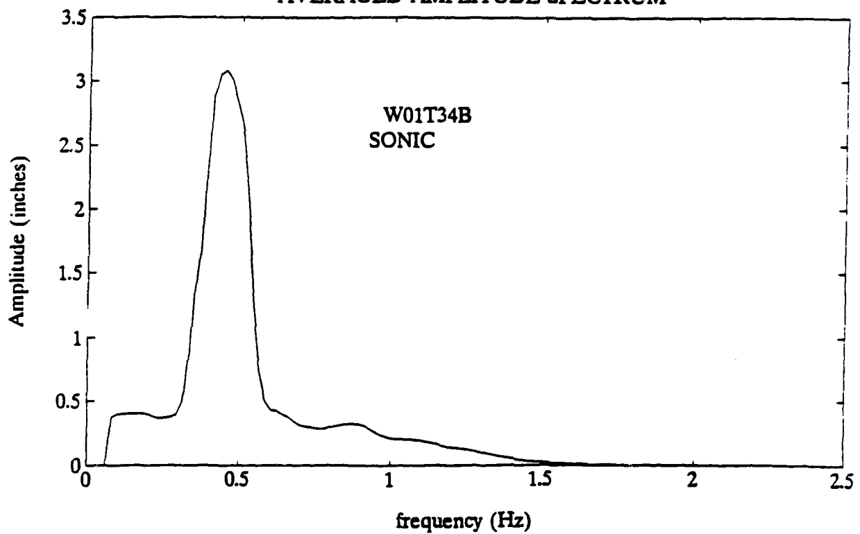
Figure B-16. Wave Averaged Amplitude Spectrum - W01T34A & W01T34B
