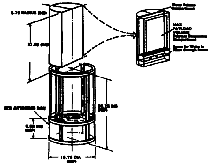
FIGURE 5. Longitudinal Cylinder
