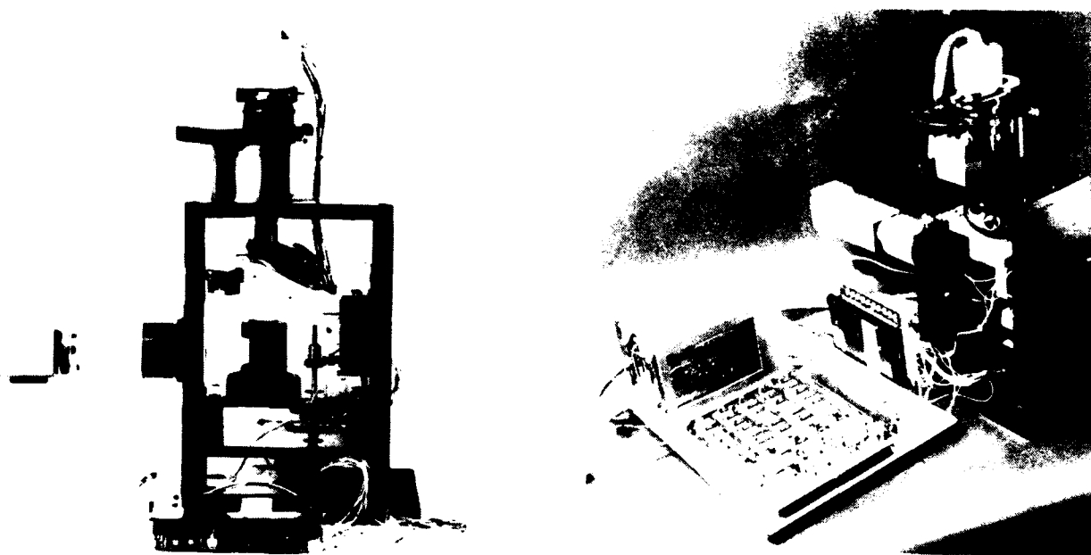
fig.5 Proto-type microscope in microgravity, by which one can observe growth steps with mono-molecular height and automatically measure the growth rate of a crystal
