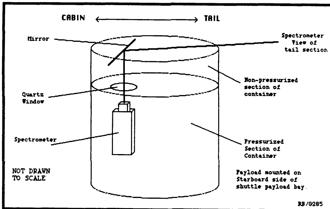
Figure 3. Spectrometer pointing angle
