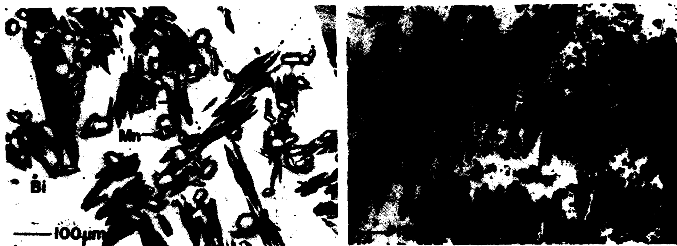
Fig. 3: Micrographs of Mn-Bi samples showing the distribution of Mn, Bi and the compound MnBi. Ground based sample left, flight sample right. MnBi compound is represented with grey color.
