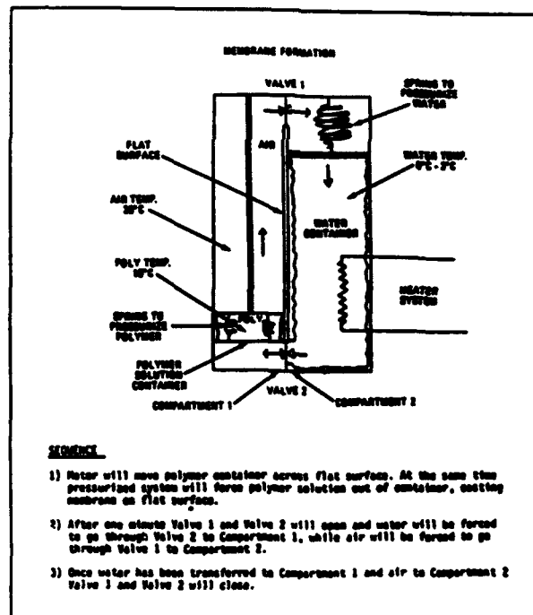
FIGURE 4. Experiment Concept
