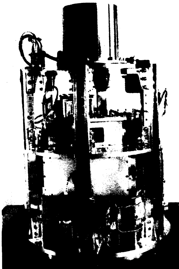
Fig. 1: MAUS standard service system with integrated experiment G-27 on top
