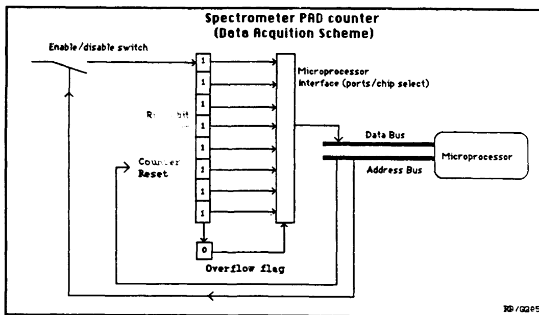
Figure 2. Data acquisition scheme
