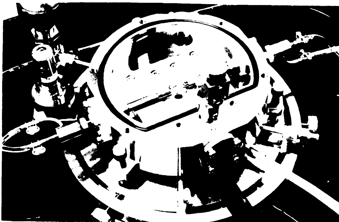
fig.4 Proto-type growth cell at high temperature (1800K) for in situ observation, (a) outside view and (b) the inside, 15cm in diameter
