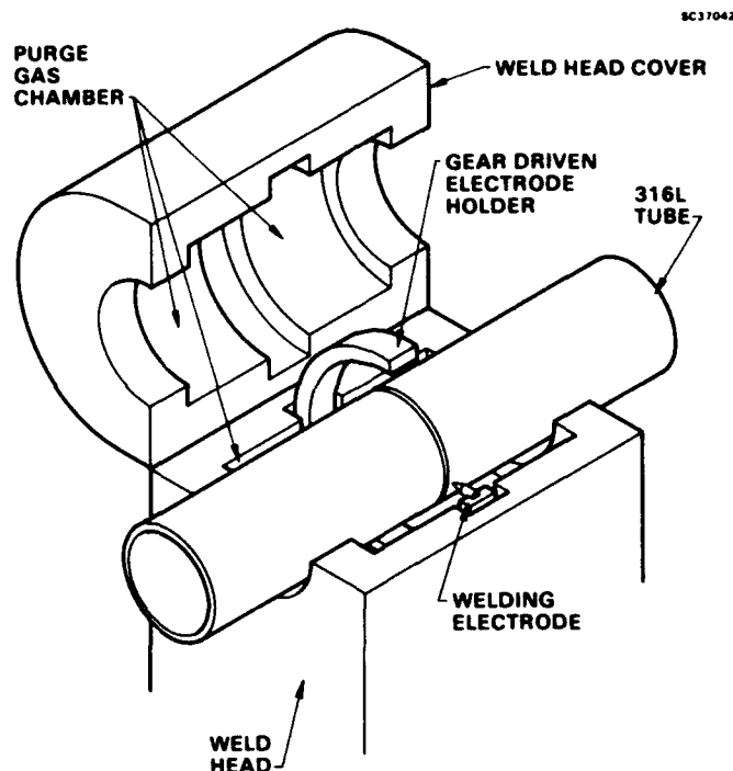
Fig. 2 Schematic diagram of in-place tube weld head.
