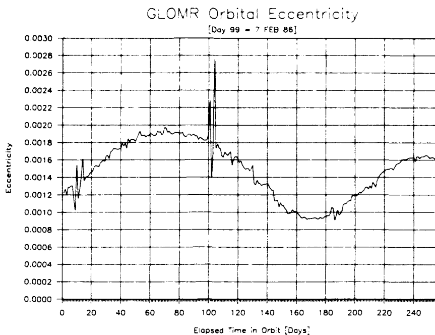
FIGURE 1 LONG TERM BEHAVIOR OF THE GLOMR ORBITAL ECCENTRICITY
