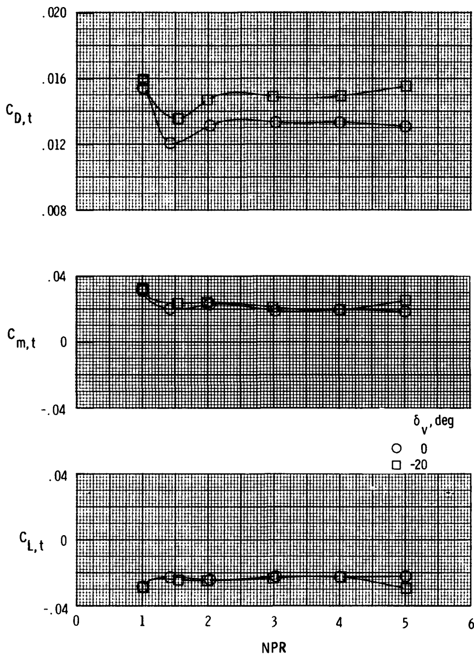
(m) Afterbody-nozzle characteristics with M = 0.90 and \alpha = 0^\circ .
