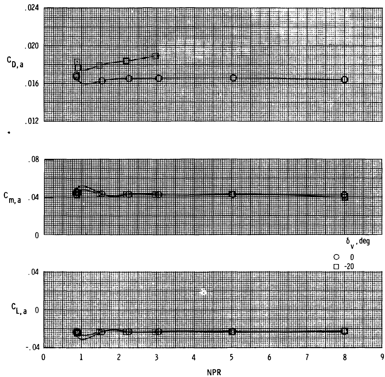
(t) Afterbody characteristics with M = 1.25 and \alpha = 0^\circ .
