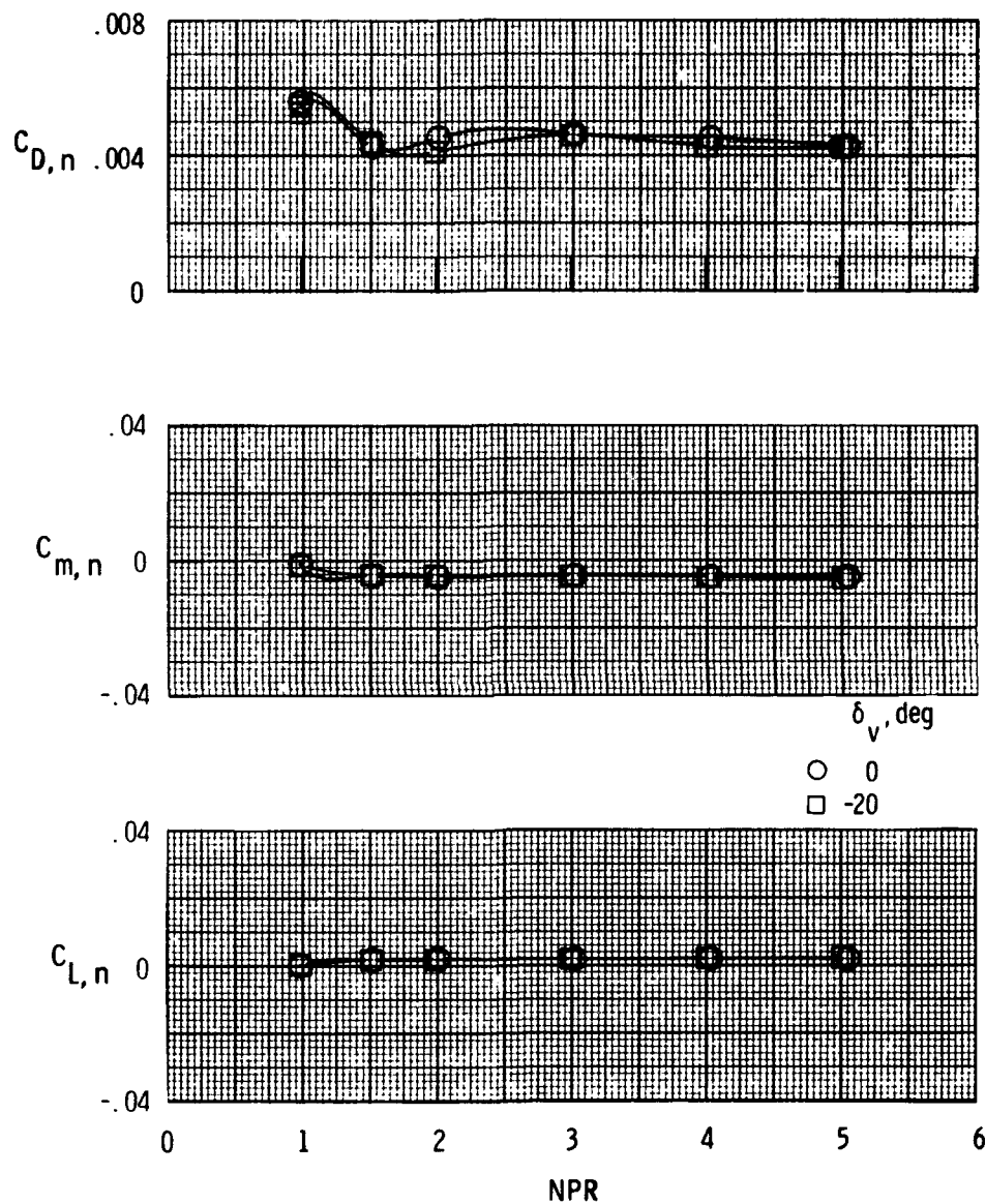
(I) Nozzle characteristics with M = 0.90 and \alpha = 4.3^\circ .
