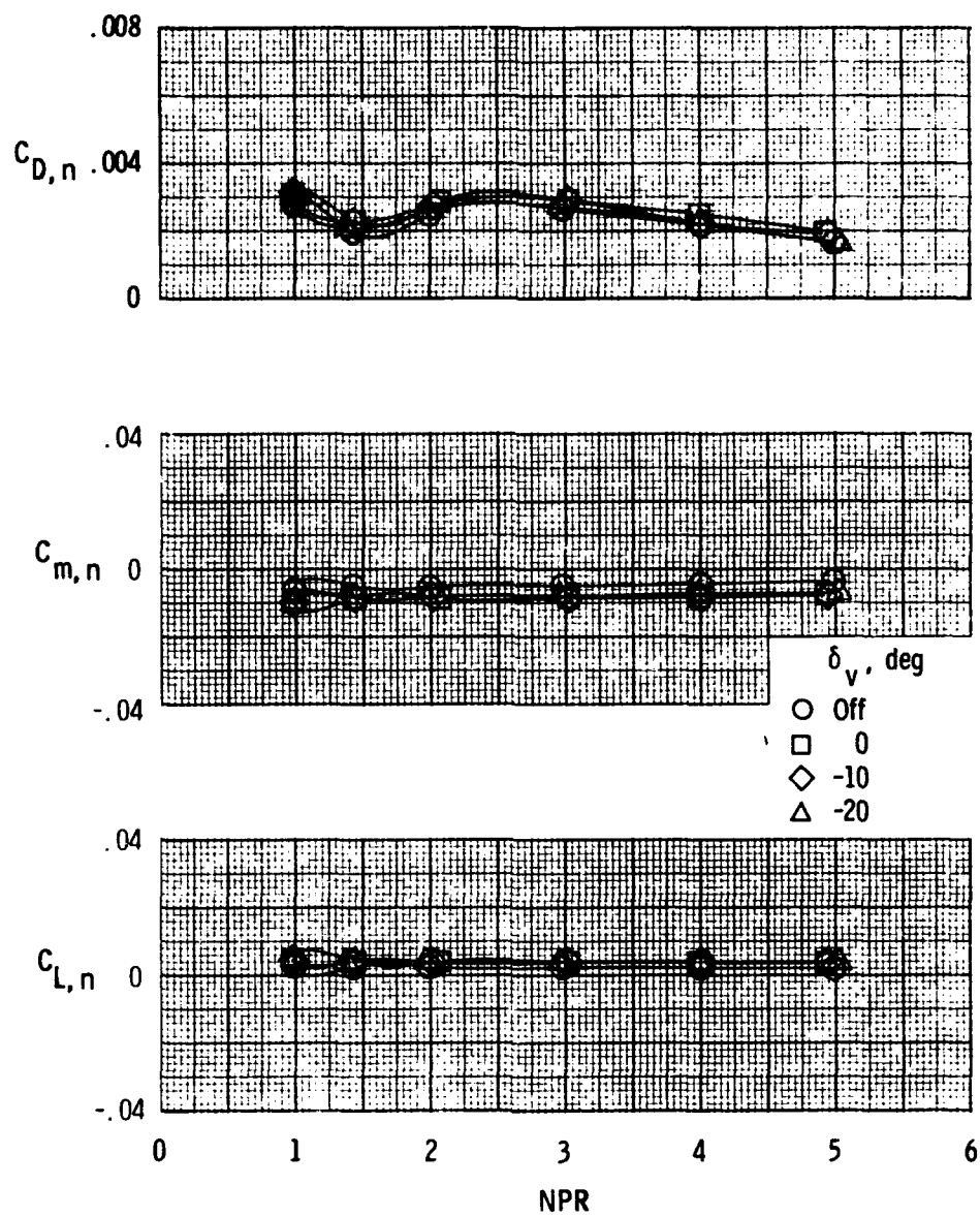
(l) Nozzle characteristics with M = 0.80 and \alpha = 4.3^\circ .
