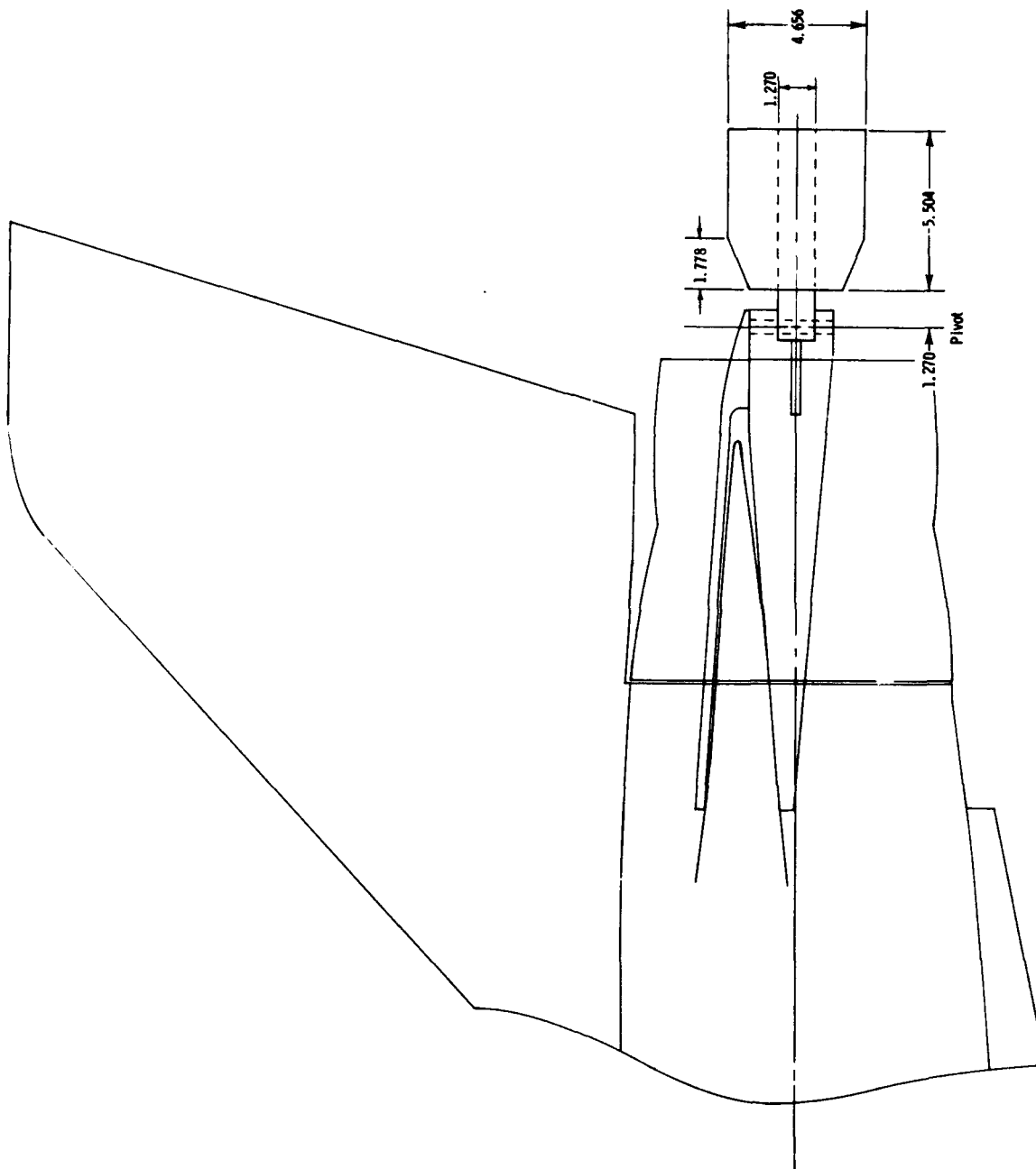
(g) Installation and details of yaw vane.
