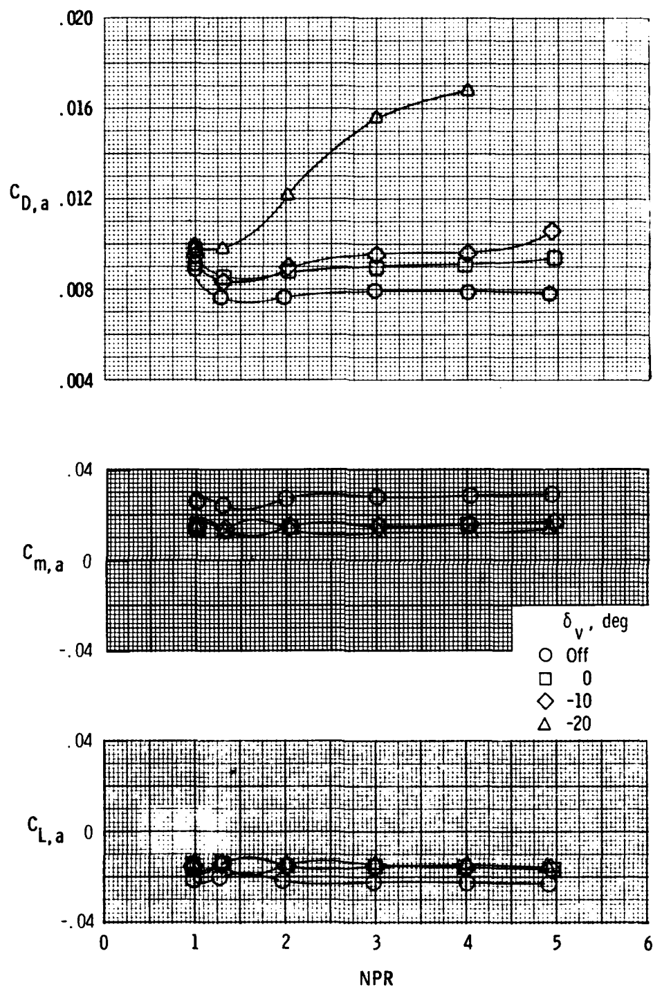
(b) Afterbody characteristics with M = 0.70 and \alpha = 0^\circ .
