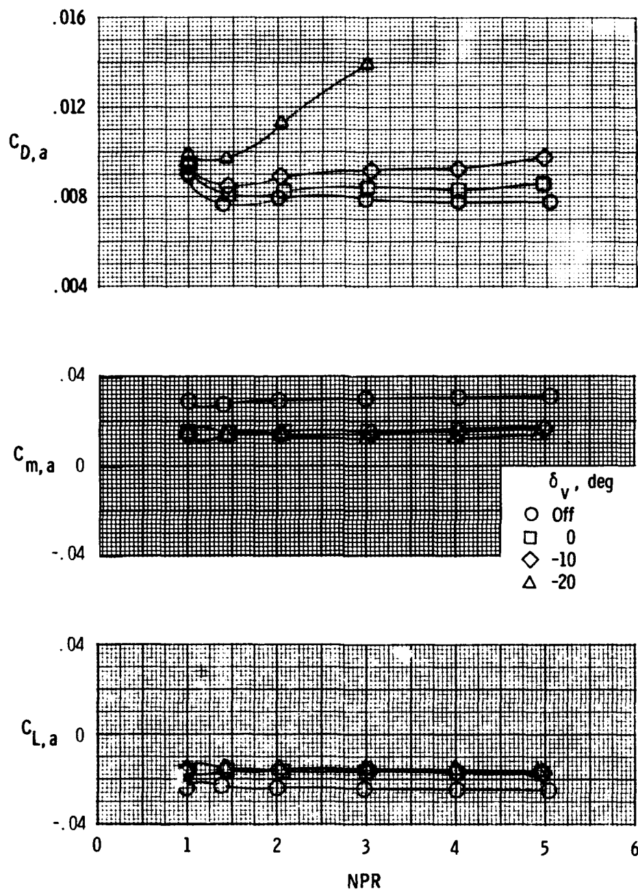
(h) Afterbody characteristics with M = 0.80 and \alpha = 0^\circ .
