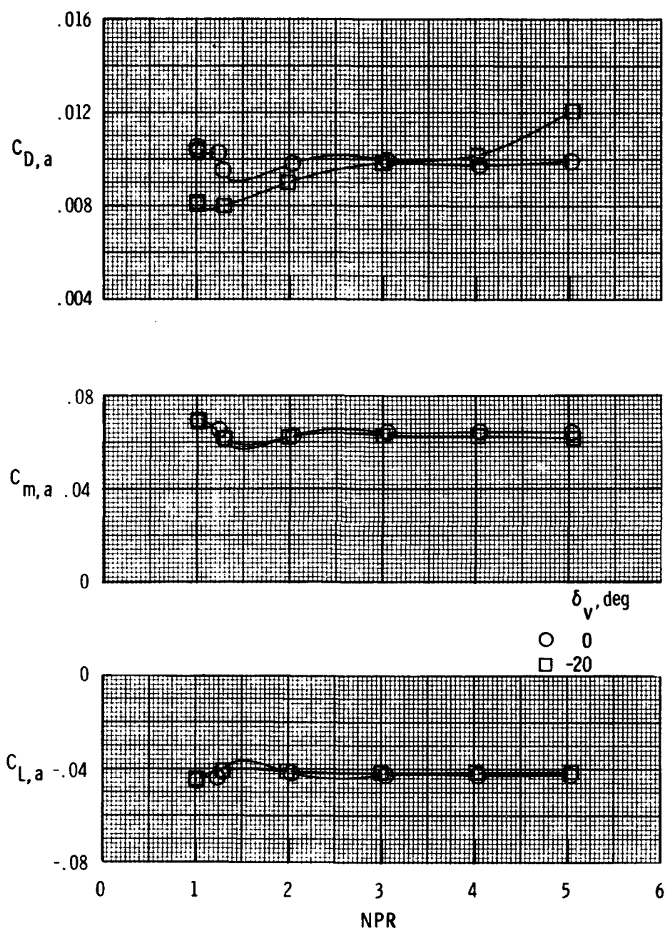
(b) Afterbody characteristics with M = 0.70 and \alpha = 0^\circ .
