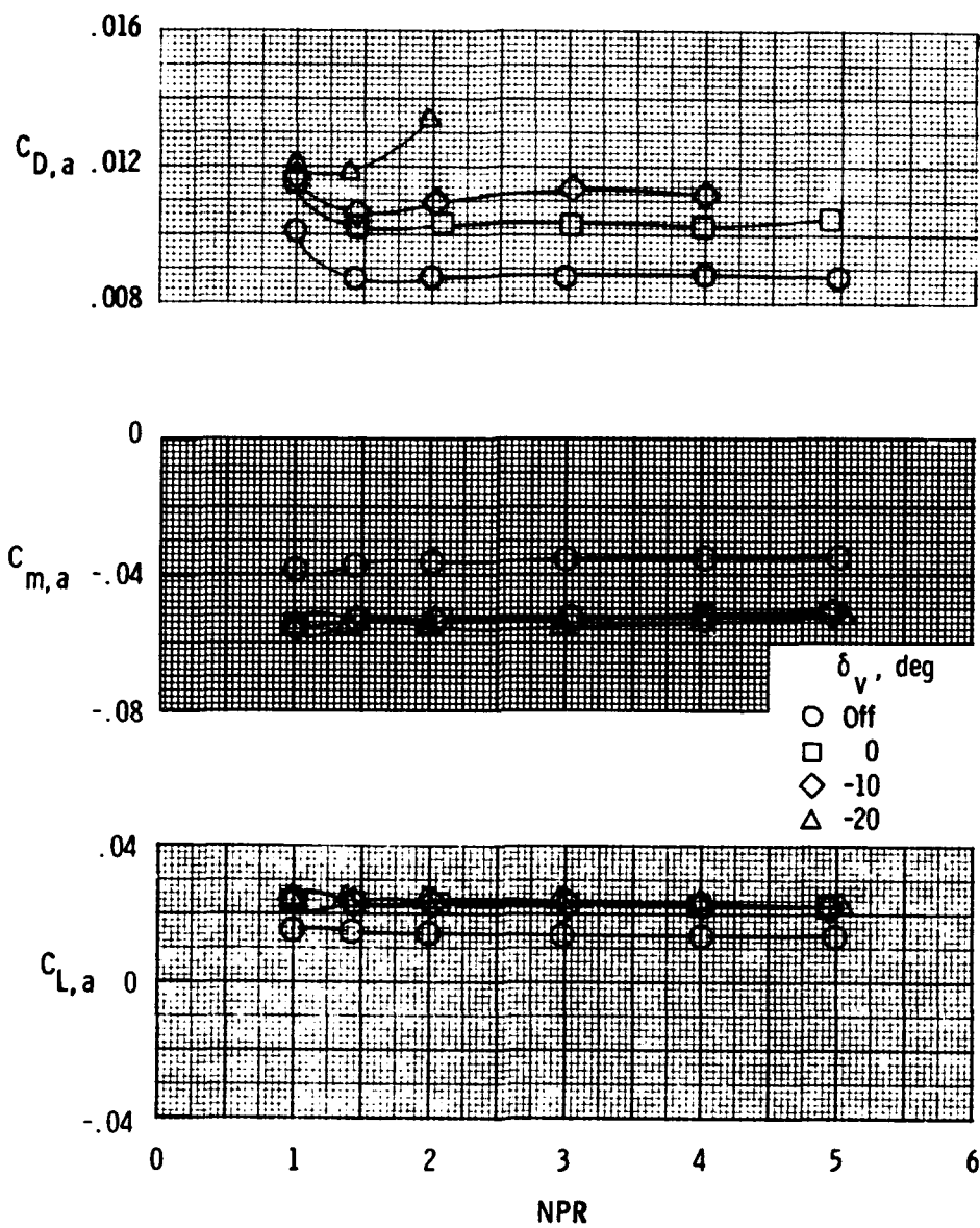
(k) Afterbody characteristics with M = 0.80 and \alpha = 4.3^\circ .
