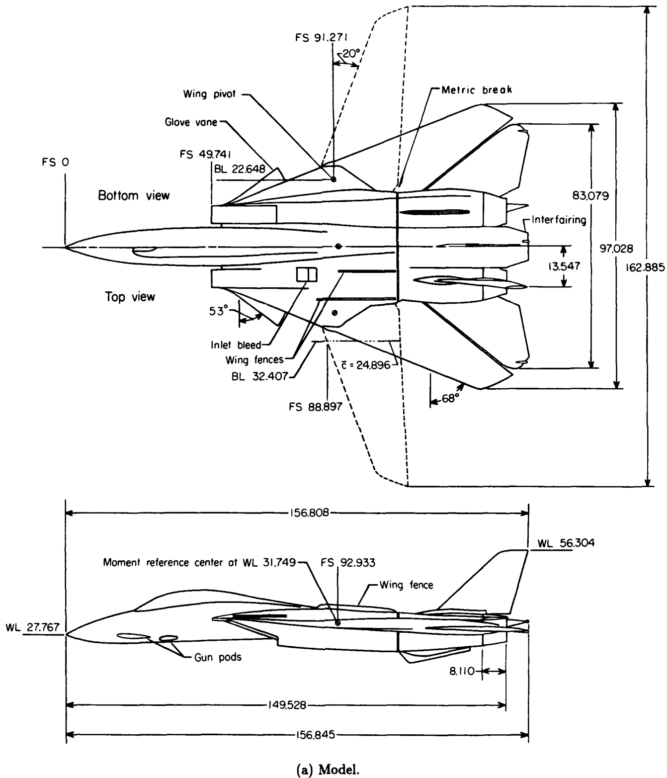
Figure 2. Sketch of model and geometric details of model support. All dimensions are given in centimeters unless otherwise specified.
