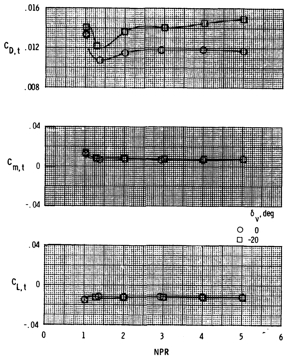
(a) Afterbody-nozzle characteristics with M = 0.70 and \alpha = 0^\circ .
