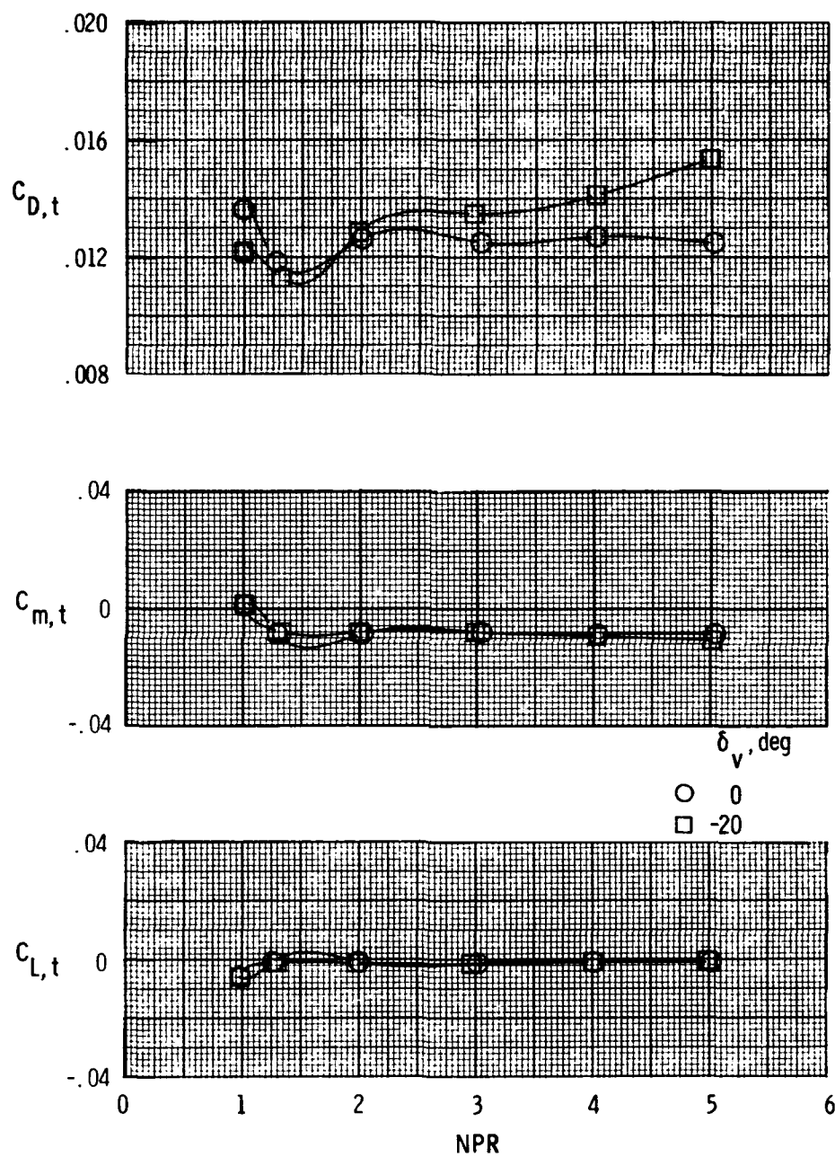
(d) Afterbody-nozzle characteristics with M = 0.70 and \alpha = 4.3^\circ .
