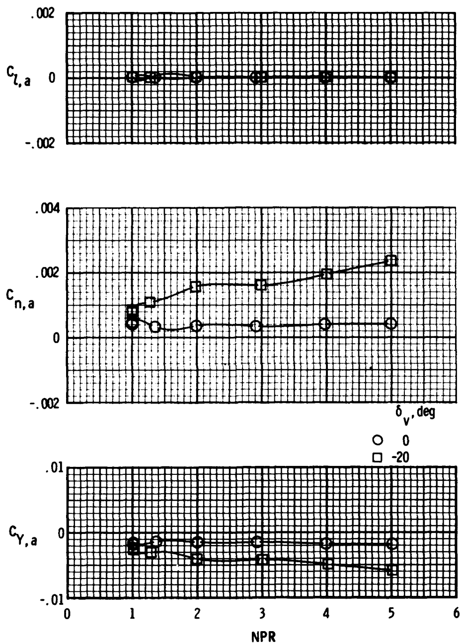
Figure 12. Afterbody lateral-directional characteristics for model with F110 cruise nozzles and yaw vanes installed. \Lambda = 68^\circ ; \delta_h = 0^\circ .
