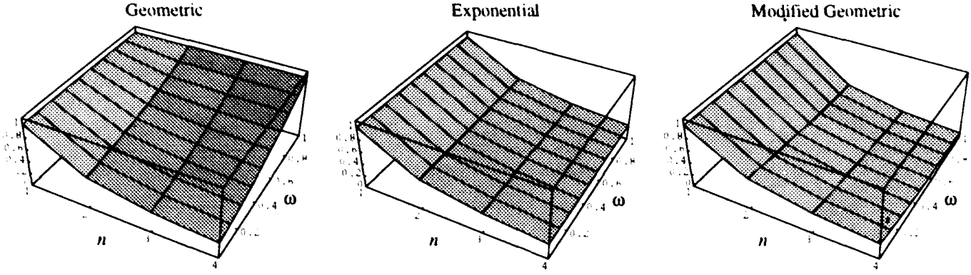
Figure 1: E[X_{(1)}] , E[Y_{(1)}] , and E[Z_{(1)}] ( n = 1, \dots, 5, \forall i, \lambda_i = 1 ) as a function of \omega .
