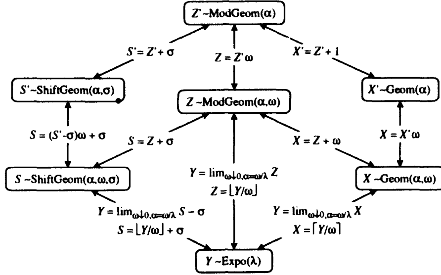
Figure 2: Relationships between the distributions discussed in this paper.
