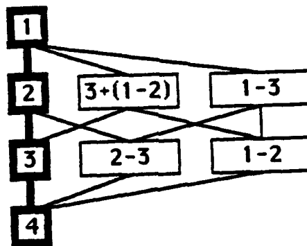
Fig. 4 Extending the MET Browerian Algebra to a Boolean Algebra
