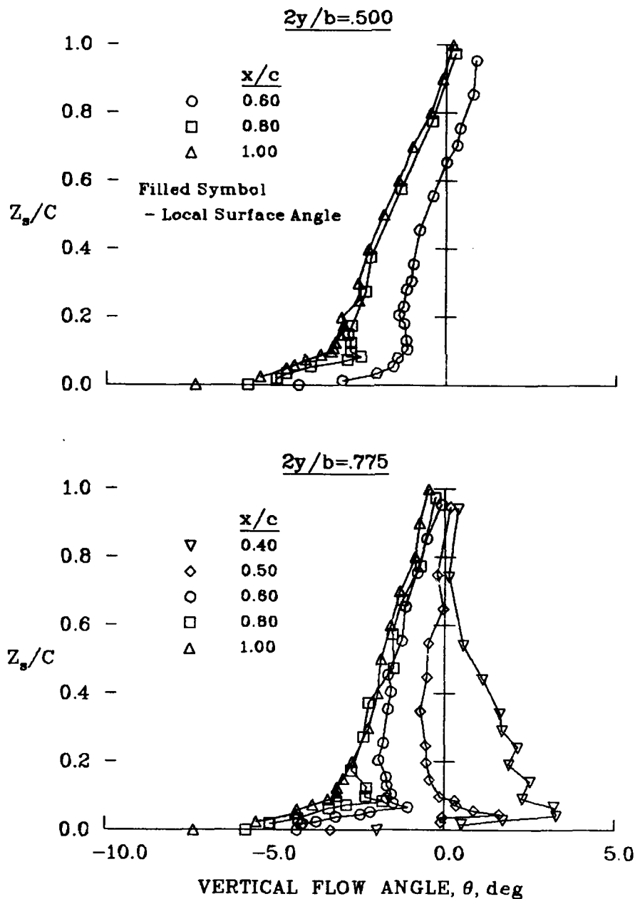
Figure 31.- Flow-field surveys of vertical flow angle; \alpha = 0^\circ , M_\infty = 0.826 , Re_{\infty, c} = 8 \times 10^6 .
