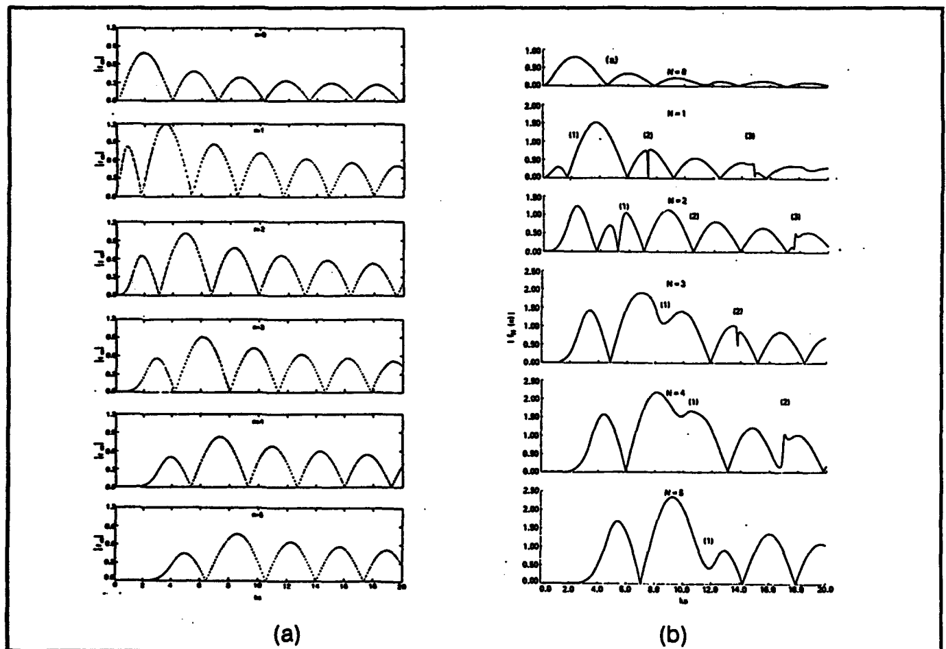
FIGURE 2-2. BACKSCATTERED SPECTRA WITH AND WITHOUT CONSIDERATION OF RESONANCE 46
