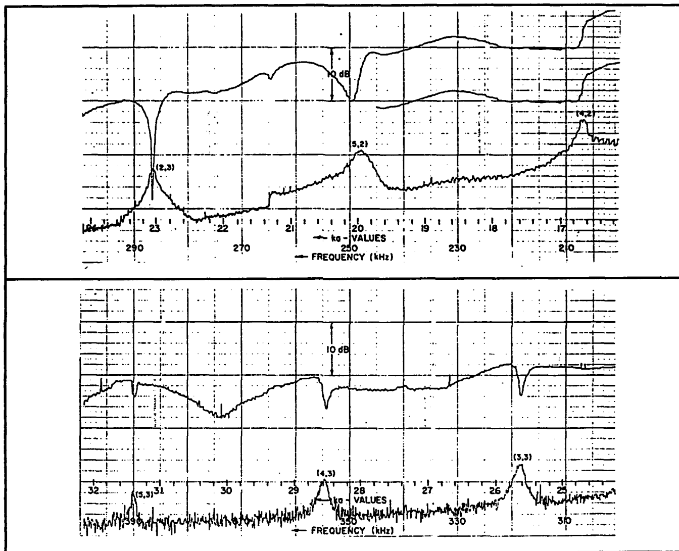
FIGURE 5-12. SPECTROGRAM OF A HORIZONTAL 1.5" DIAMETER HOLLOW CYLINDER
