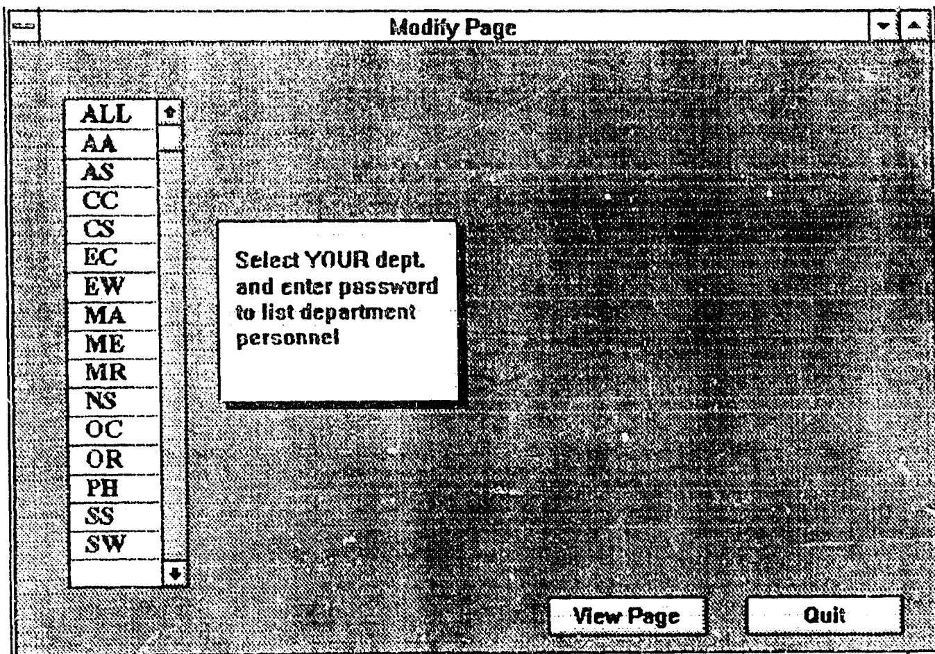
Figure 15 Modify Page
