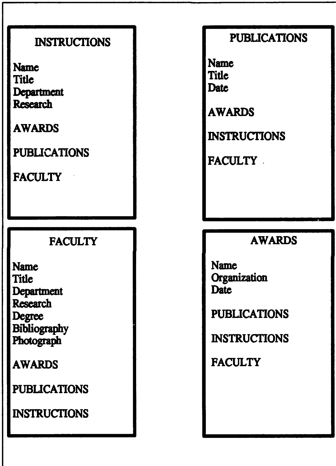
Figure 1 Object Model
