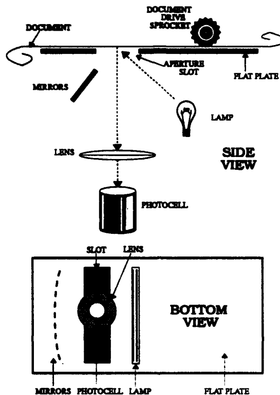
Figure 1.1: Facsimile Scanner
