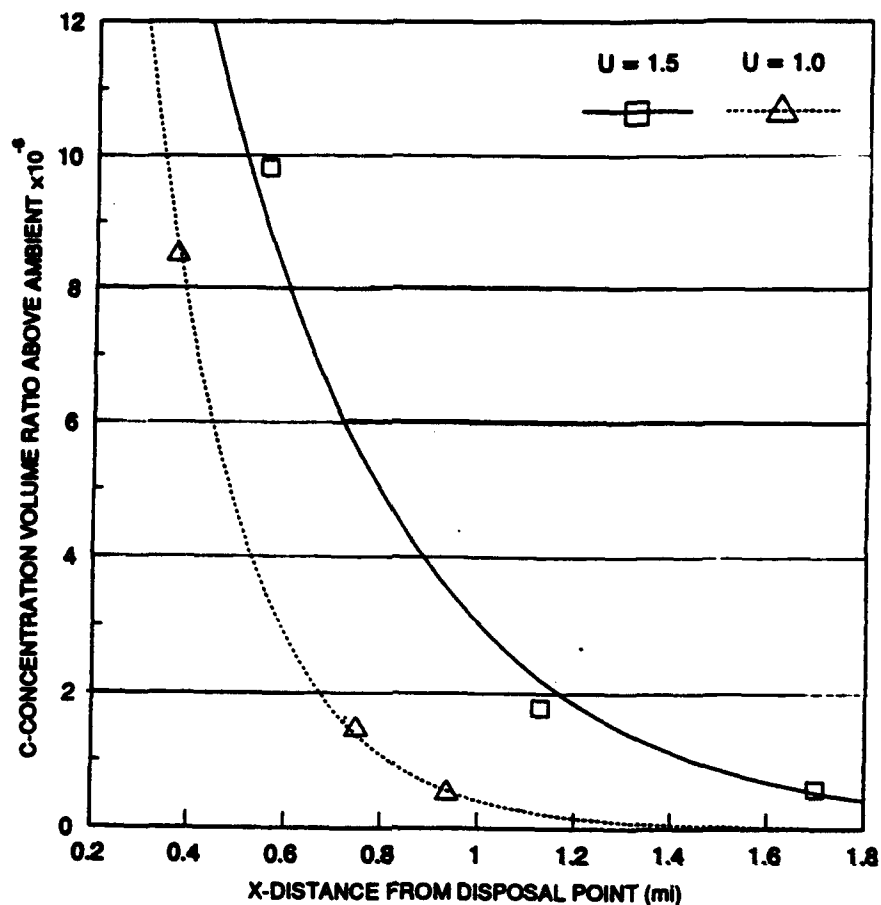
Figure 39. Evolution of depth-averaged peak plume concentration for Cases 3 and 4 of fine-grained material
