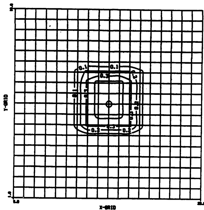
Figure 38. Contour plot of the coarse-grained site deposition pattern (Case 4)
