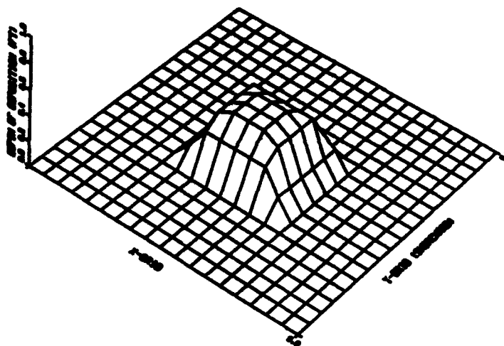
Figure 35. Three-dimensional view of the coarse-grained site deposition pattern (Case 3)
