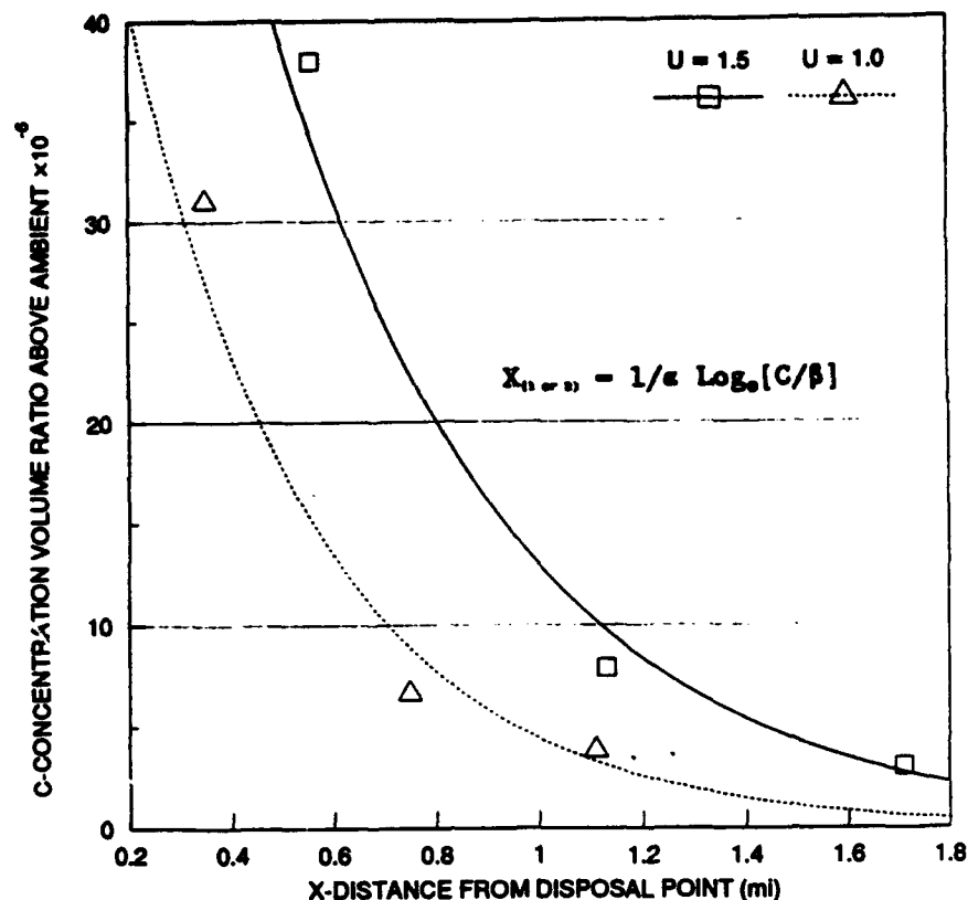
Figure 30. Evolution of depth-averaged peak plume concentration for Cases 1 and 2 of fine-grained material
