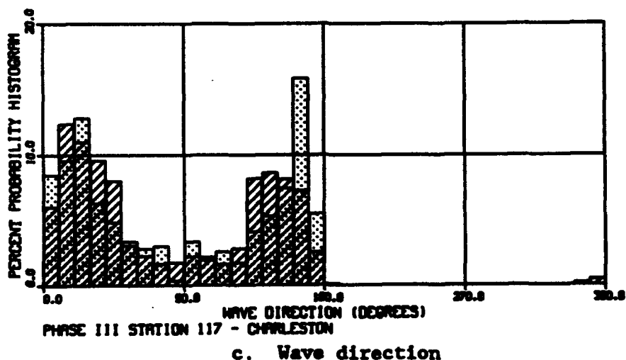
Figure 5. Probability histograms for simulated wave and 1956 WIS data
