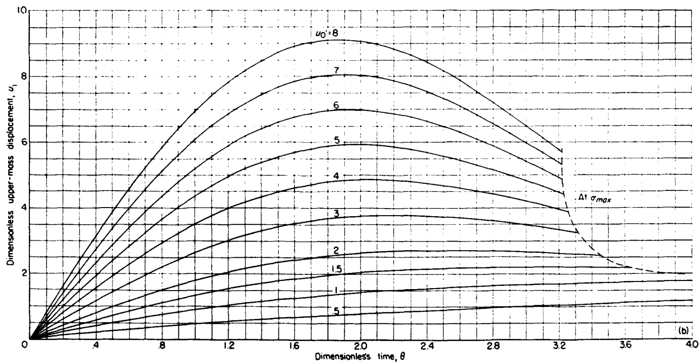
(b) Relationship between upper-mass displacement and time.
