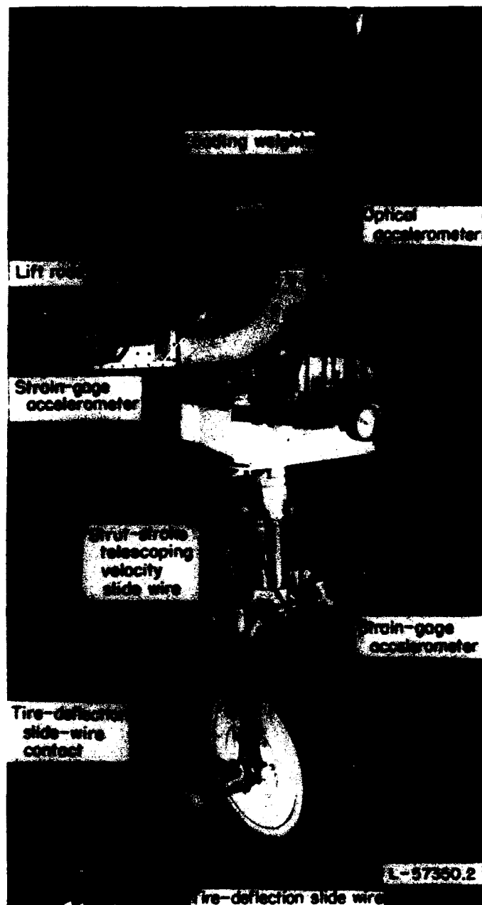
FIGURE 15.—View of landing gear and instrumentation.
