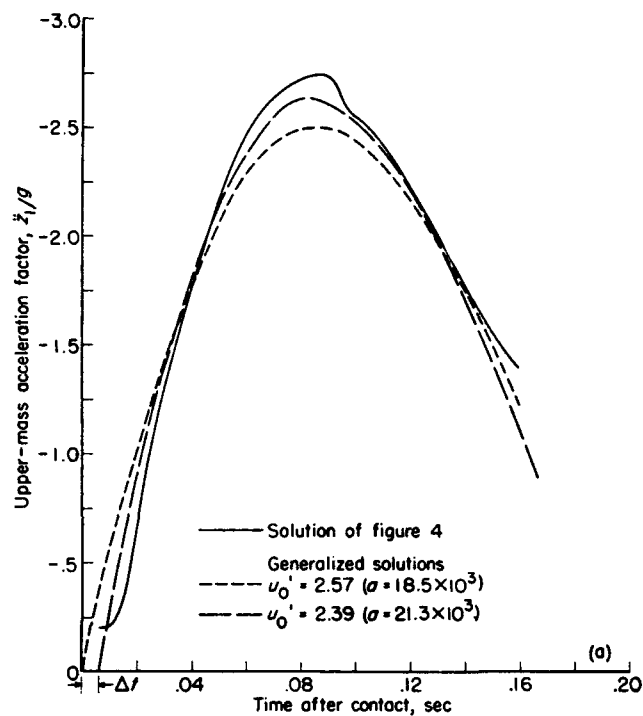
(a) Time history of upper-mass acceleration.
