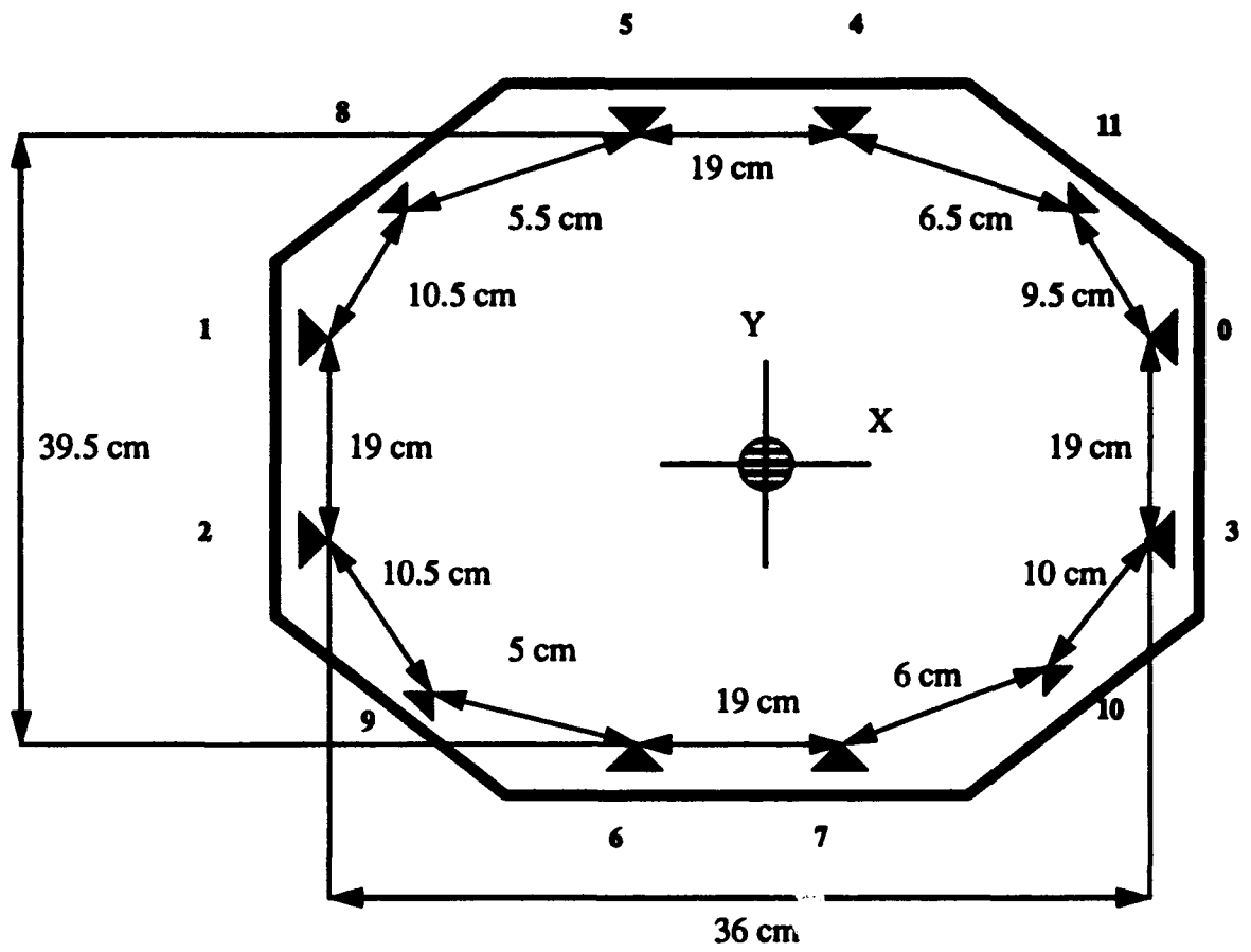
Figure 9: Sonar positions on Yamabico
