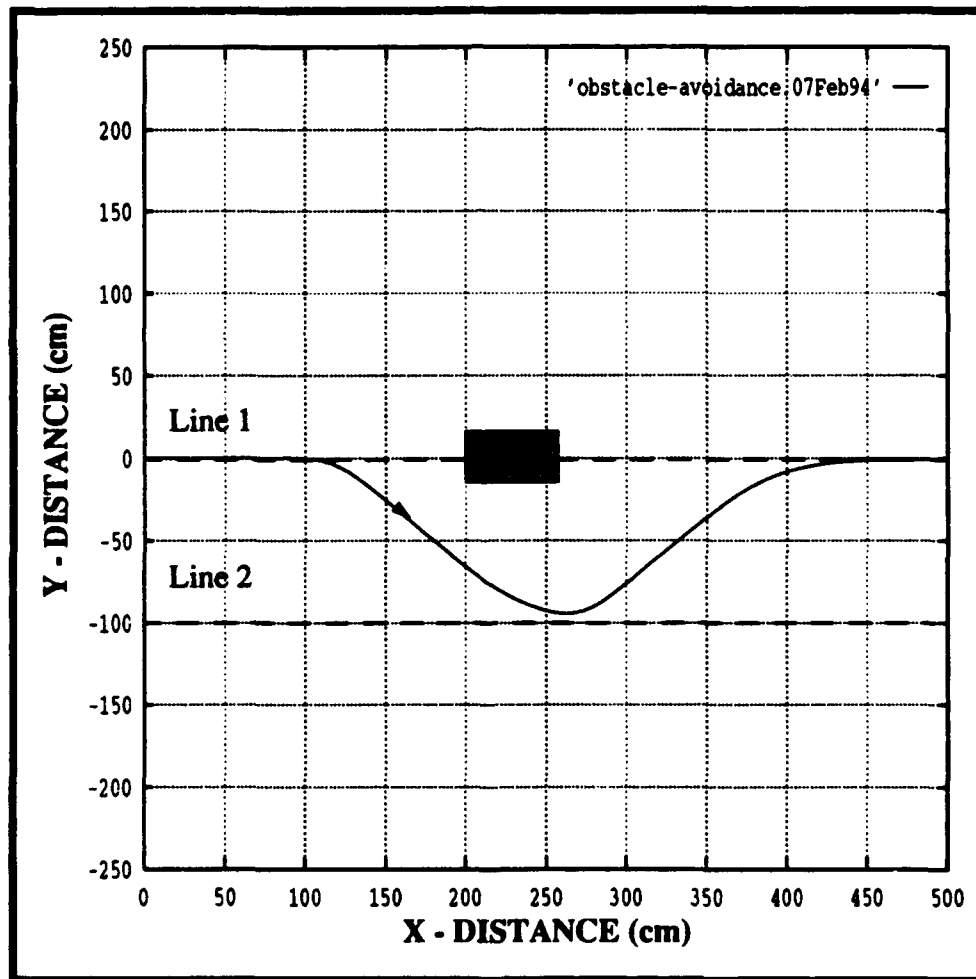
Figure 35: Obstacle avoidance results
