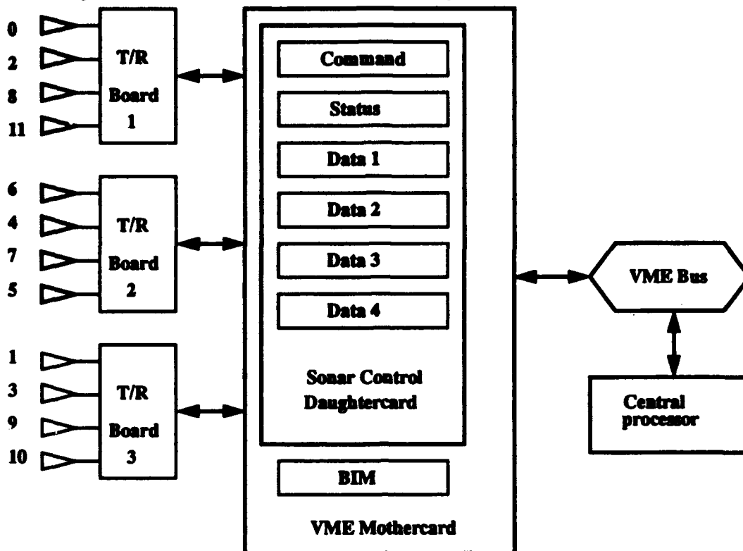
Figure 3: Sonar Hardware Architecture
