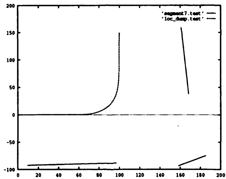
Figure 15: Path and sonar segment data
