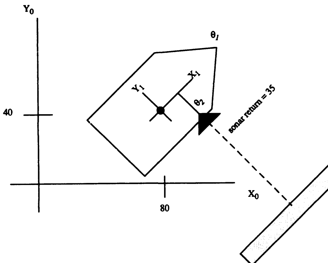
Figure 7: Example of Compose with sonar return
