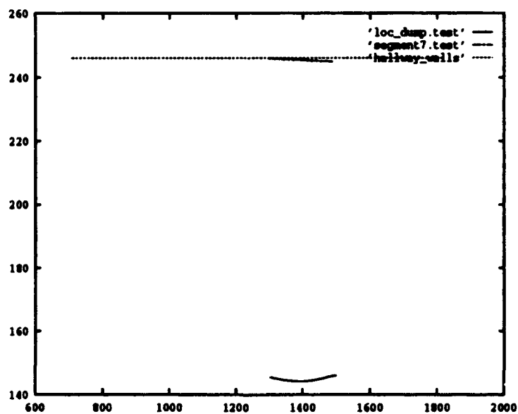
Figure 12: Local trace and segment sonar data from translational scan
