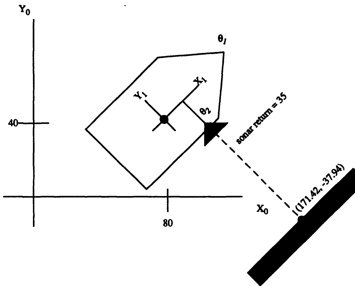
Figure 8: Result of compose on example
