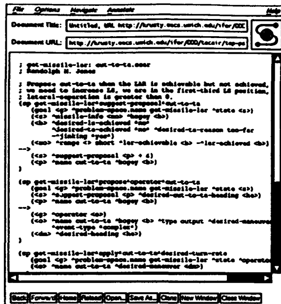
Figure 5: The Soar productions for cut-to-ta.
