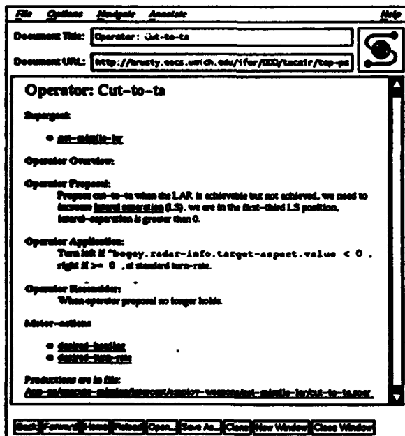
Figure 4: The Cut-to-ta PSCM document.
