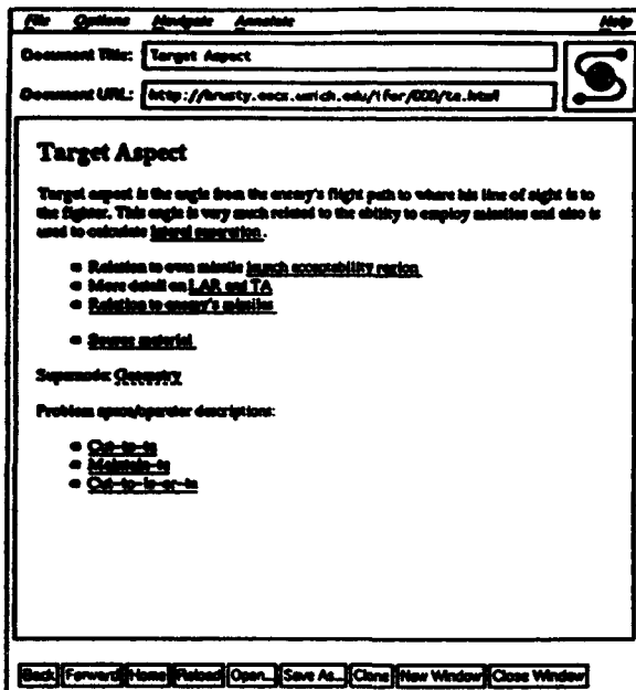
Figure 3: The Target Aspect Knowledge Document.
