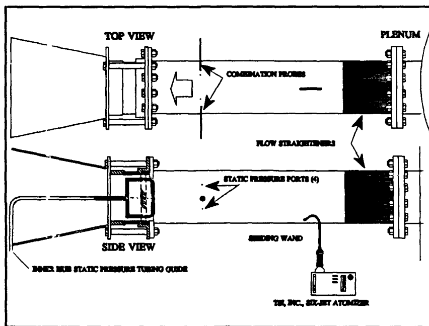
Figure 1. Supply Pipe Schematic
