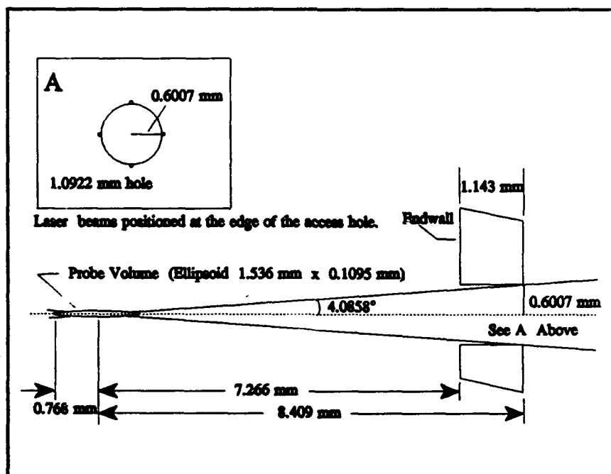
Figure 10. Endwall LDV Alignment Technique
