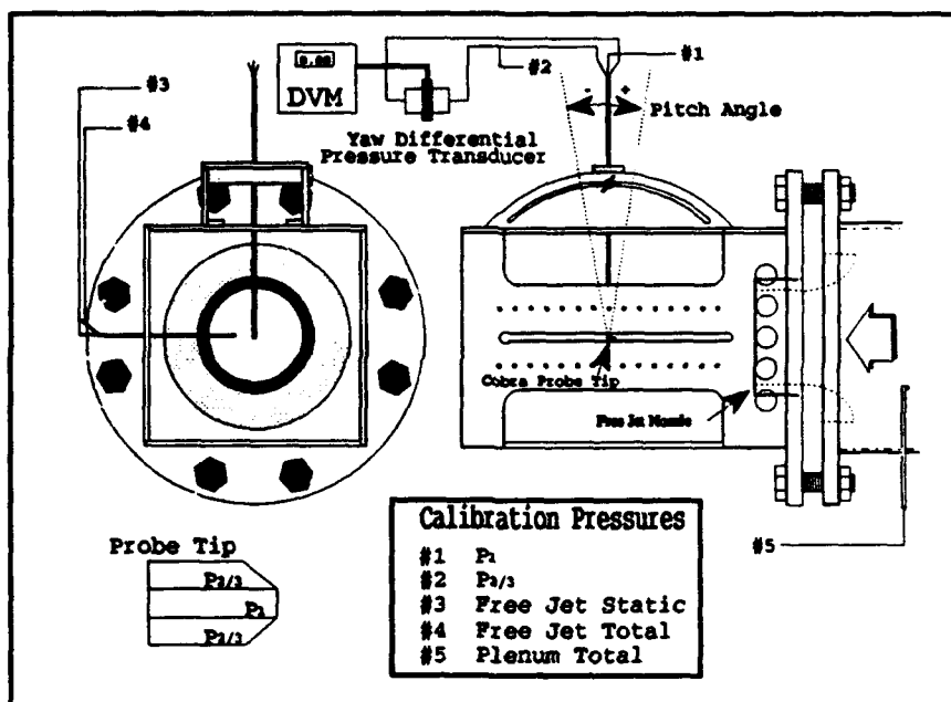
Figure 9. Yaw Probe Calibration Equipment
