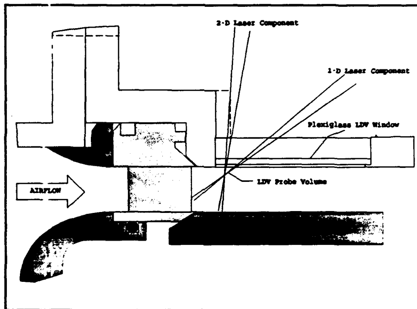
Figure 6. LDV Access Modifications
