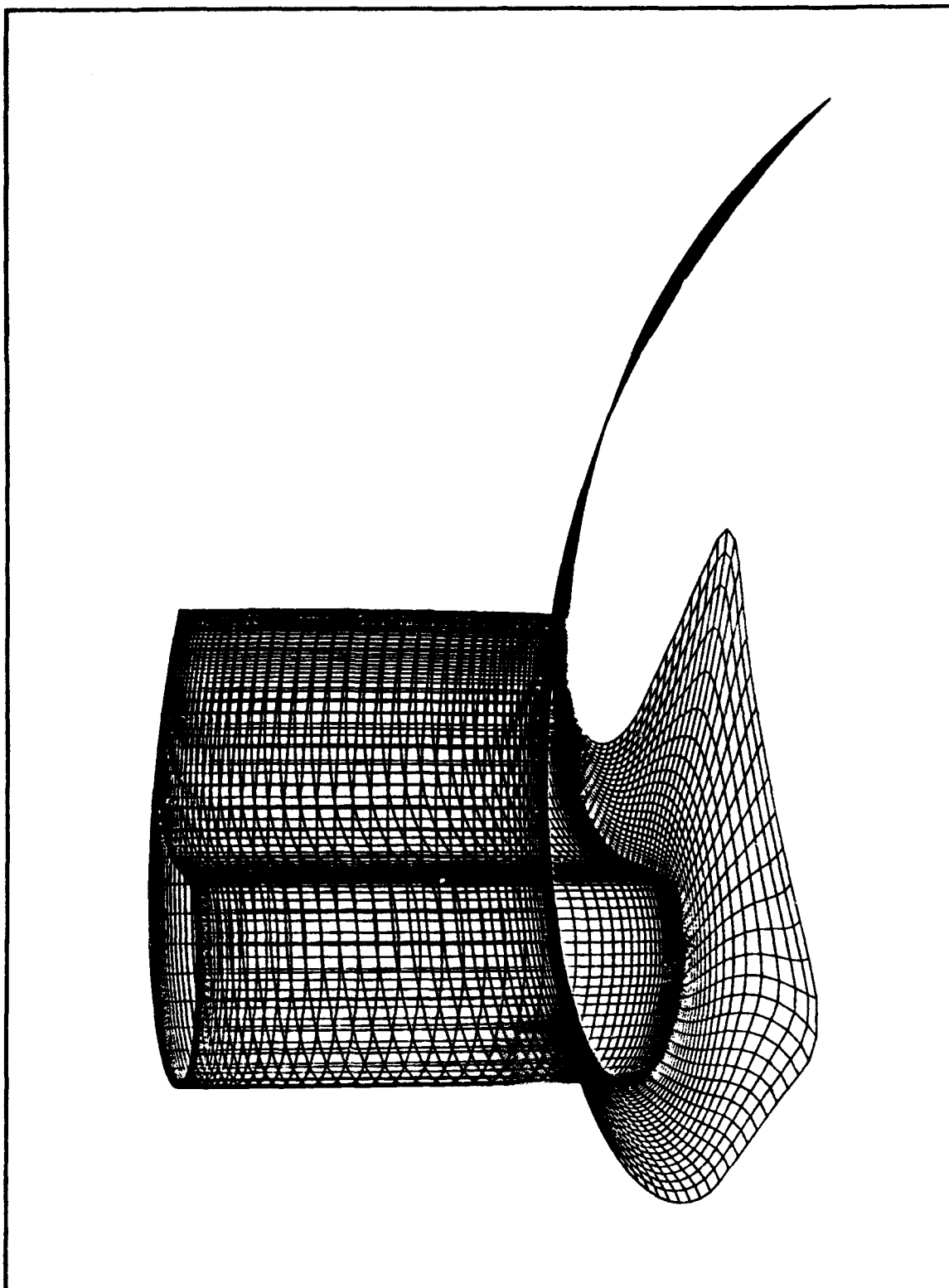
Figure C2. Grid Geometry, 3-D Perspective
