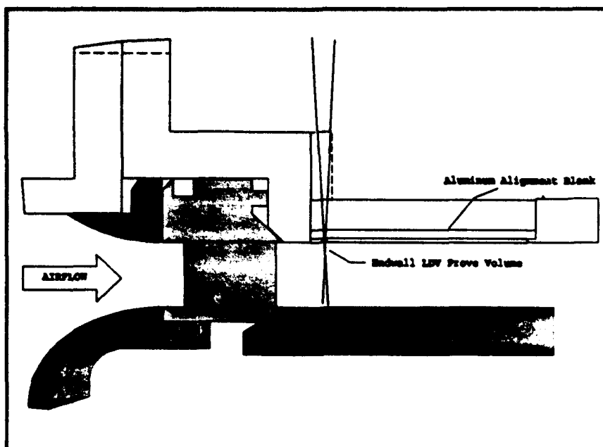
Figure 7. Endwall Measurement Technique
