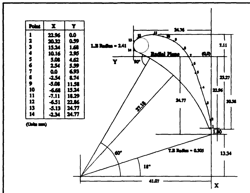
Figure 3. Blade Geometry
