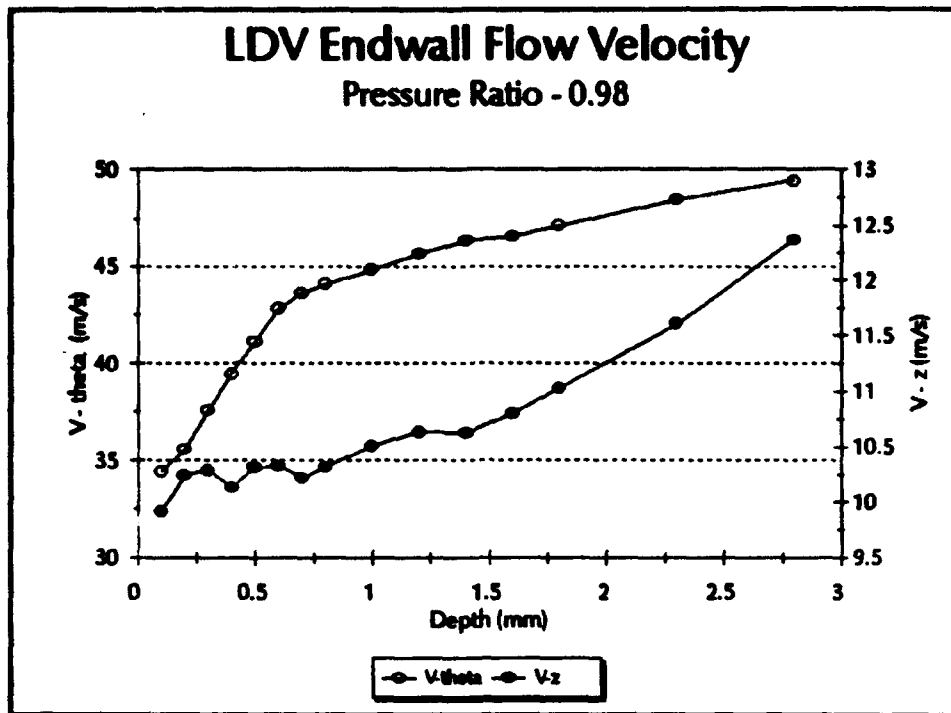
Figure 16. Single Component LDV Endwall Velocity
