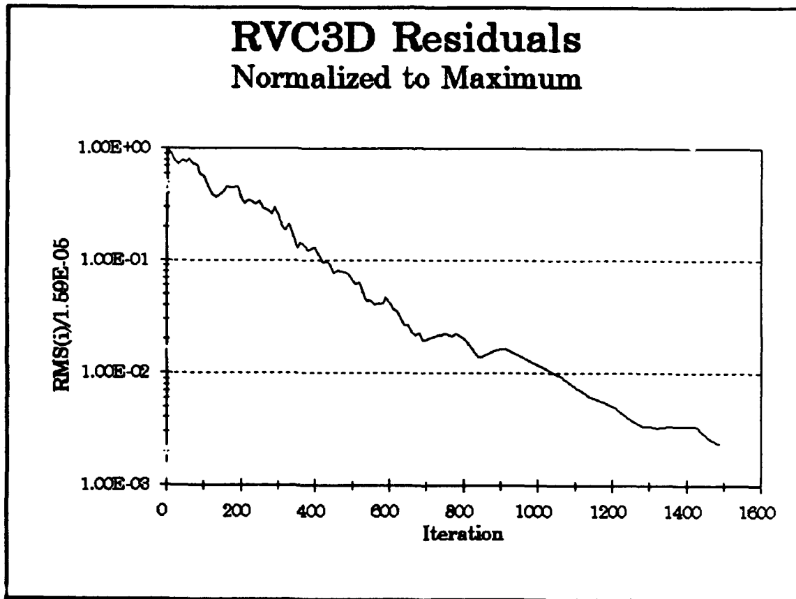
Figure D1. RVC3D Residuals
