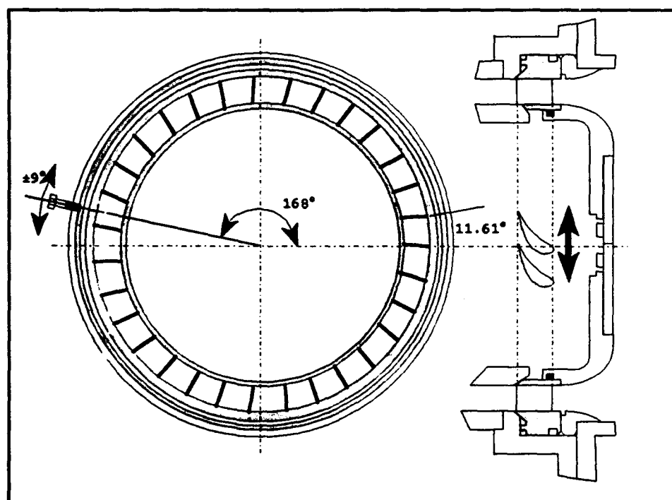
Figure 4. Wake Positioning System
