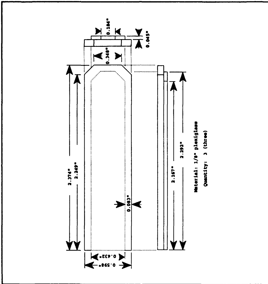
Figure A7. Plexiglas Window
