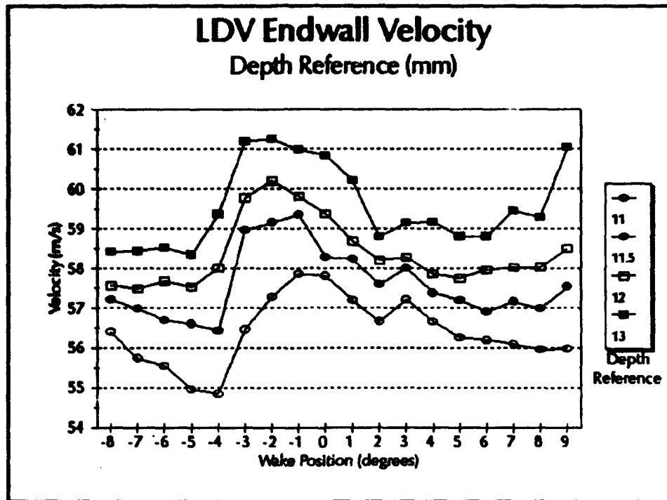
Figure 18. Two Component LDV Endwall Velocity
