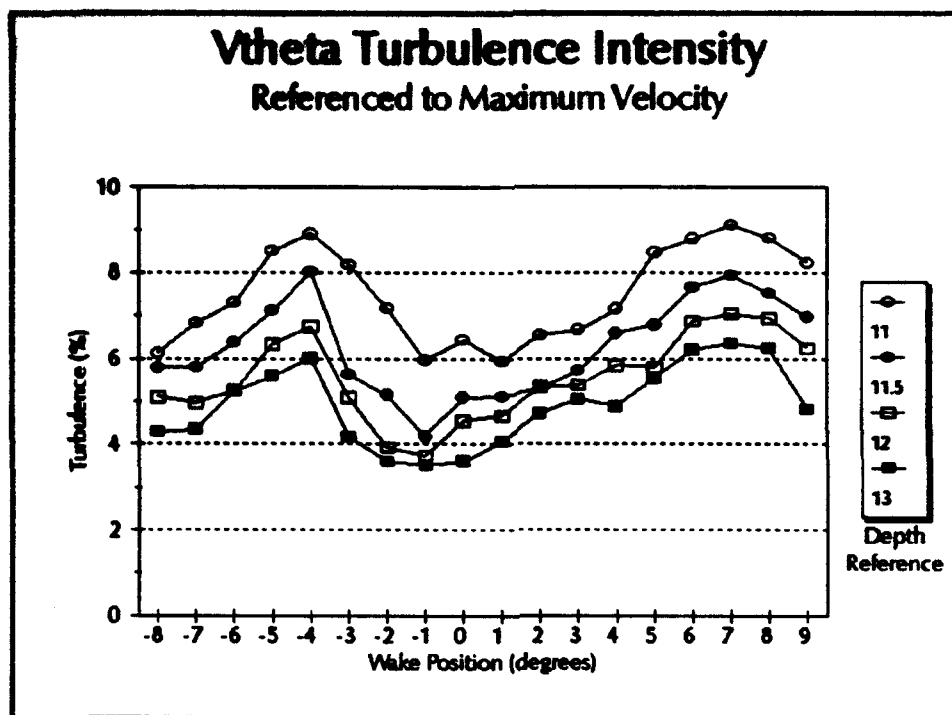
Figure 20. Two Component LDV Turbulence, V-theta
