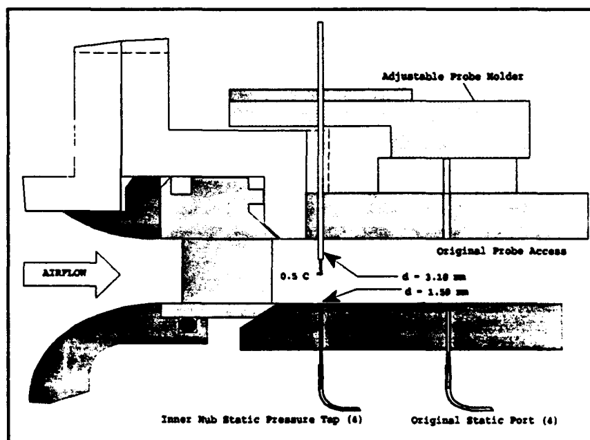
Figure 5. Pressure Measurement Changes
