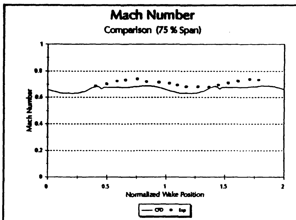
Figure 31. Mach Number Comparison, 75%
