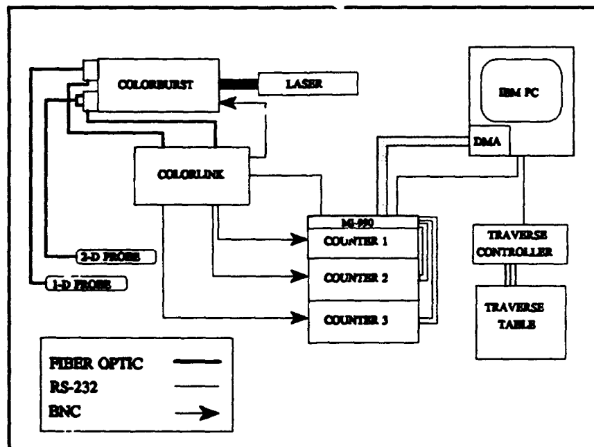
Figure 8. LDV Wiring Schematic
