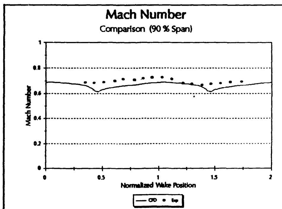
Figure 32. Mach Number Comparison, 90%
