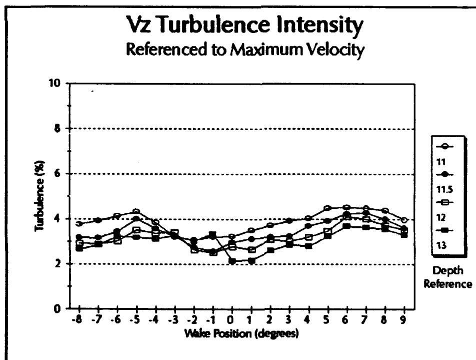
Figure 21. Two Component LDV Turbulence, V-z
