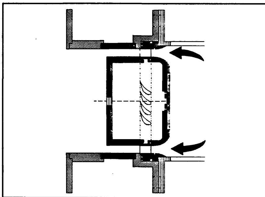
Figure 2. Annular Turbine Cascade Cutaway
