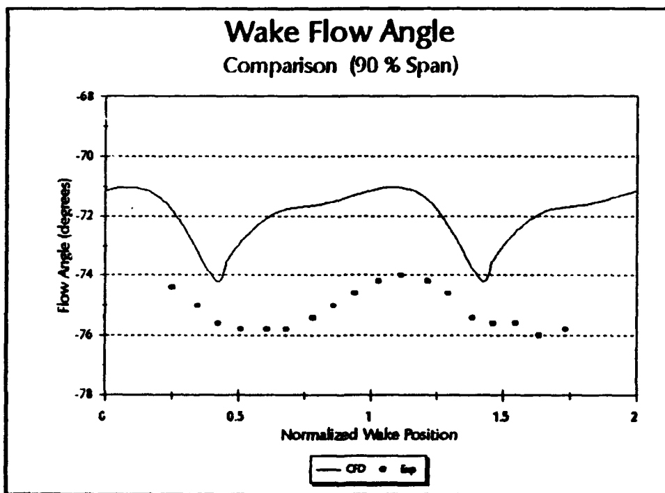
Figure 36. Flow Angle Comparison, 90%
