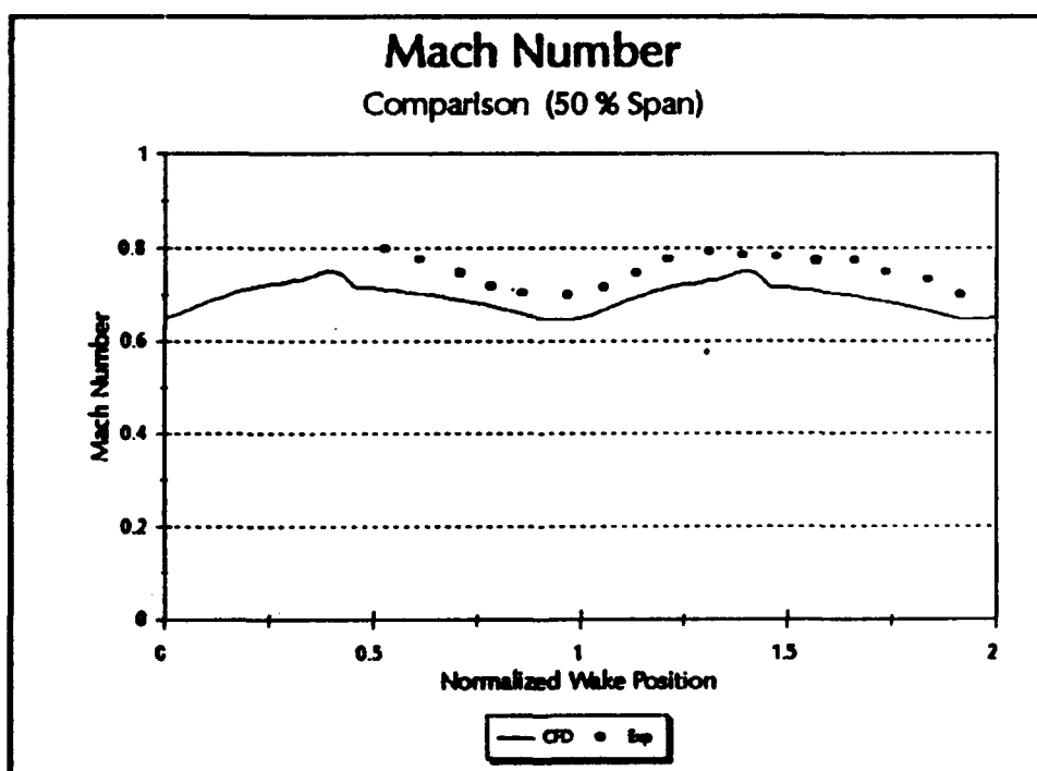
Figure 30. Mach Number Comparison, 50%
