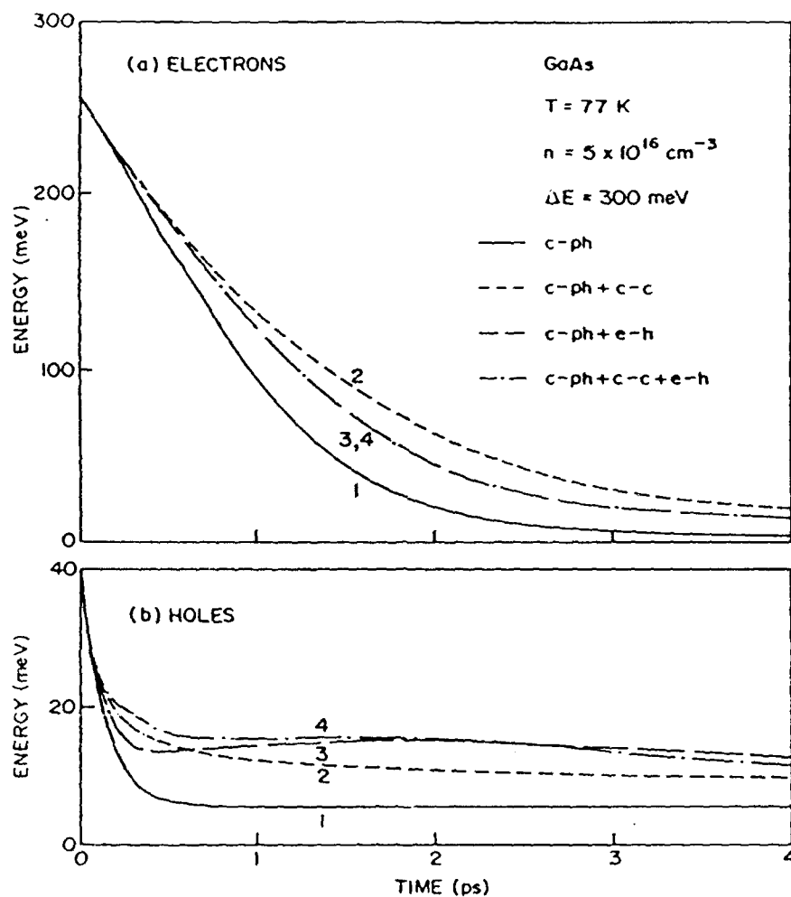
Figure 5. Time evolution of the carrier energy for different active scattering mechanisms (a) electrons, (b) holes.
