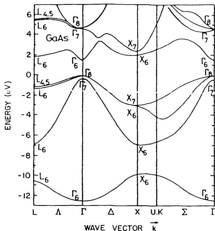
Figure 1.1 Band structure of the semiconductor gallium arsenide [4]. (Reprinted, with permission, from Physical Review [Section] B: Solid State. )
