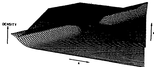
Figure 3. Density Matrix on the (x, x') Plane
