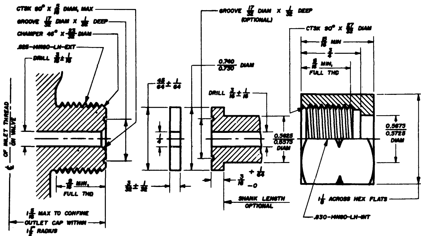
VALVE OUTLET NO. 331
