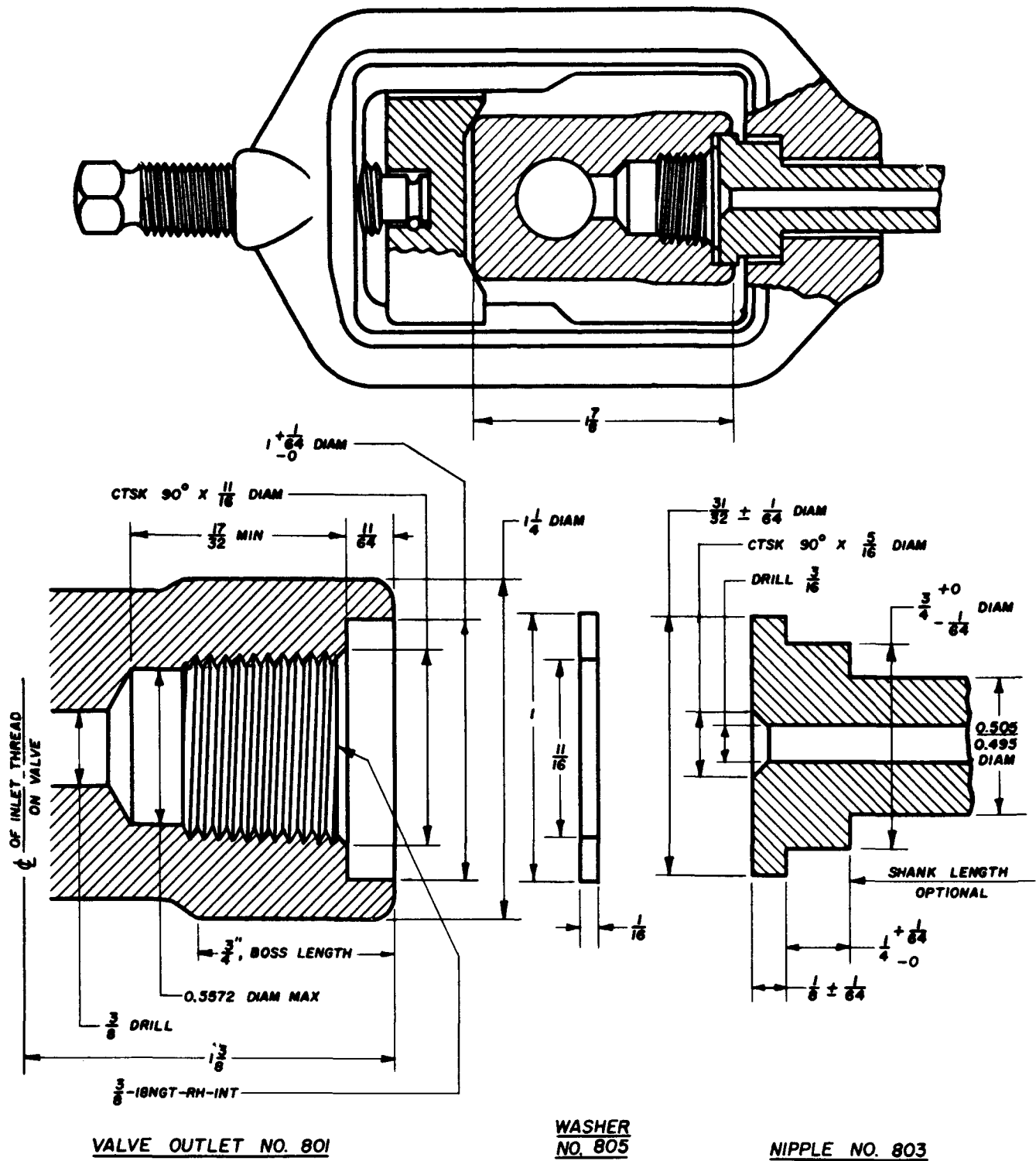
FIGURE IX.23.—No. 800 standard valve outlet connection, yoke type, for ammonia, anhydrous.
