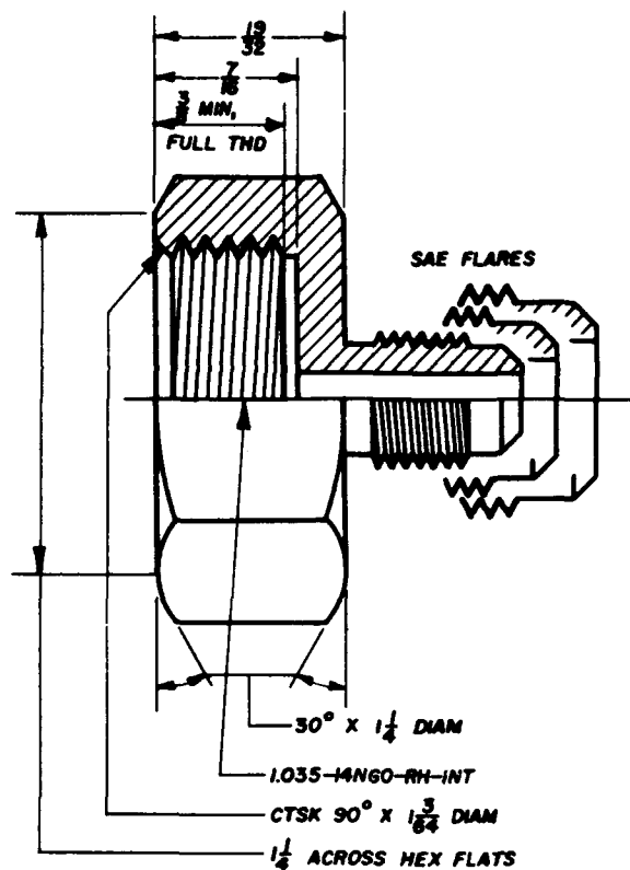
CONVERTER NO. 624
