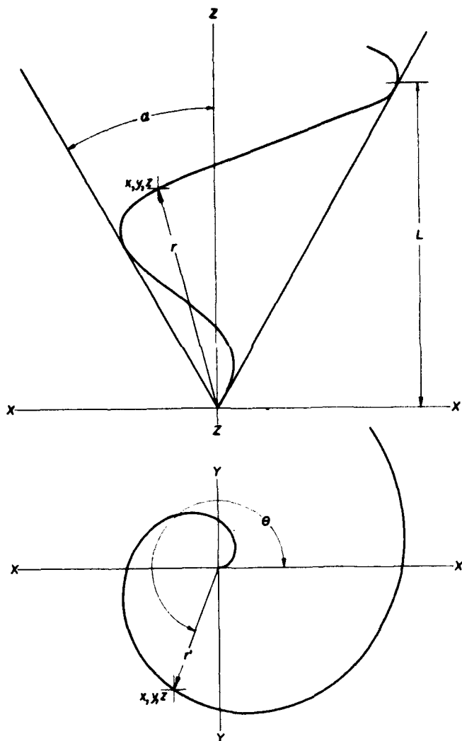
FIGURE 8.1.—The conical spiral.
