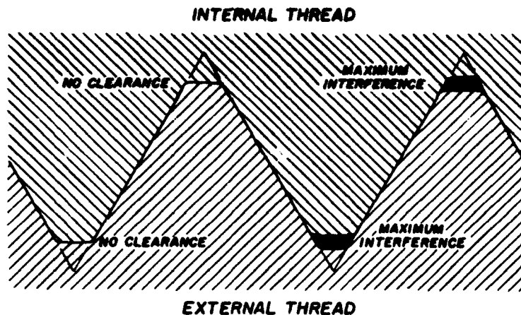
FIGURE VIII.1.—Dryseal American Standard pipe threads for pressure-tight joints.
