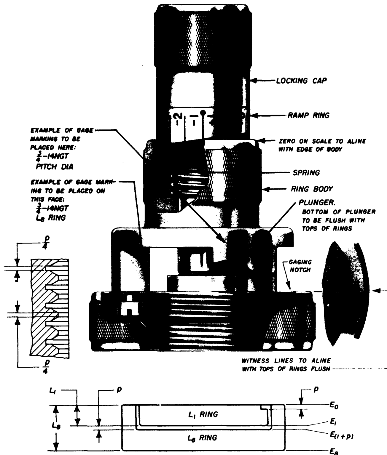
FIGURE IX.36.—Pitch diameter ring gages; NGT, SGT.
