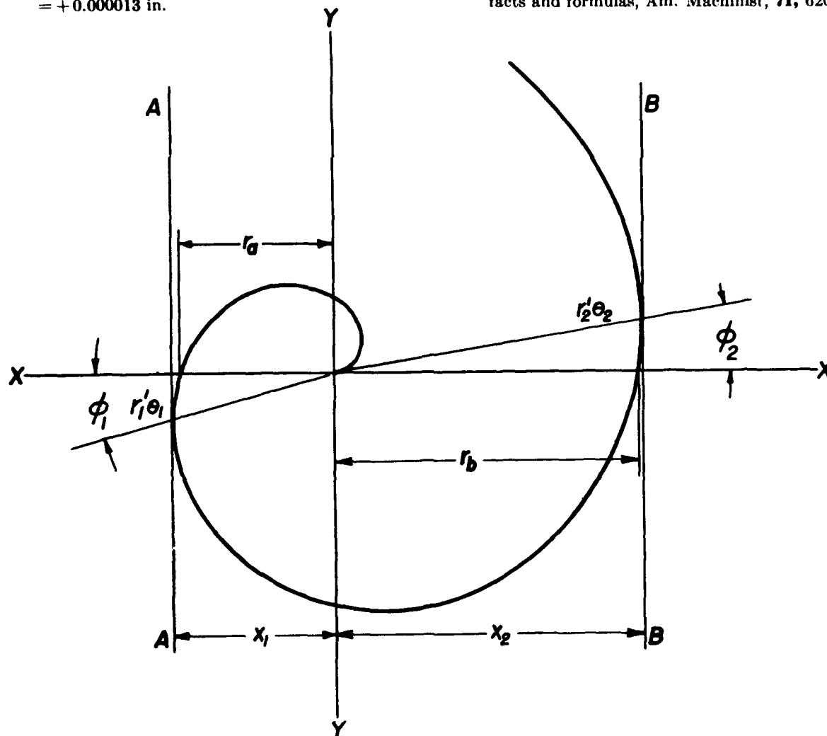
FIGURE 8.4.—Measurement of Archimedes' spiral.
