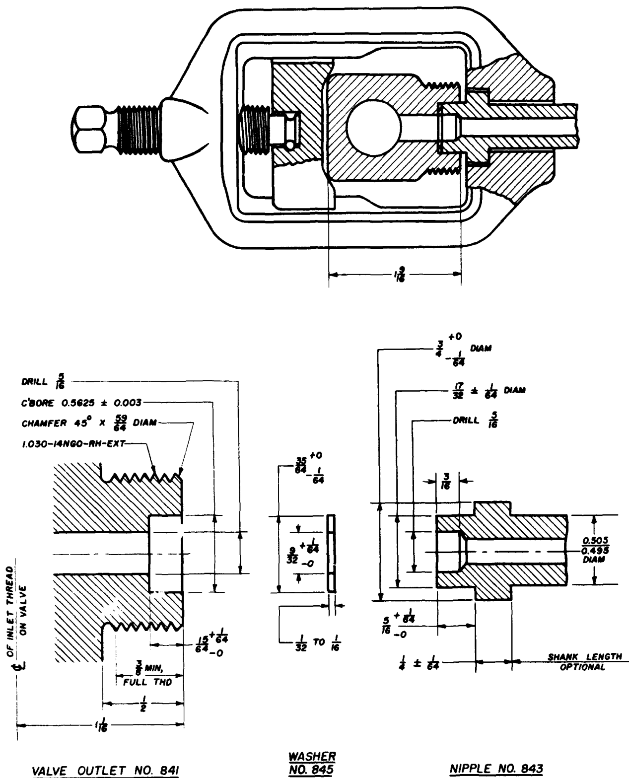
FIGURE IX.25.—No. 840 standard valve outlet connection, yoke type, for chlorine (with washer inside of recess).
