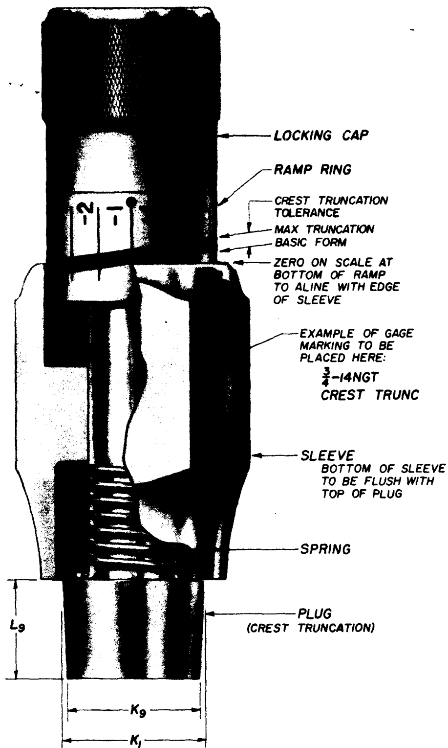
FIGURE IX.40.—Crest truncation plug gage; NGT, SGT.
