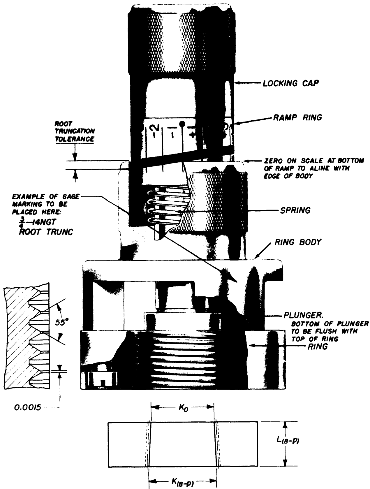
FIGURE IX.38. Root truncation ring gage; NGT, SGT.
