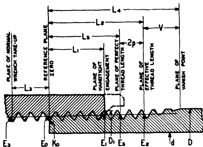
FIGURE VII.3.—American Standard taper pipe thread notation.
