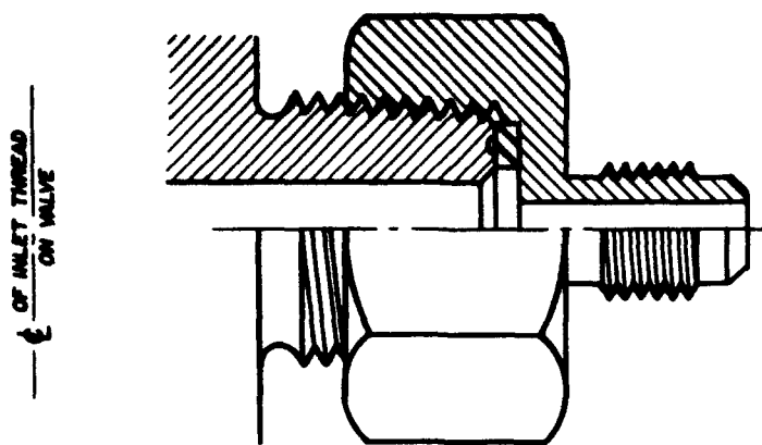
CONNECTION NO. 360
