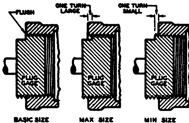
FIGURE VII.8.—Gaging internal taper threads.
