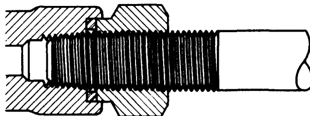
TYPICAL LOCKNUT CONNECTION
