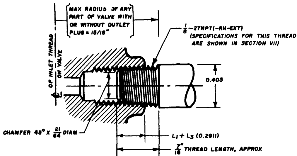
PIPE CONNECTION NO. 163
