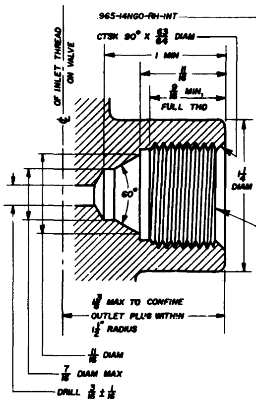
VALVE OUTLET NO. 581
