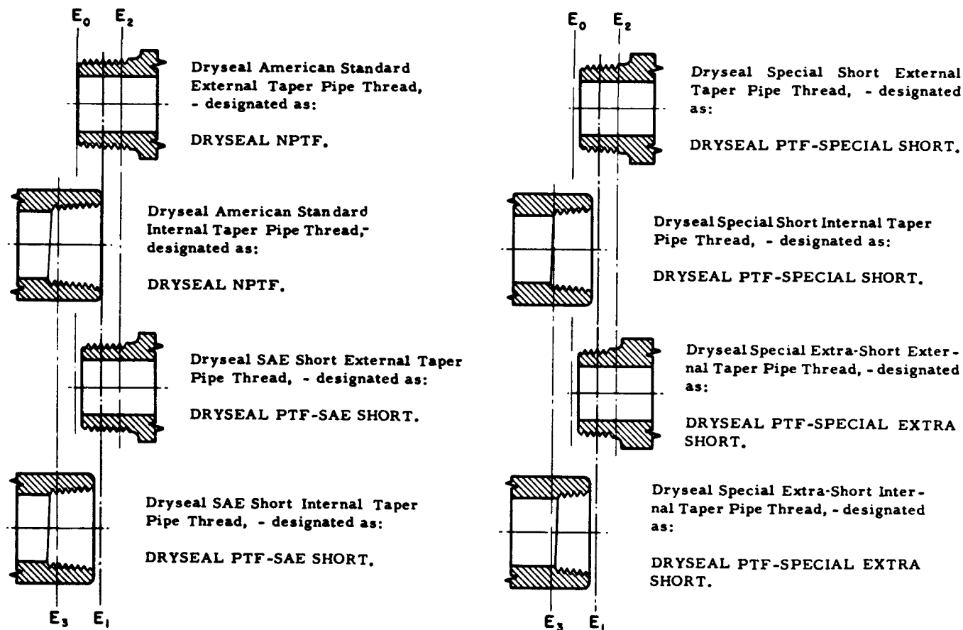
FIGURE 7.2.—Comparison of special length Dryseal threads with standard length Dryseal threads.
