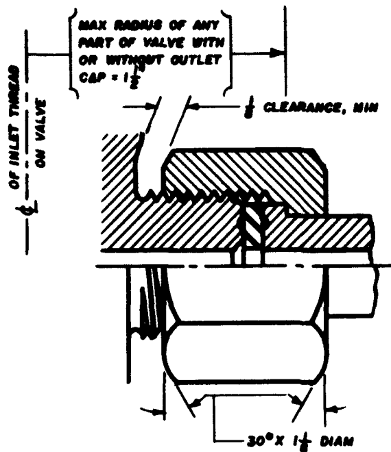
CONNECTION NO. 320
