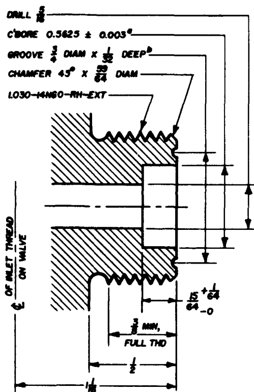
VALVE OUTLET NO. 621
