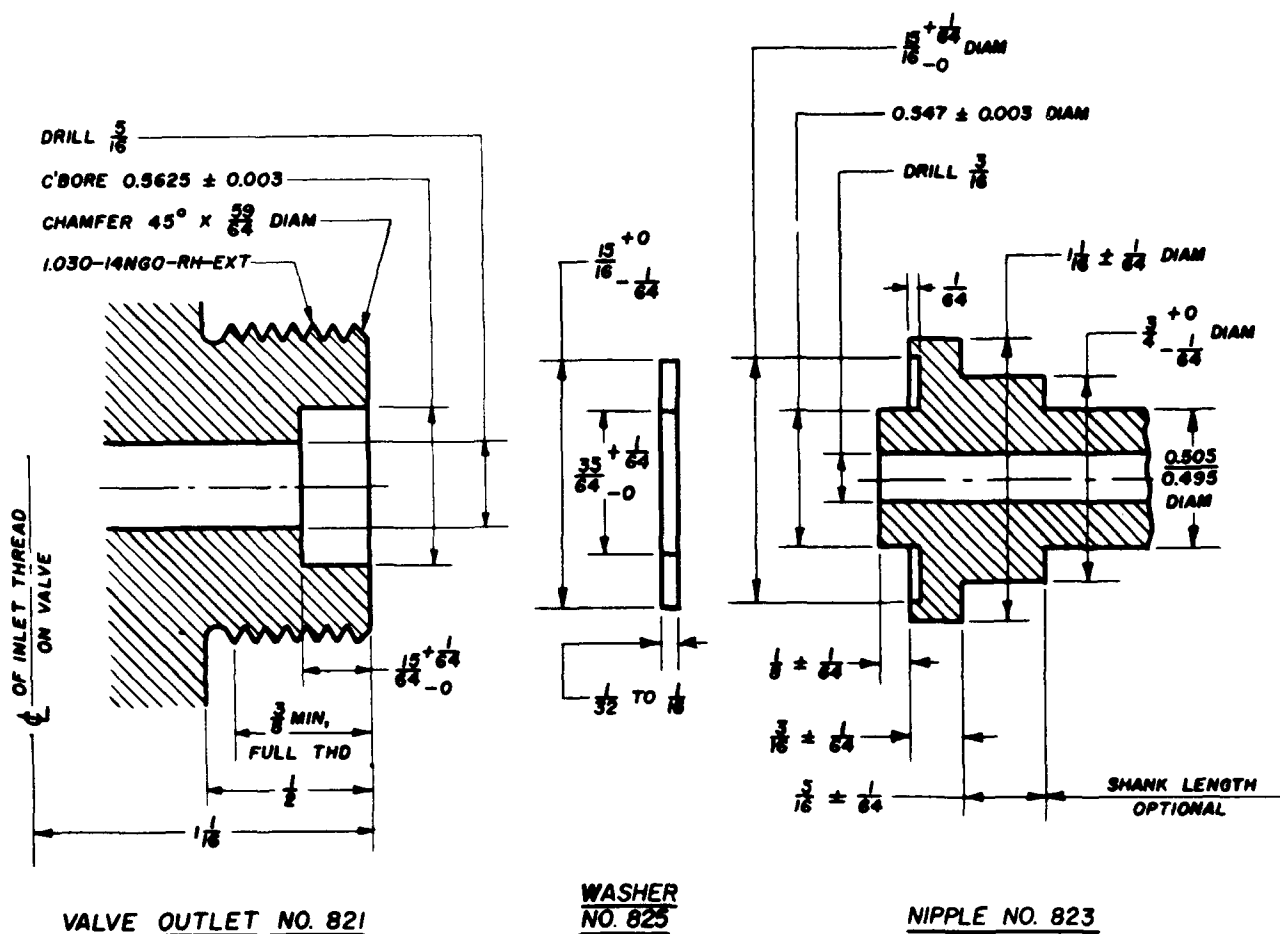
FIGURE IX.24.—No. 820 standard valve outlet connection, yoke type, for chlorine (with washer on outer face).
