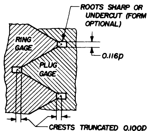
FIGURE VII.5.—Form of gage thread.
