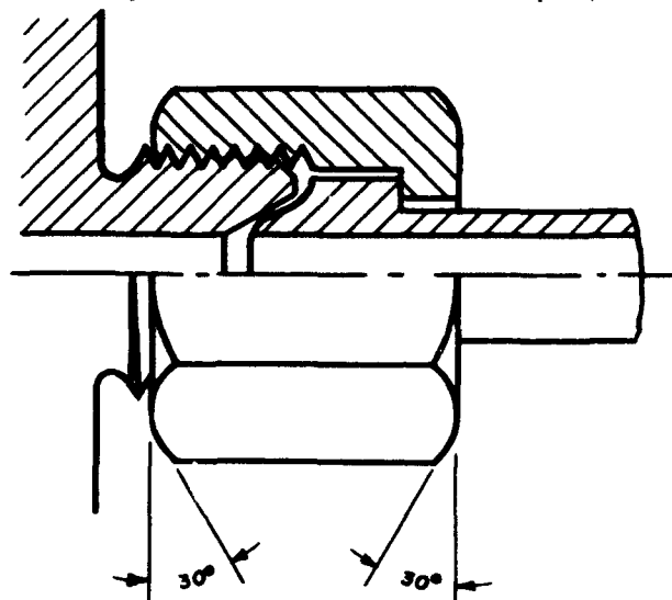
CONNECTION NO. 120
