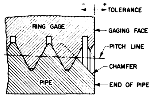
(A) ENLARGED VIEW SHOWING CHAMFERED EXTERNAL THREAD OF BASIC SIZE
