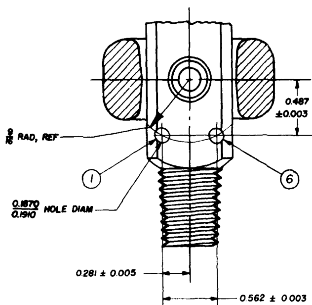
VALVE OUTLET NO. 941
