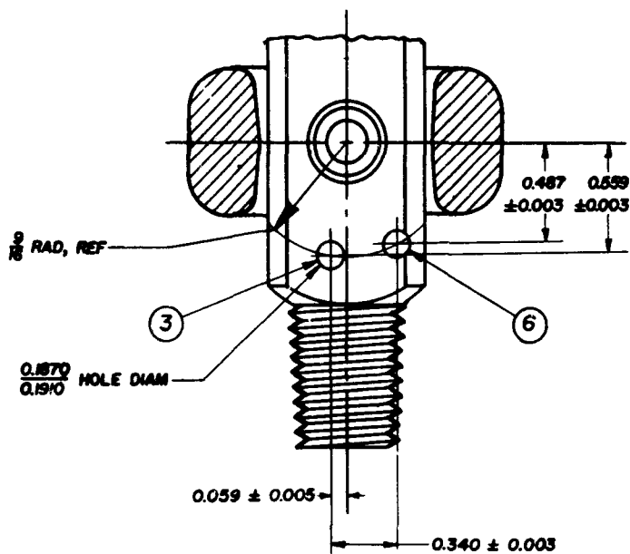
VALVE OUTLET NO. 921
