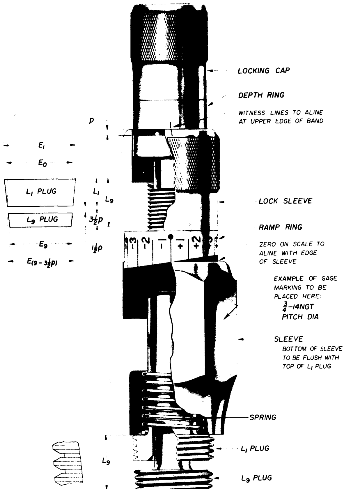
FIGURE IX.39.—Pitch diameter plug gage; NGT, SGT.
