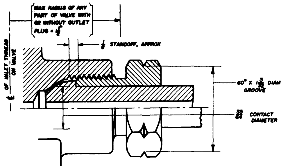
CONNECTION NO. 510
