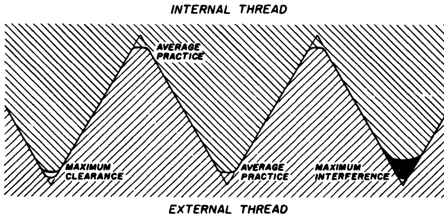
FIGURE VII.2.—American Standard taper pipe threads for pressure-tight joints, NPT.
