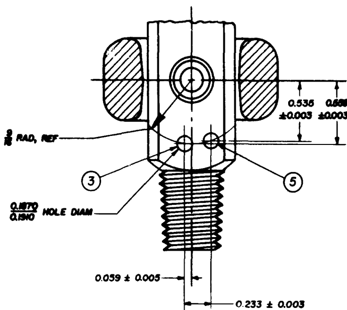
VALVE OUTLET NO. 911
