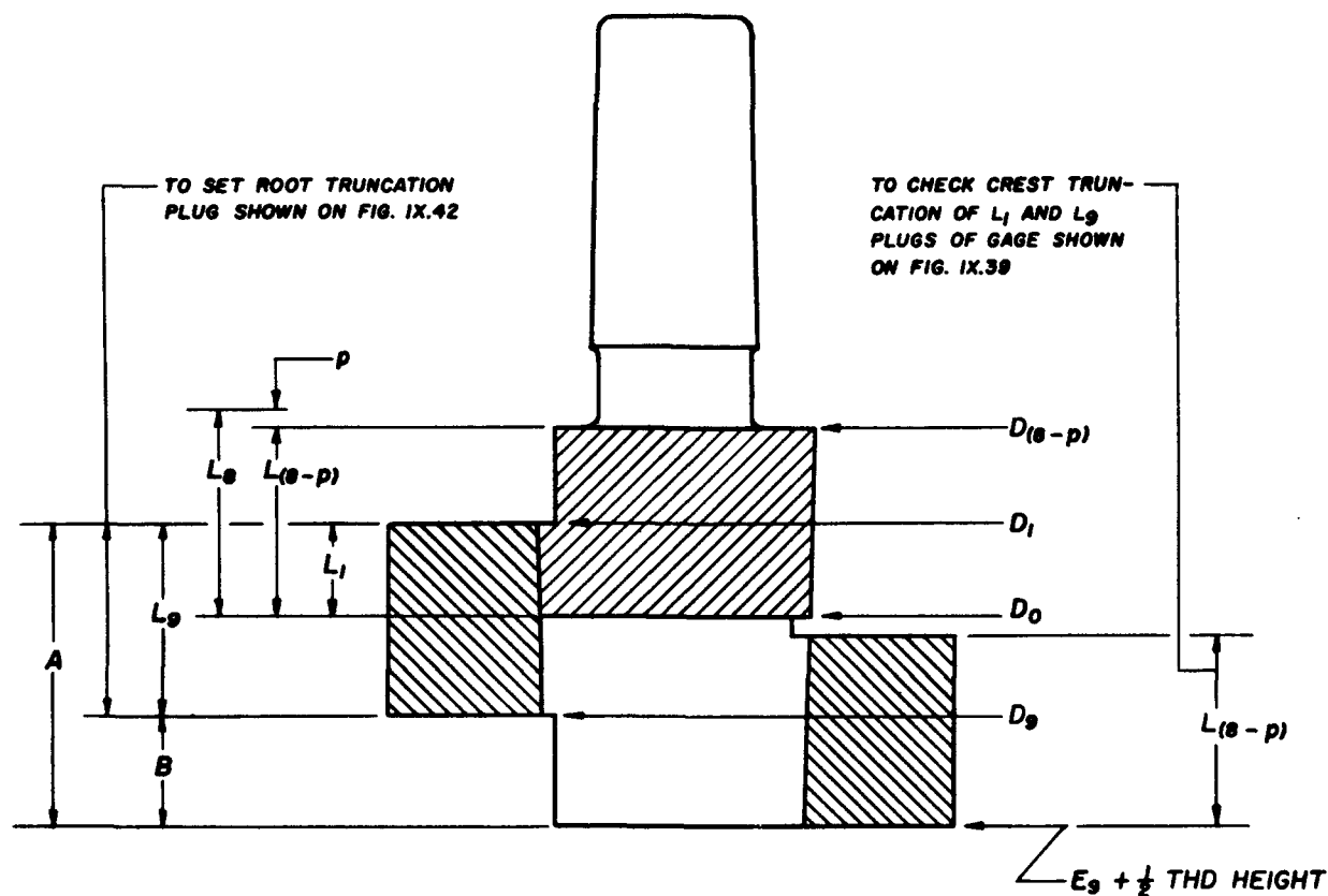
FIGURE IX.43.—Master setting plug and ring gages for setting pitch diameter of threaded plug and ring gages; NGT, SGT.
