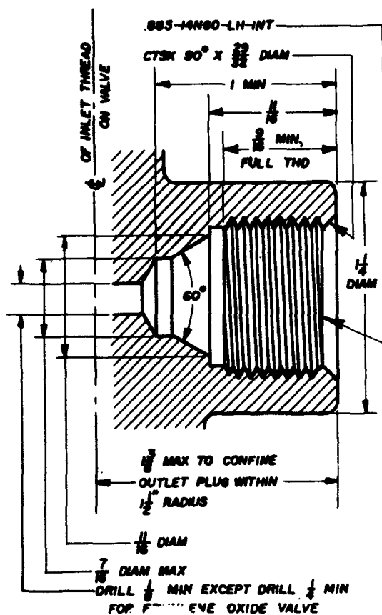
VALVE NO. 511
