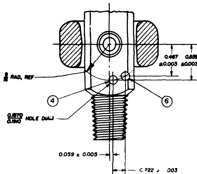
VALVE OUTLET NO. 931
