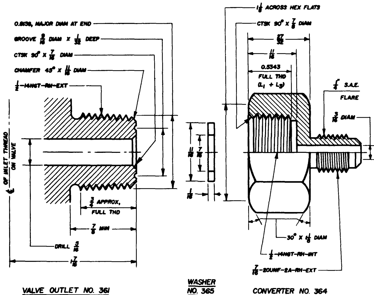
CONNECTION NO. 360
