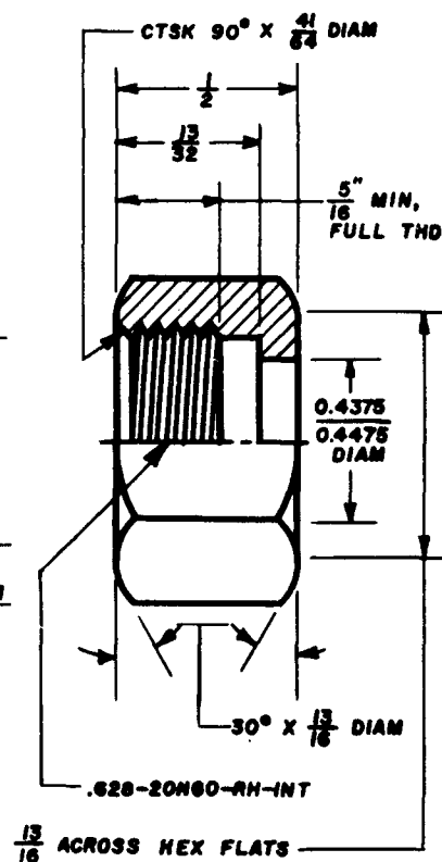
HEX NUT NO. 204
