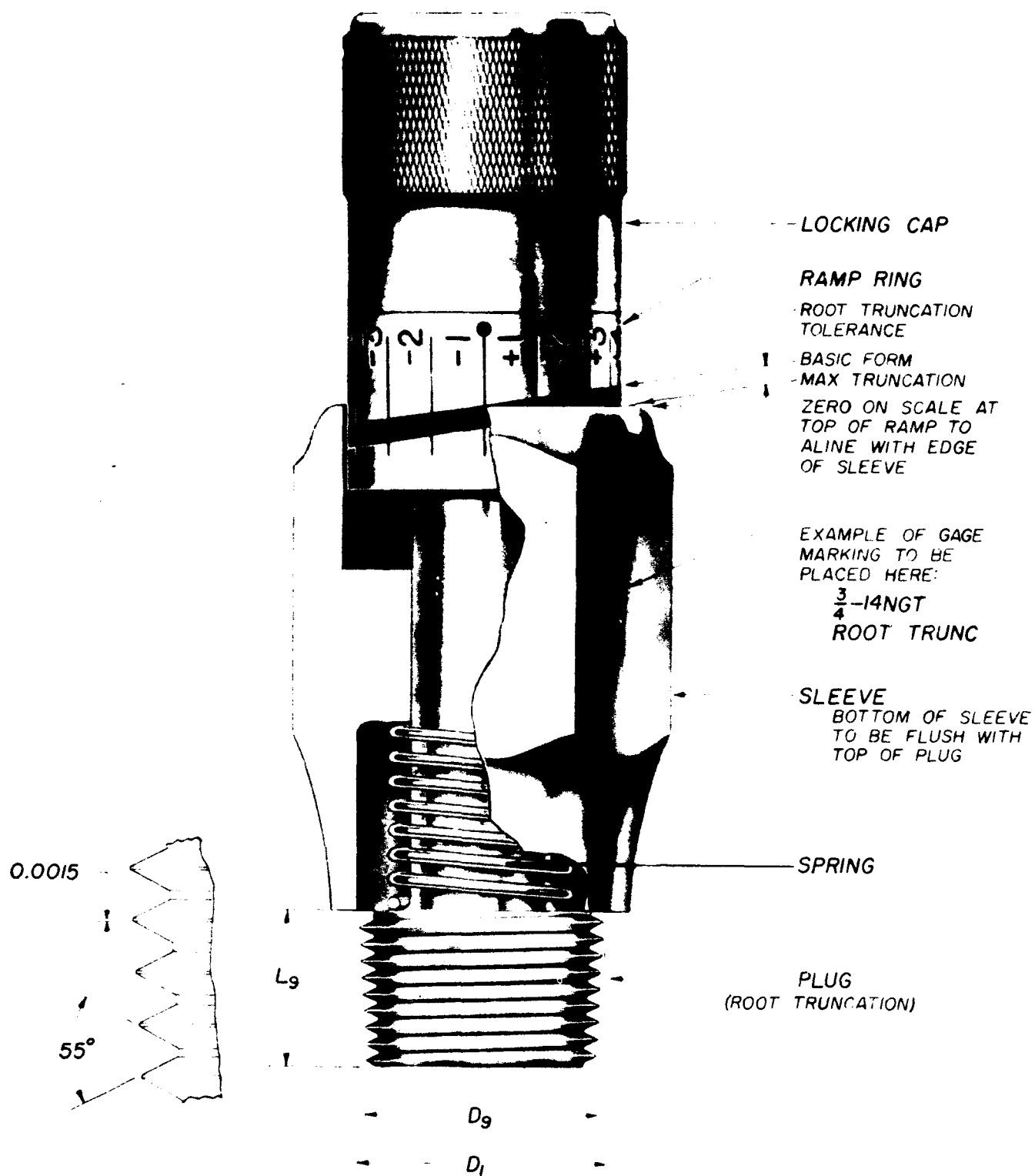
FIGURE IX.42.—Root truncation plug gage; NGT, SGT.
