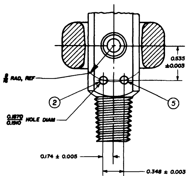
VALVE OUTLET NO. 871
