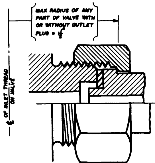
CONNECTION NO. 660
