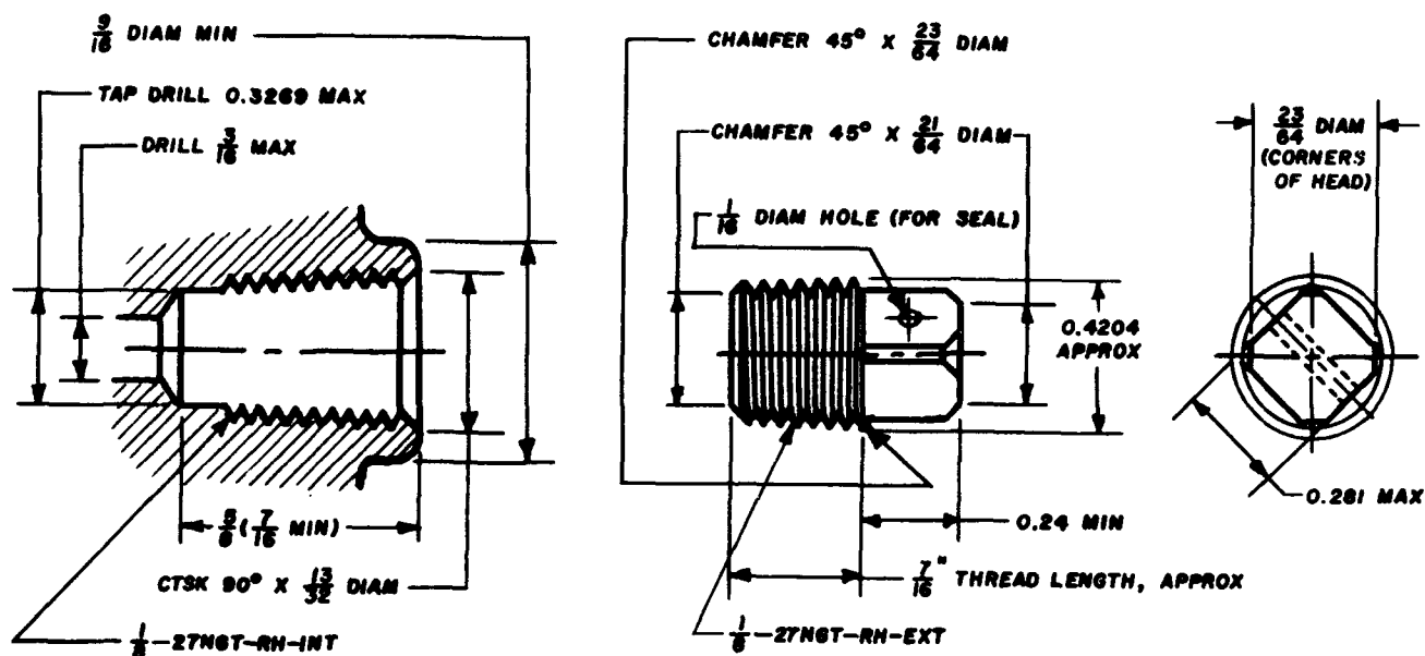
VALVE OUTLET NO. 161
