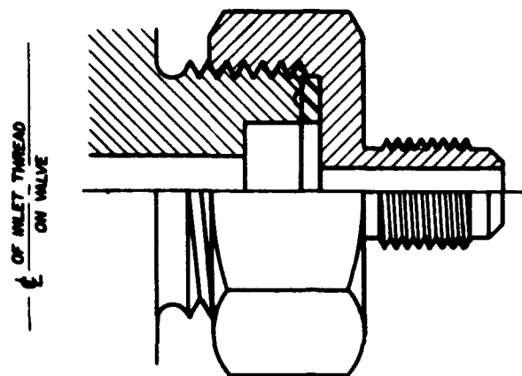
CONNECTION NO. 620
