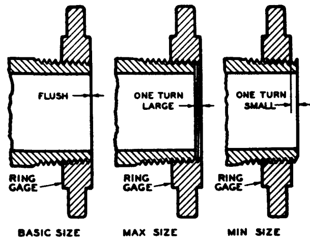
FIGURE VII.7.—Gaging external taper threads with thin ring gage.
