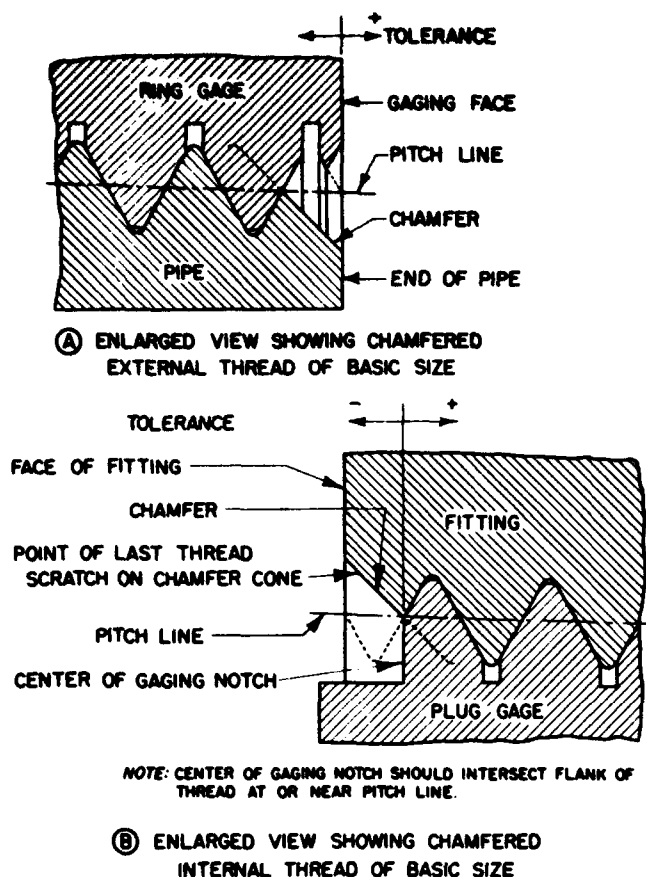
FIGURE VIII.2.—Gaging of chamfered threads (see pars. 3(a) and 3(b), pp. 27 and 28).
