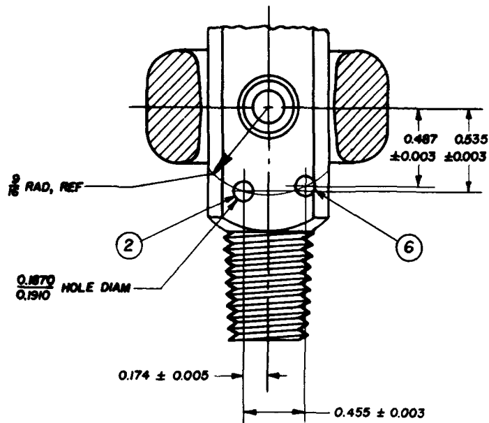
VALVE OUTLET NO. 881
