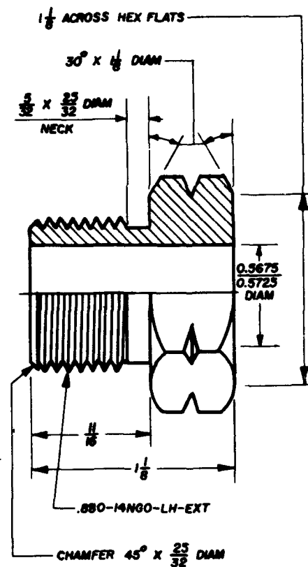
HEX NUT NO. 514
