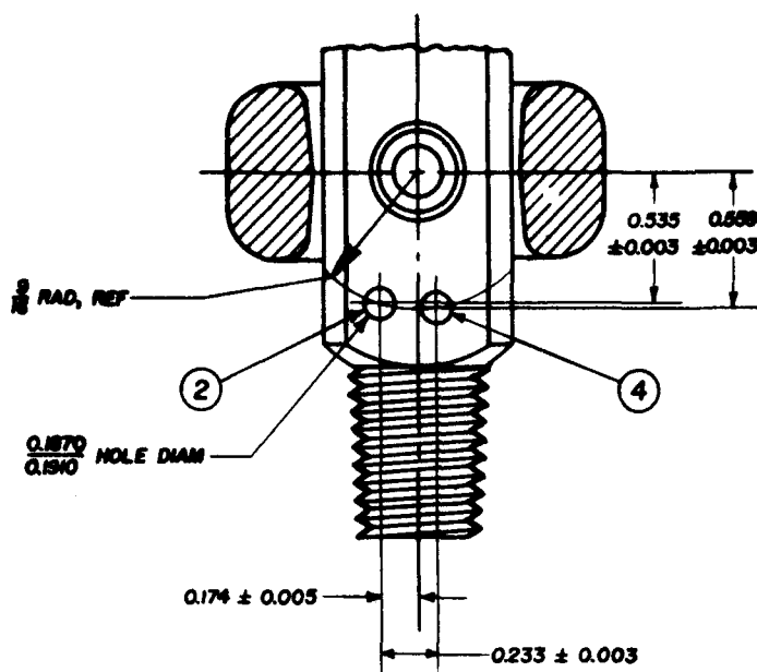
VALVE OUTLET NO. 891
