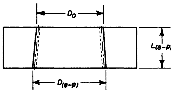
FIGURE IX.37.—Crest truncation ring gage: NGT, SGT.
