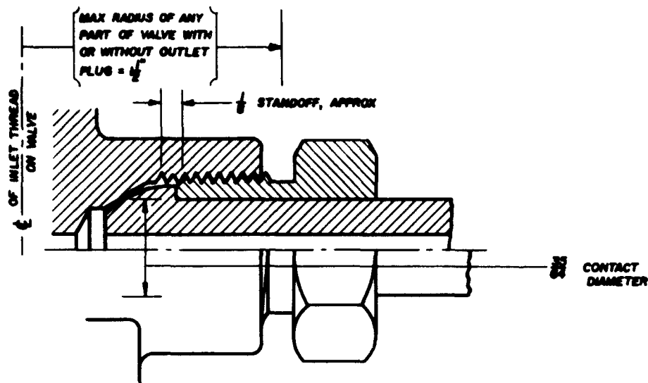
CONNECTION NO. 580
