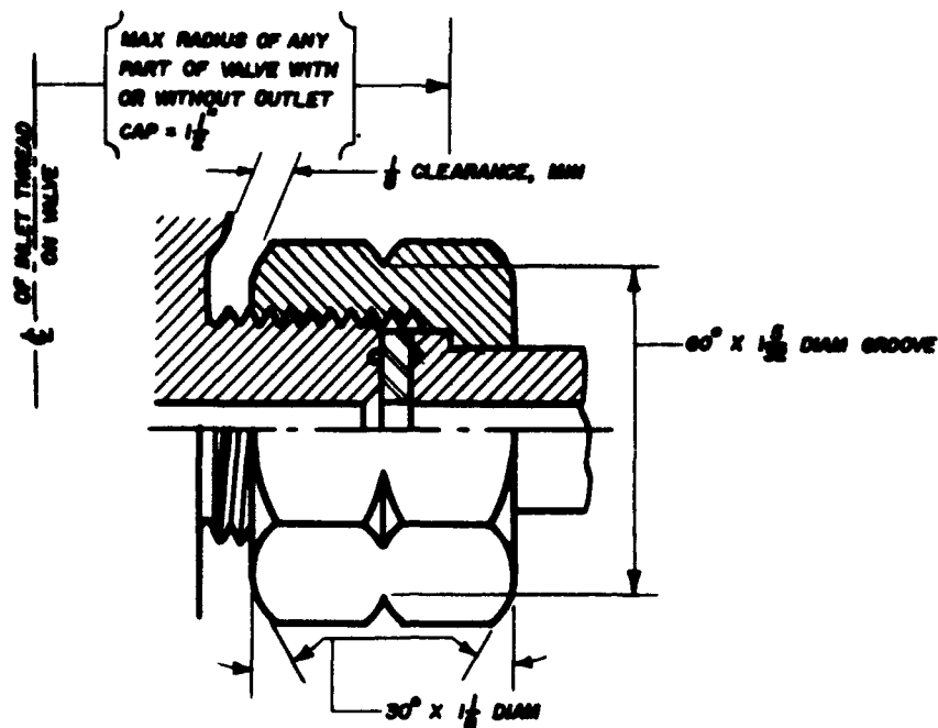
CONNECTION NO. 330
