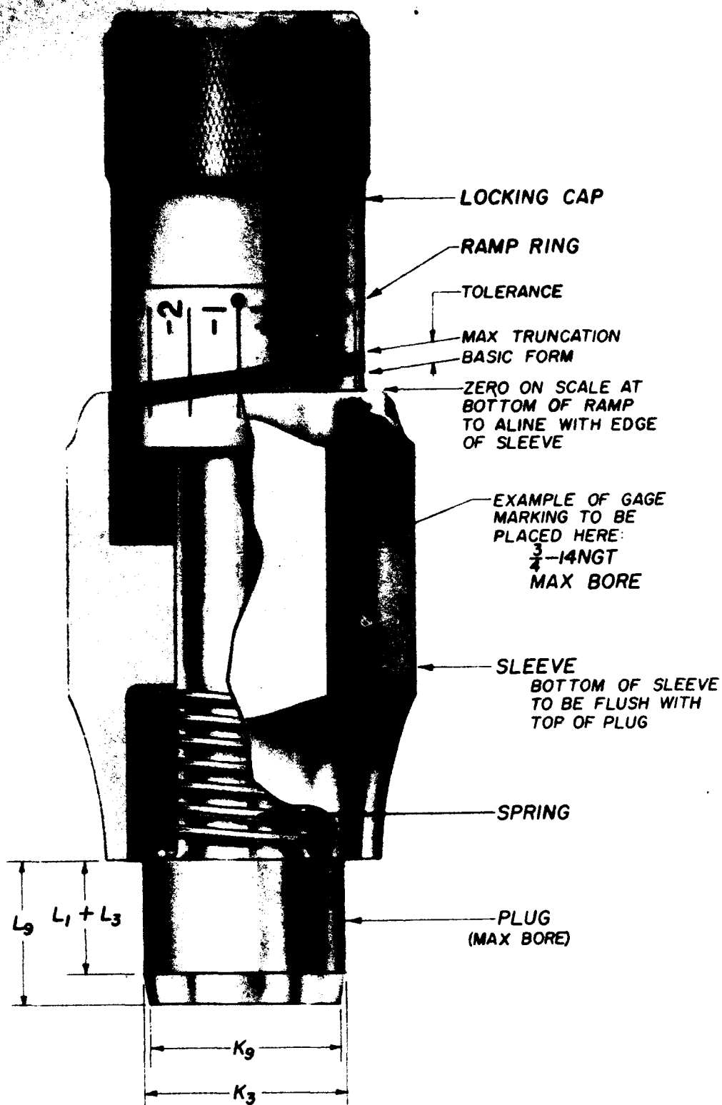
FIGURE IX.41.—Maximum bore plug gage; NGT, SGT.
