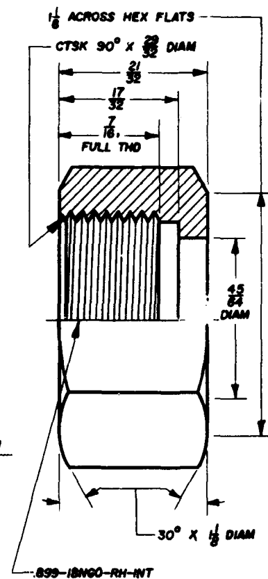
HEX NUT NO. 524
