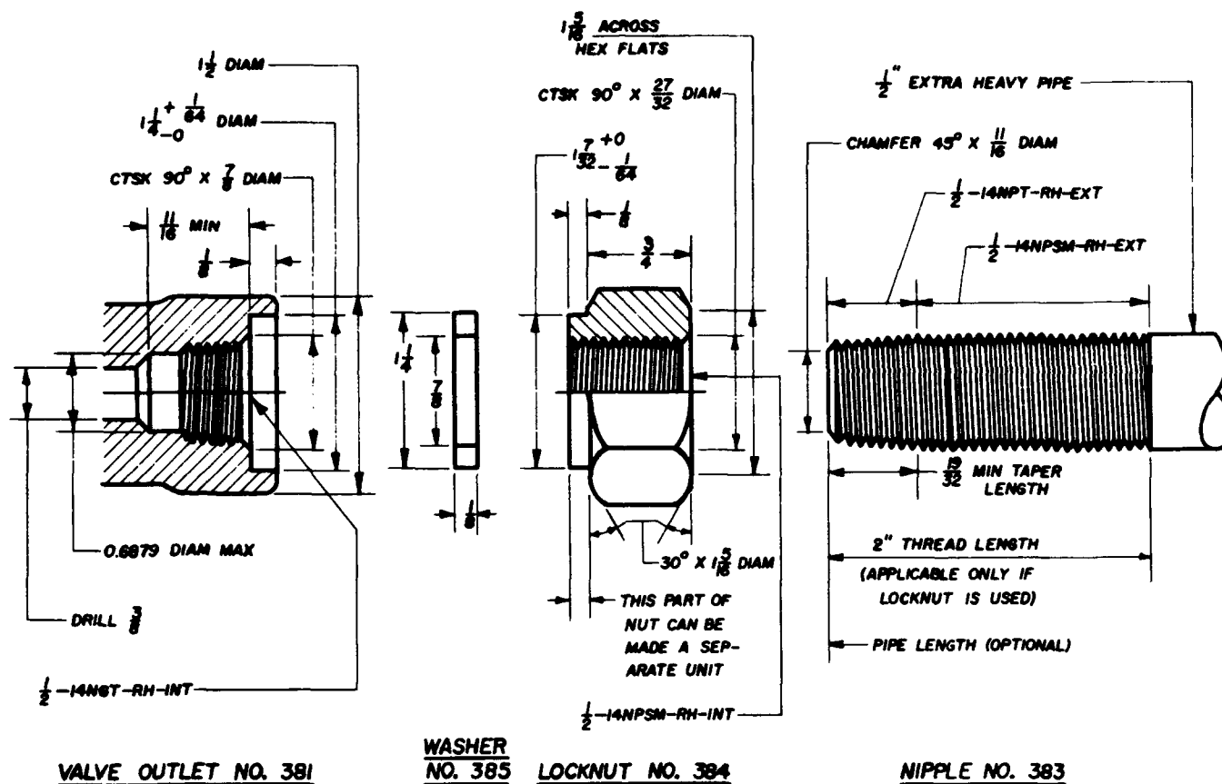
PLAIN PIPE CONNECTION
