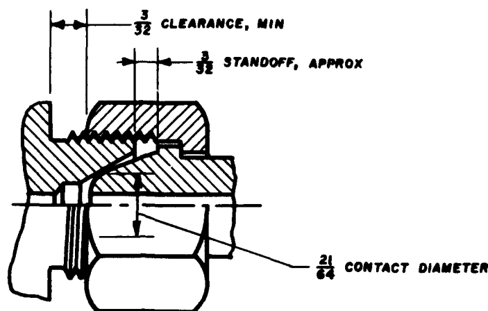
CONNECTION NO. 200
