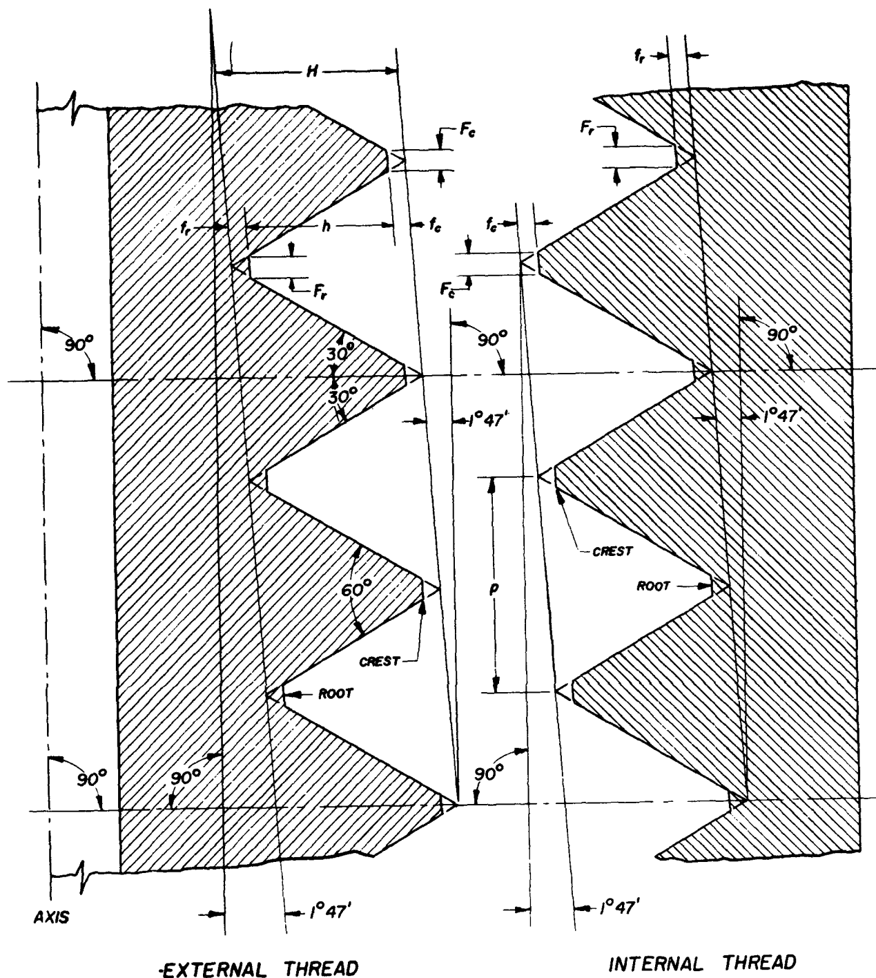
FIGURE VII.1.—Basic form of American Standard taper pipe thread
