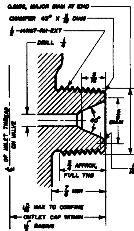
VALVE OUTLET NO. 341
