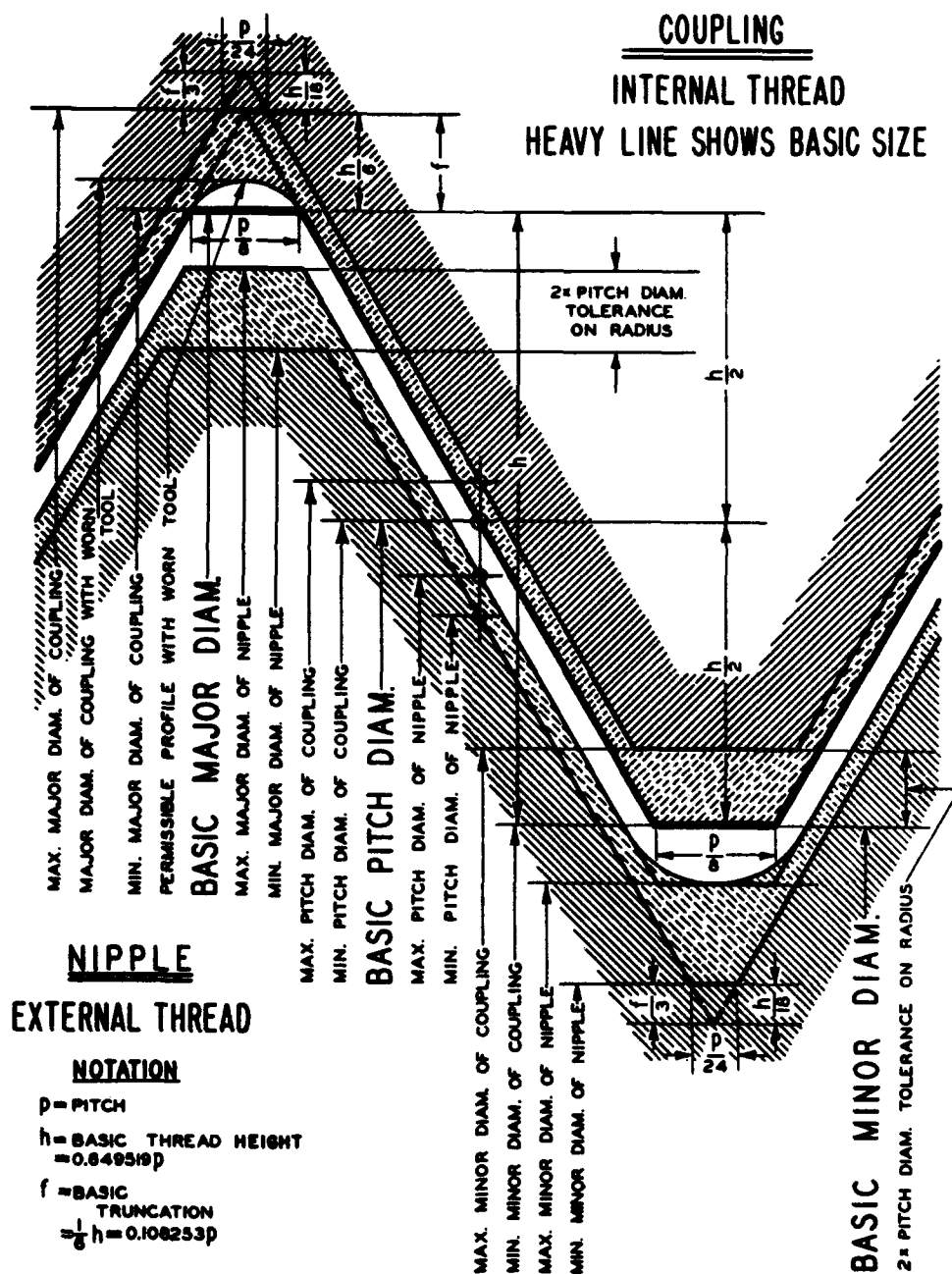
FIGURE X.1.—American National hose coupling and fire-hose coupling form of thread, NPSH and NH.
