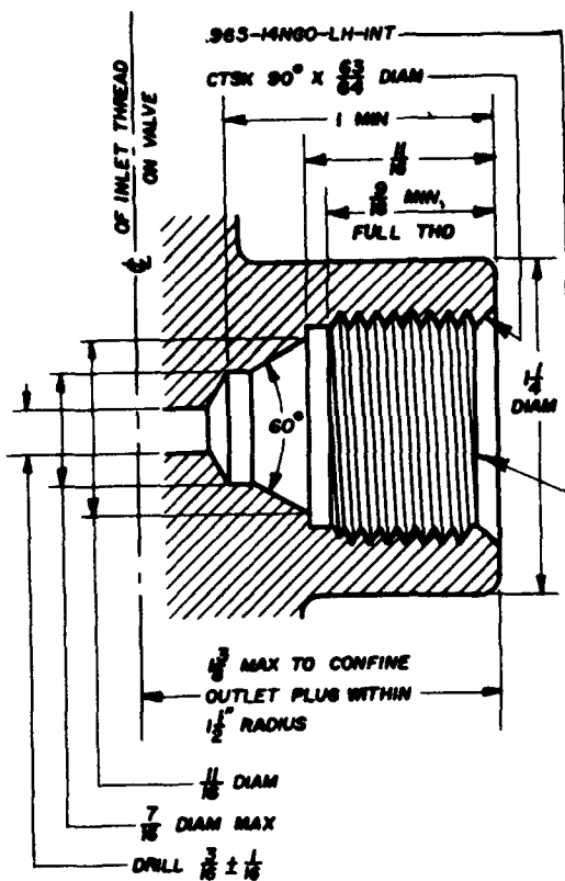
VALVE OUTLET NO. 591
