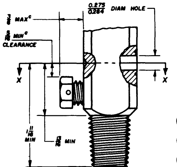
VALVE OUTLET
