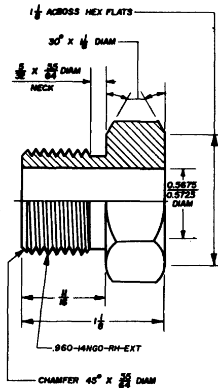
HEX NUT NO. 584
