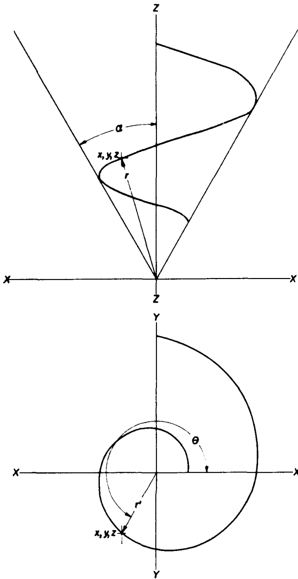
FIGURE 8.2.—The conical helix.
