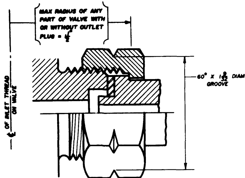
CONNECTION NO. 670
