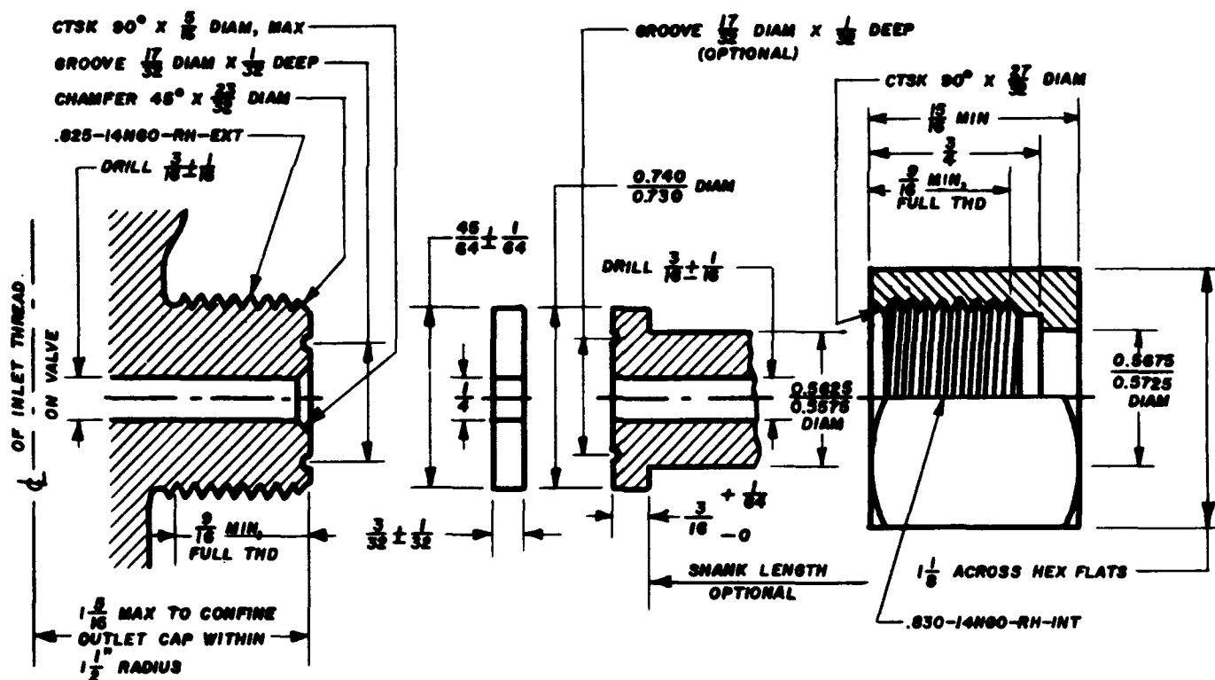
VALVE OUTLET NO. 321
