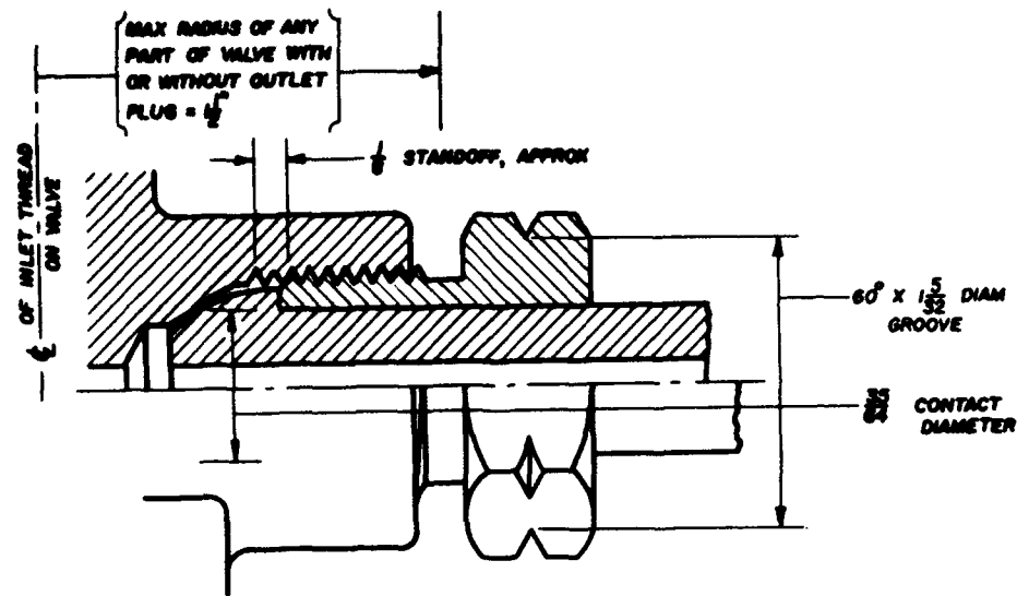
CONNECTION NO. 590
