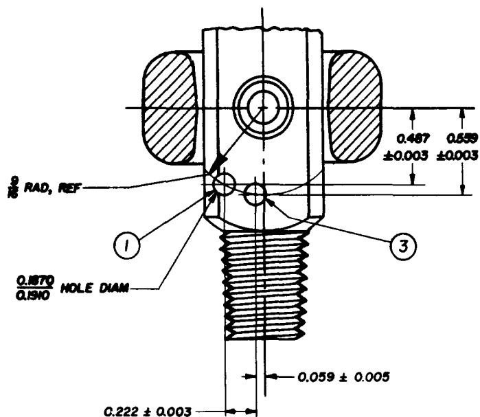
VALVE OUTLET NO. 901
