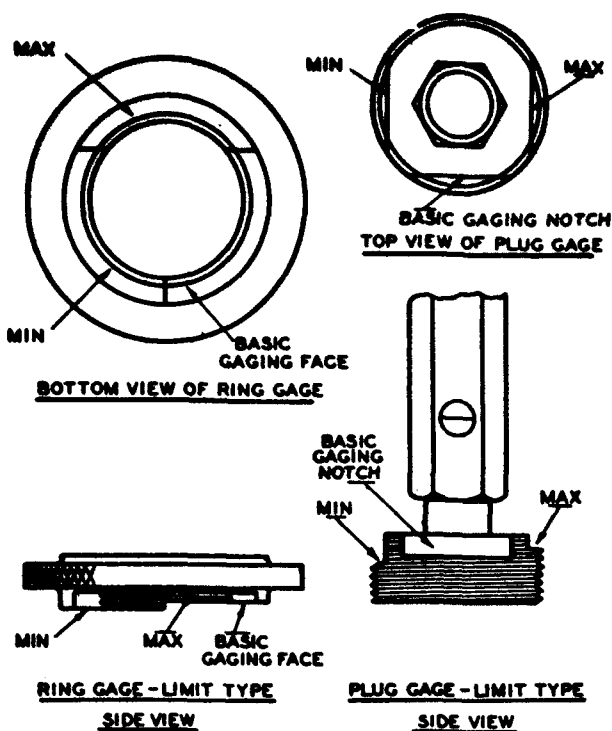
FIGURE VII.6.—Alternative form of taper pipe thread limit plug and thread ring gages.
