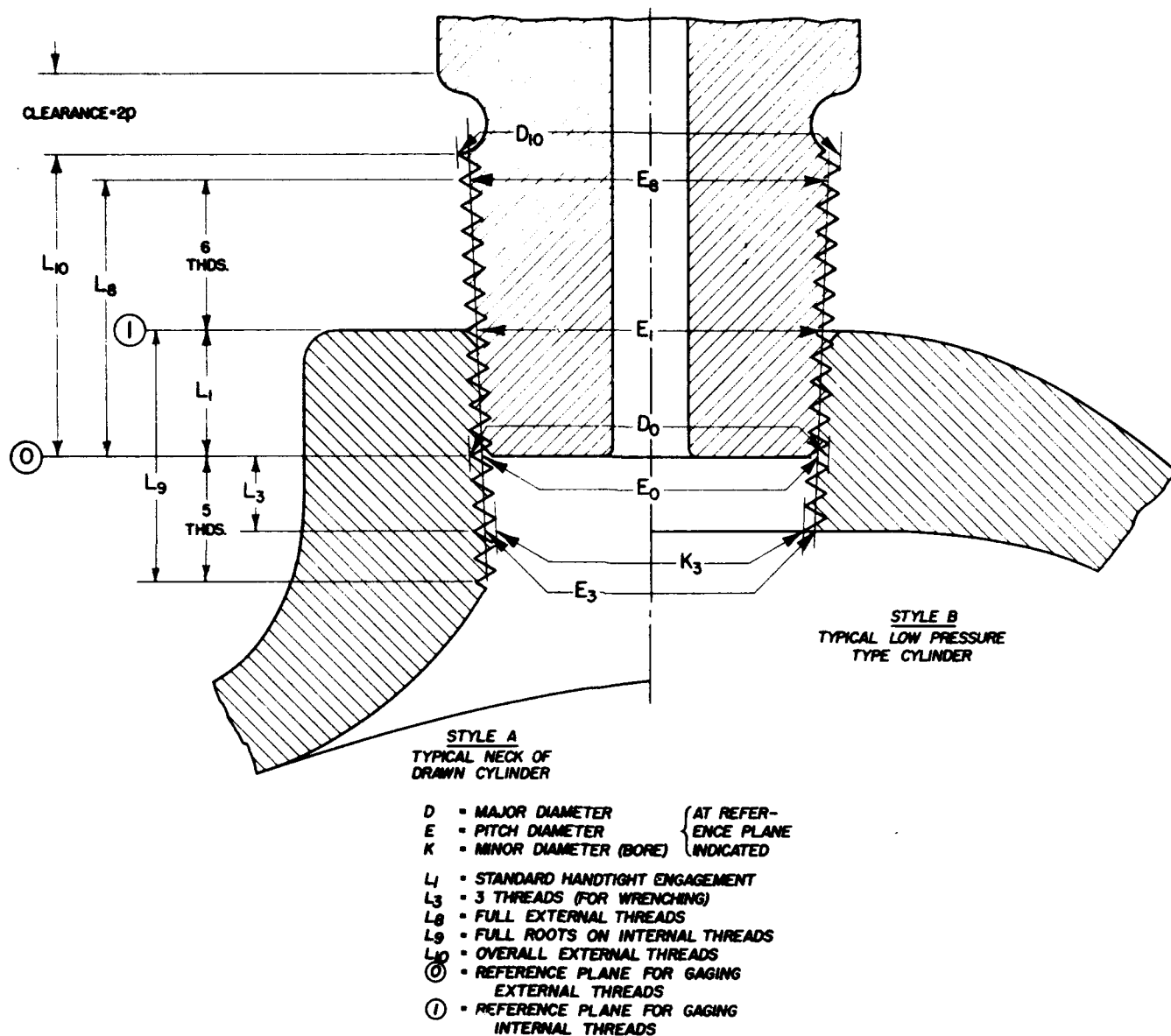
FIGURE IX.35.—Relationship between internal and external thread dimensions of NGT, NGT(Cl), and SGT threads.
