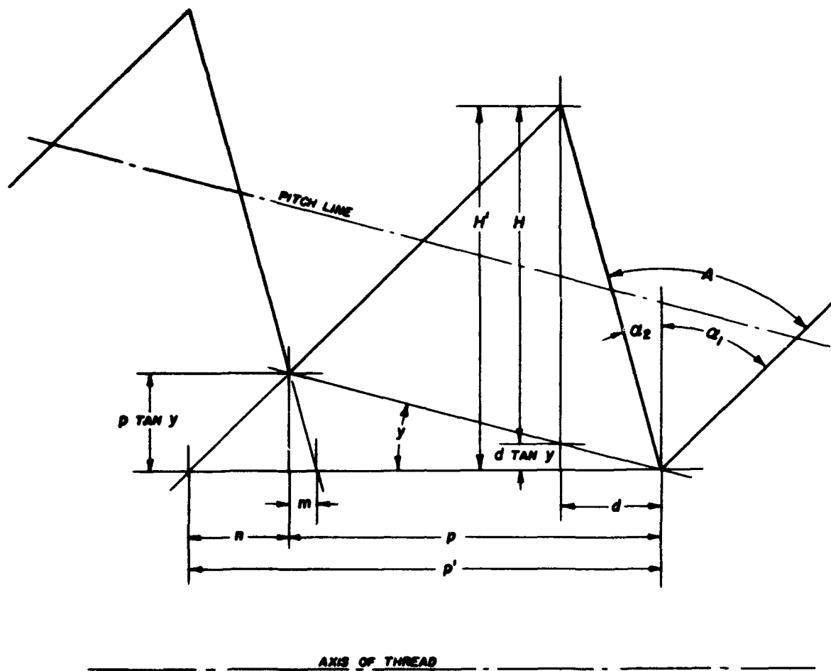
FIGURE 8.3.—Geometry of unsymmetrical taper screw thread.
