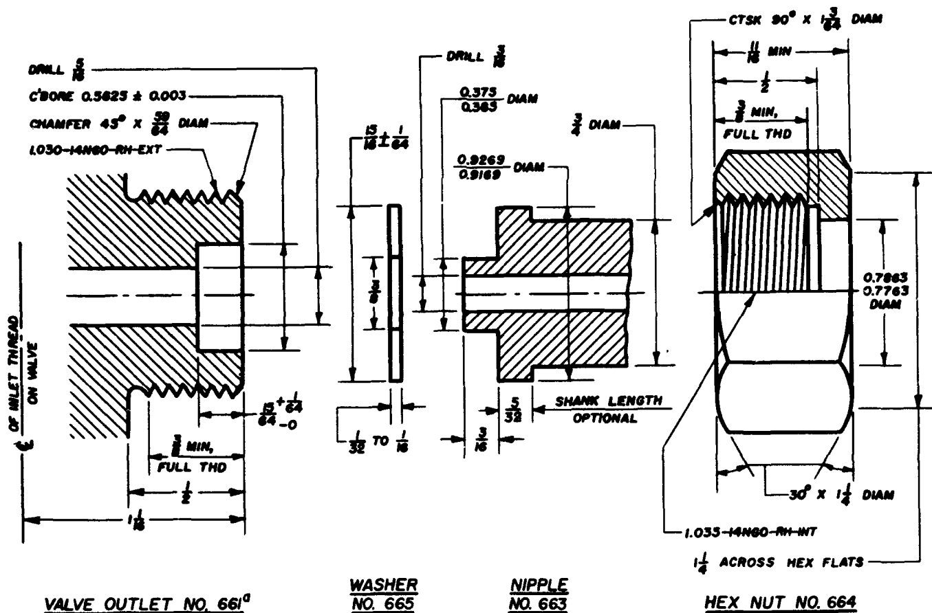
CONNECTION NO. 660
