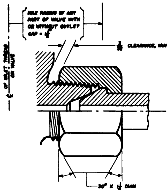
CONNECTION NO. 340
