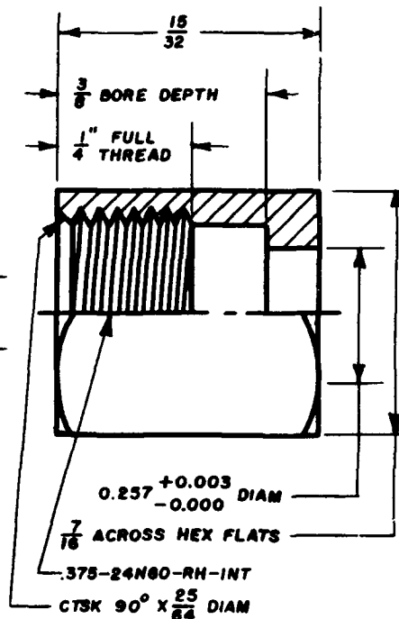
HEX NUT NO. 124
