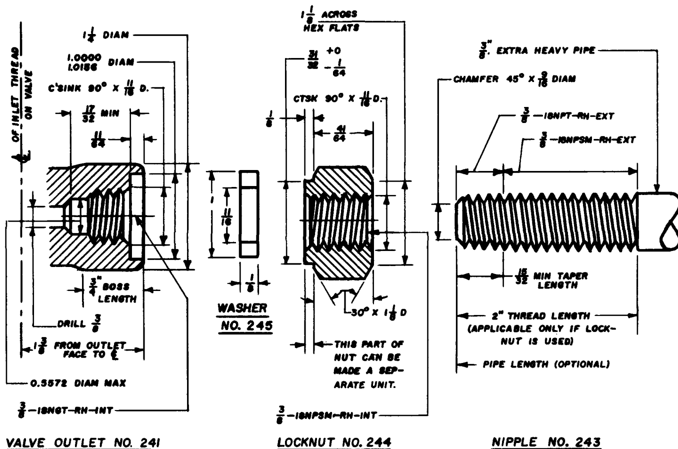
PLAIN PIPE CONNECTION
