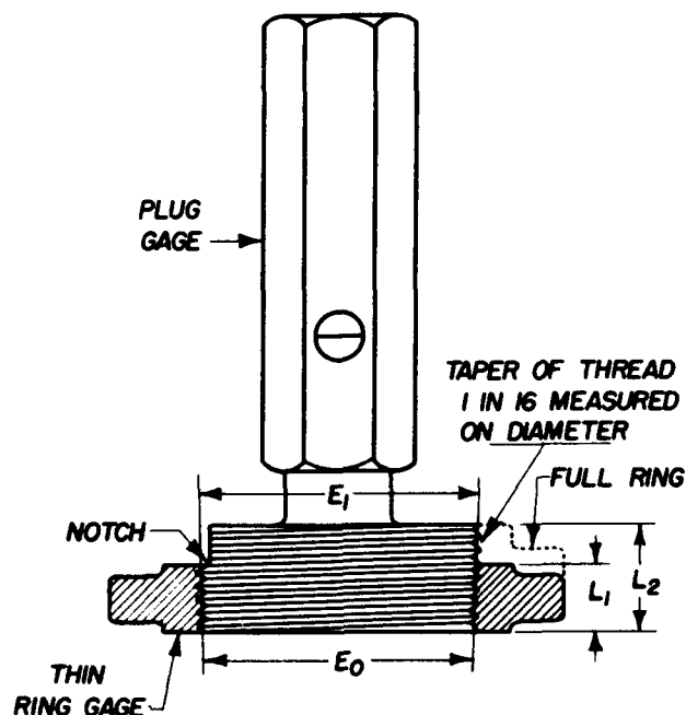
FIGURE VII.4.—American Standard taper pipe thread plug and thin ring gages.
