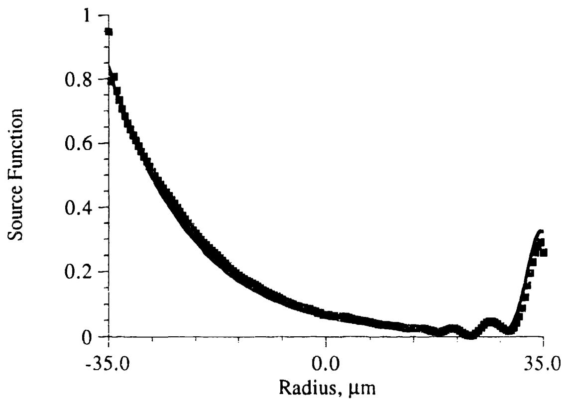
Fig. 6. Source functions calculated along the z-axis from numerical (points) and Mie (solid line) solutions for Debye amplitude functions for a water drop of diameter 70\text{ }\mu\text{m} surrounded by air, illuminated by a 10.591\text{ }\mu\text{m} polarized plane wave (example IV in Table I).
