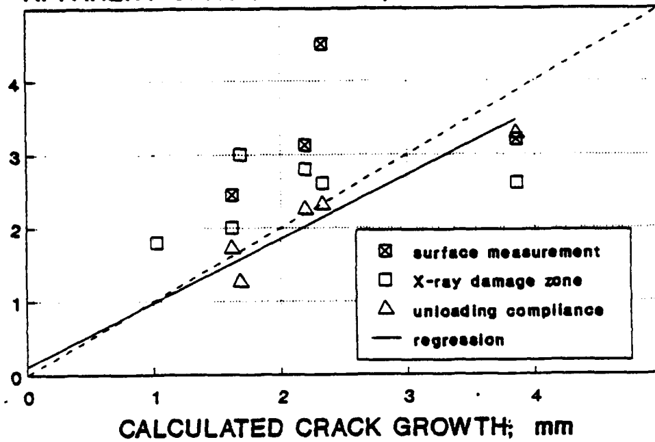
Figure 5. Comparison of crack growth by various determinations.
