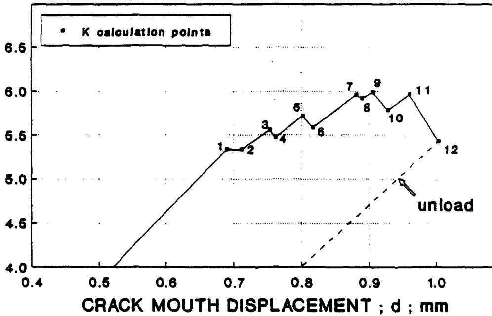
Figure 6. Load versus crack-mouth displacement behavior: specimen #8.
