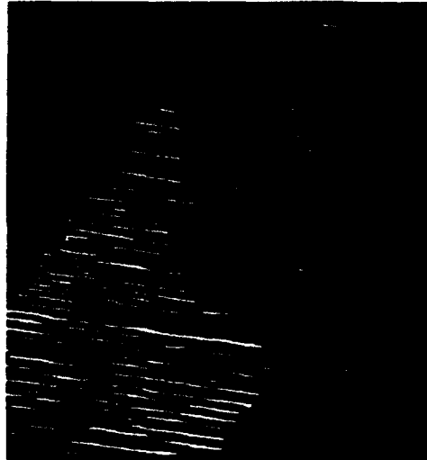
Figure 3. Microcrack Shapes Extracted From Figure 2 Using Morphology Based Image Processing Algorithm
