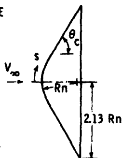
(a) FREE-STREAM CONDITIONS AND BODY SHAPE
