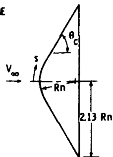
(a) FREE-STREAM CONDITIONS AND BODY SHAPE
