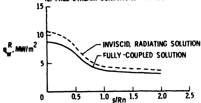
(b) COMPARISON OF RADIATIVE HEATING
