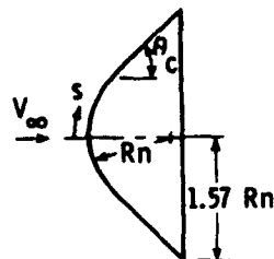
(a) FREE-STREAM CONDITIONS AND BODY SHAPE
