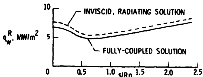
(b) COMPARISON OF RADIATIVE HEATING
