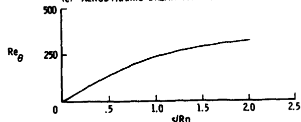
(f) MOMENTUM THICKNESS REYNOLDS NUMBER DISTRIBUTION
