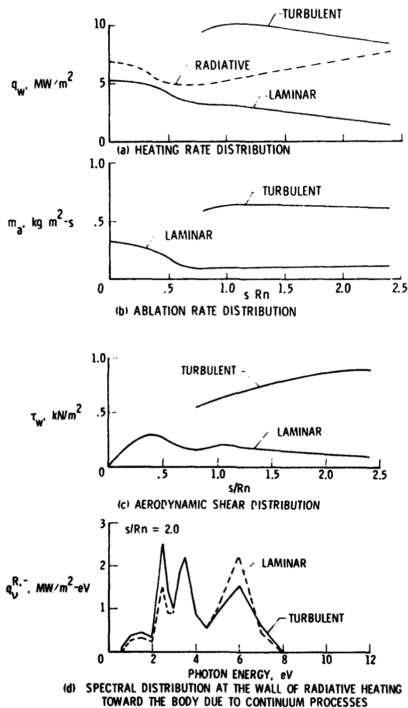
Figure 5.- Comparison between a turbulent and laminar boundary layer for fully coupled solution for large probe.
