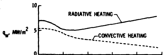
(c) RADIATIVE AND CONVECTIVE HEATING DISTRIBUTION
