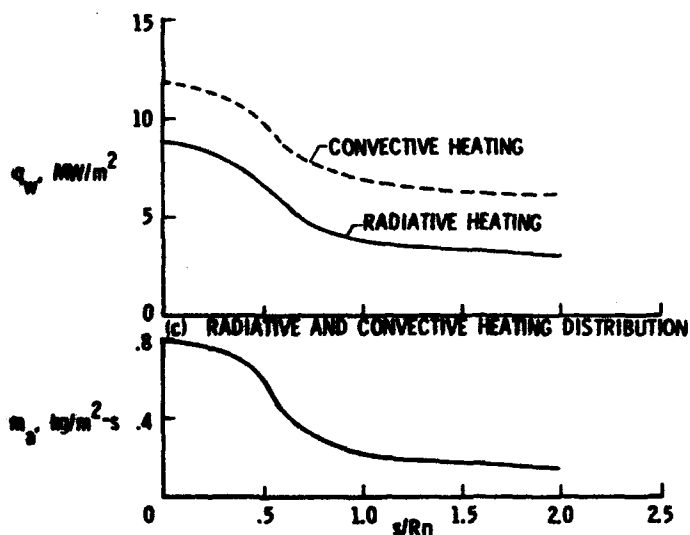
(c) RADIATIVE AND CONVECTIVE HEATING DISTRIBUTION
