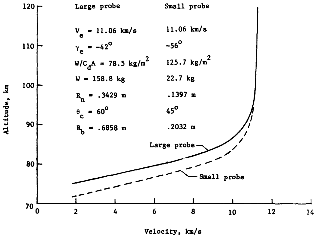
(a) Type I probes
