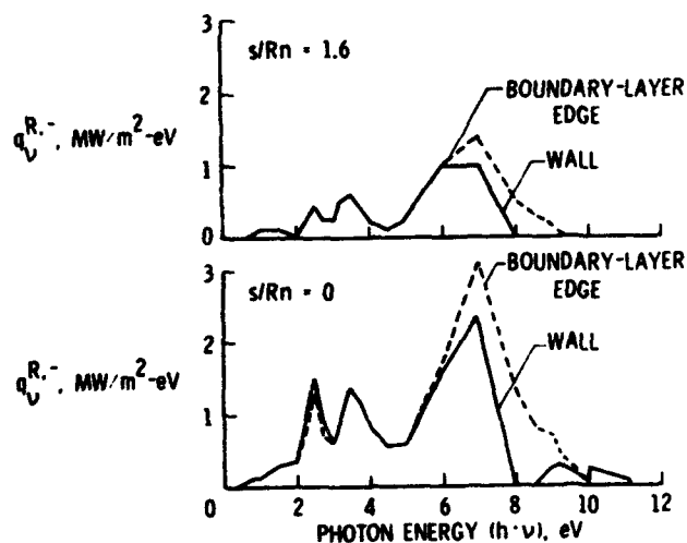
(g) SPECTRAL DISTRIBUTION OF RADIATIVE HEATING TOWARD THE BODY DUE TO CONTINUUM PROCESSES
