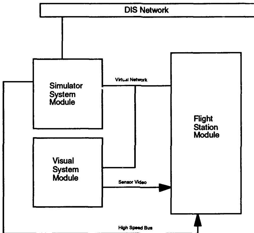
Figure 1.3-2 ARWA Simulator Subsystem Architecture
