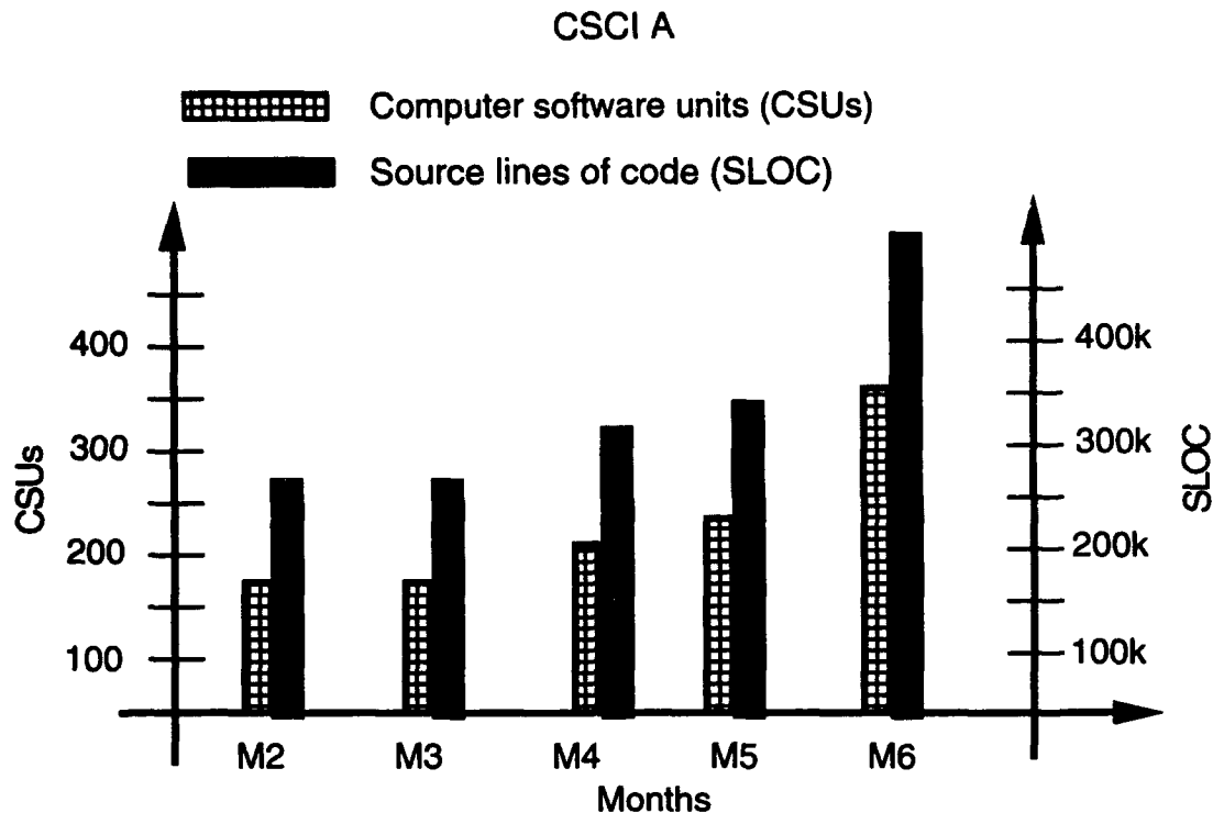
Figure 3-7 Sample CSCI Software Size Tracking
