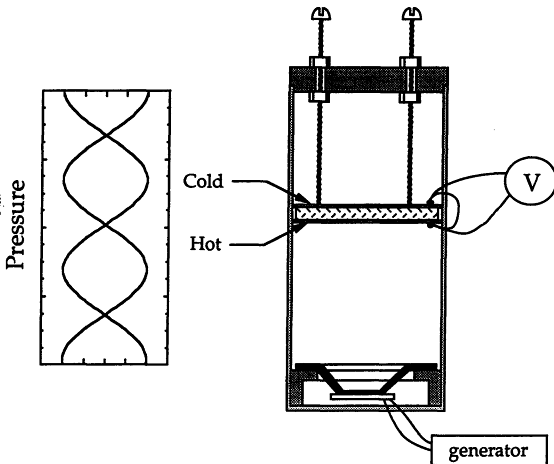
Fig. 3 Four to Five KiloHertz Refrigerator
