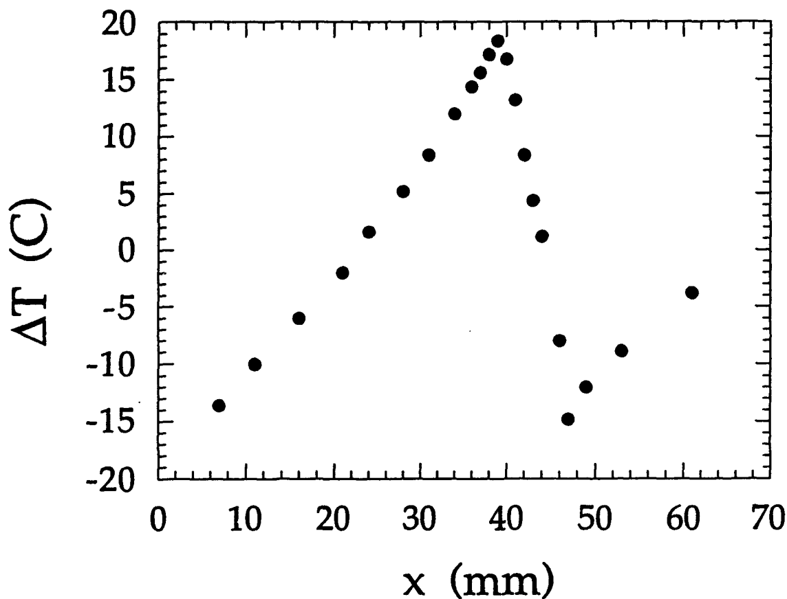
Fig. 4 Positon of stack on standing wave and its effect on \Delta T .
