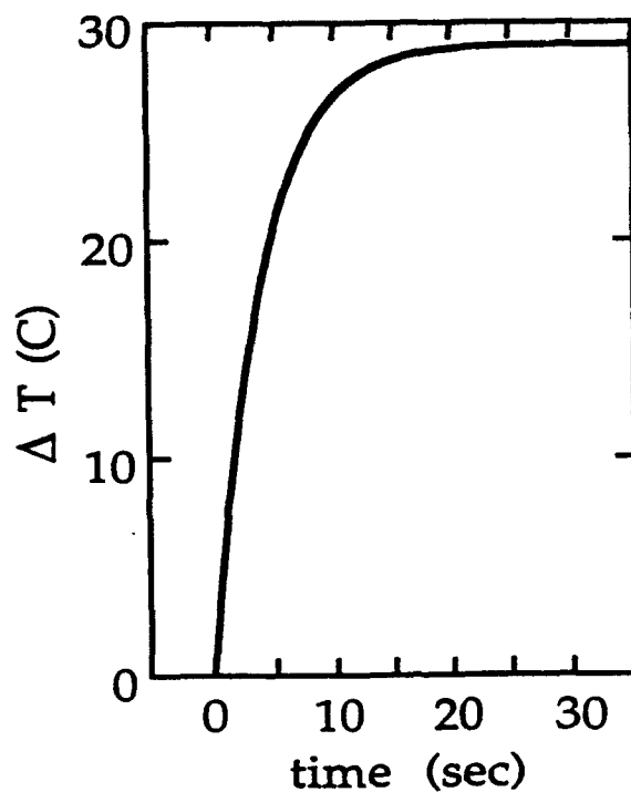
Fig. 5 Time dependence of \Delta T when driver puts out 160dB of sound at 4.2 kHz.
