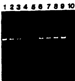
FIG. 3. Amplification of nahR from four sediment samples with nested primer PCR. For lanes 1, 3, 5, and 7, a 2- \mu l concentrated sample was used as a template for PCR amplification; and for lanes 2, 4, 6, and 8, a 2- \mu l 1:10 dilution of the same samples was used. Lanes: 1 and 2, seep sediment; 3 and 4, upgradient sediment; 5 and 6, downgradient sediment; 7 and 8, source sediment; 9, positive control (part of a P. putida G7 colony added to the PCR mixture); 10, PCR negative control (reagent only).
