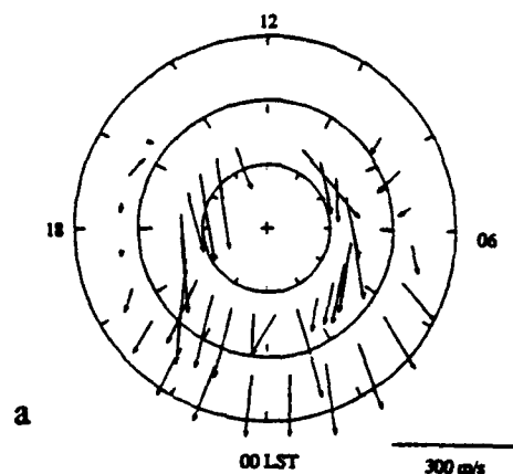
Thule and Sondrestrom – VSH winds, solar min., low K_p
