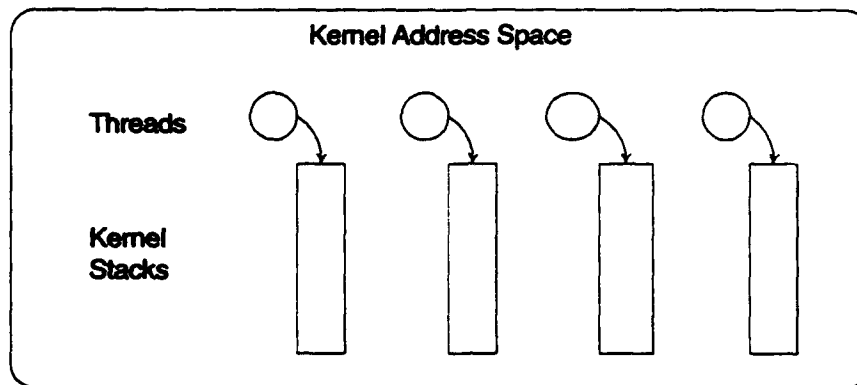
Figure 3-1: One Kernel Stack Per Thread
