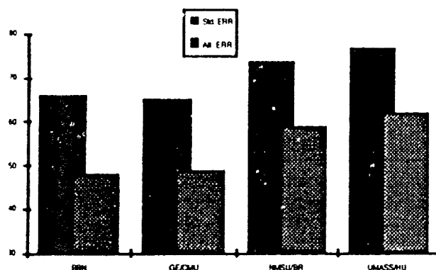
Figure 4. Tipster system MUC-5 EME scores for two formulations of error per response fill
