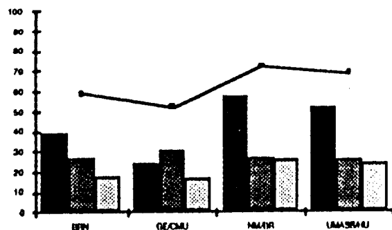
Figure 7. Tipster system scores for the EJV core-template test
