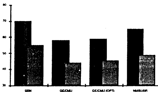
Figure 5. Tipster system MUC-5 JME scores for two formulations of error per response fill
