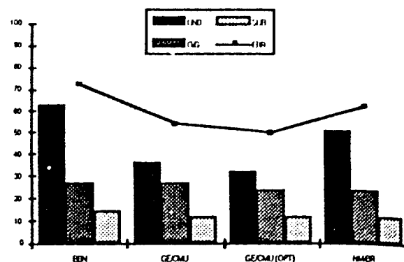
Figure 8. Tipster system scores for the JJV full-template test
