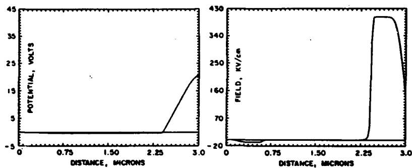
Figure 3c. Potential and electric field distribution at 21 v.
