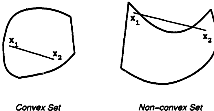
Figure 7: Convex sets.
