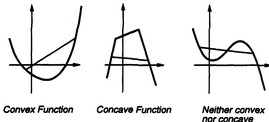
Figure 8: Convex Functions
