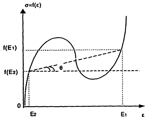
Fig. 1. The stress-strain curve for the shape-memory fibers.
