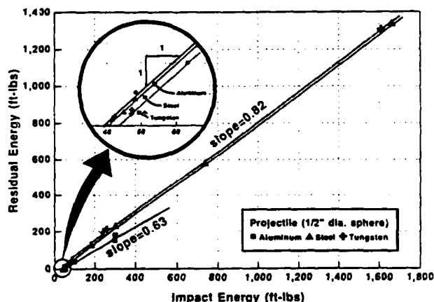
Figure 1. Deviations in the E_i vs. E_r slope as a function of kinetic energy possessed by aluminum, steel, and tungsten impactors.
