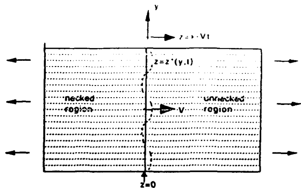
Fig. 2. A schematic sketch of a propagating neck in a uniaxially reinforced sheet.
