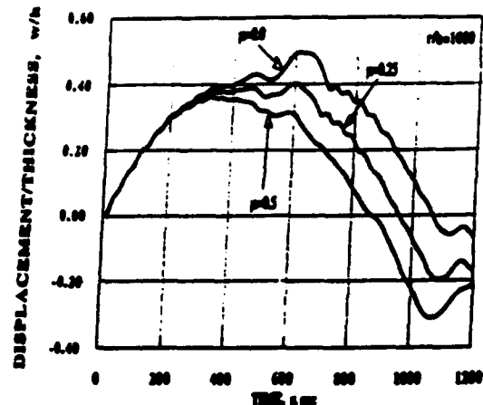
Fig. 3. Effect of simple geometric imperfections on central deflection for non-dimensional shell radius (r/h) = 1000 (plate thickness: 0.1345cm).
