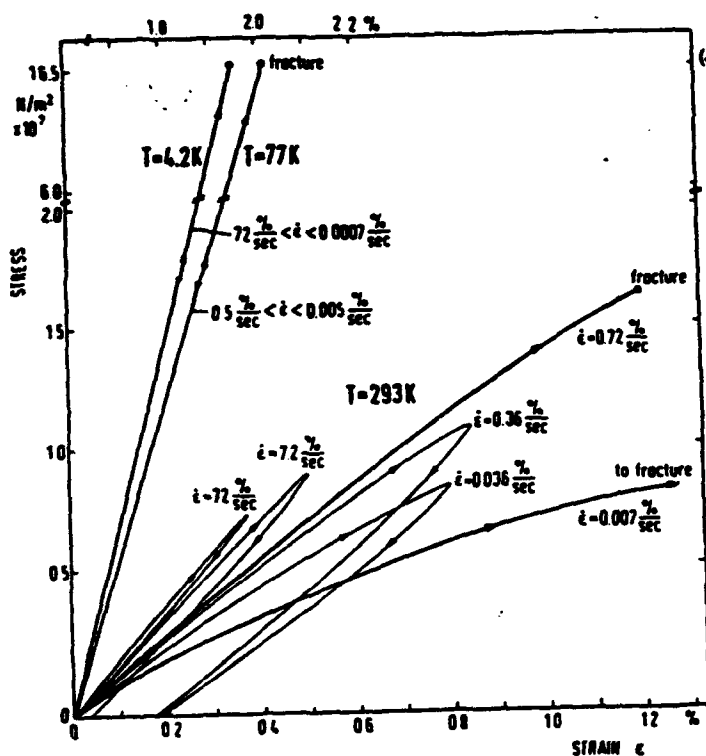
Figure 1. Stress-strain behavior of epoxy resins at different strain rates, \dot{\epsilon} , and temperatures, T (after Hartwig 1979).
