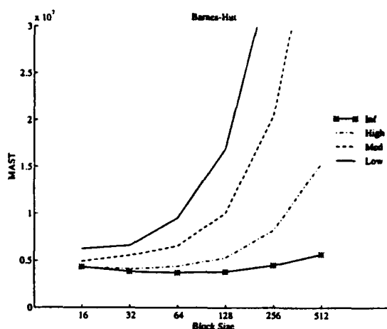
Figure 2: MAST of Barnes-Hut.
