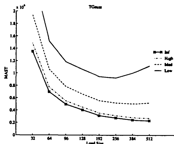
Figure 12: MAST of TGauss under sequential prefetching.
