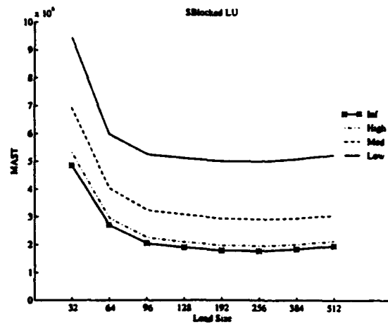
Figure 24: MAST of SBlocked LU under hybrid prefetching.
