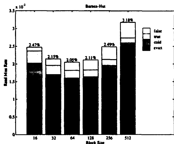
Figure 1: Read miss rate of Barnes-Hut.
