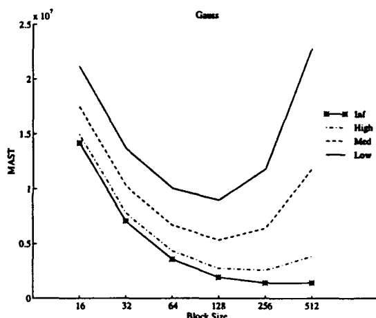
Figure 4: MAST of Gauss.
