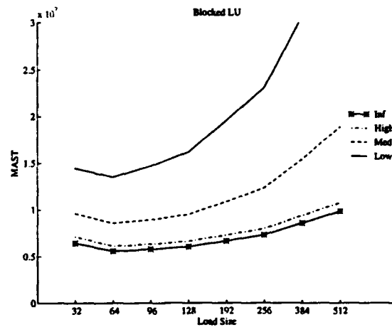
Figure 16: MAST of Blocked LU under sequential prefetching.
