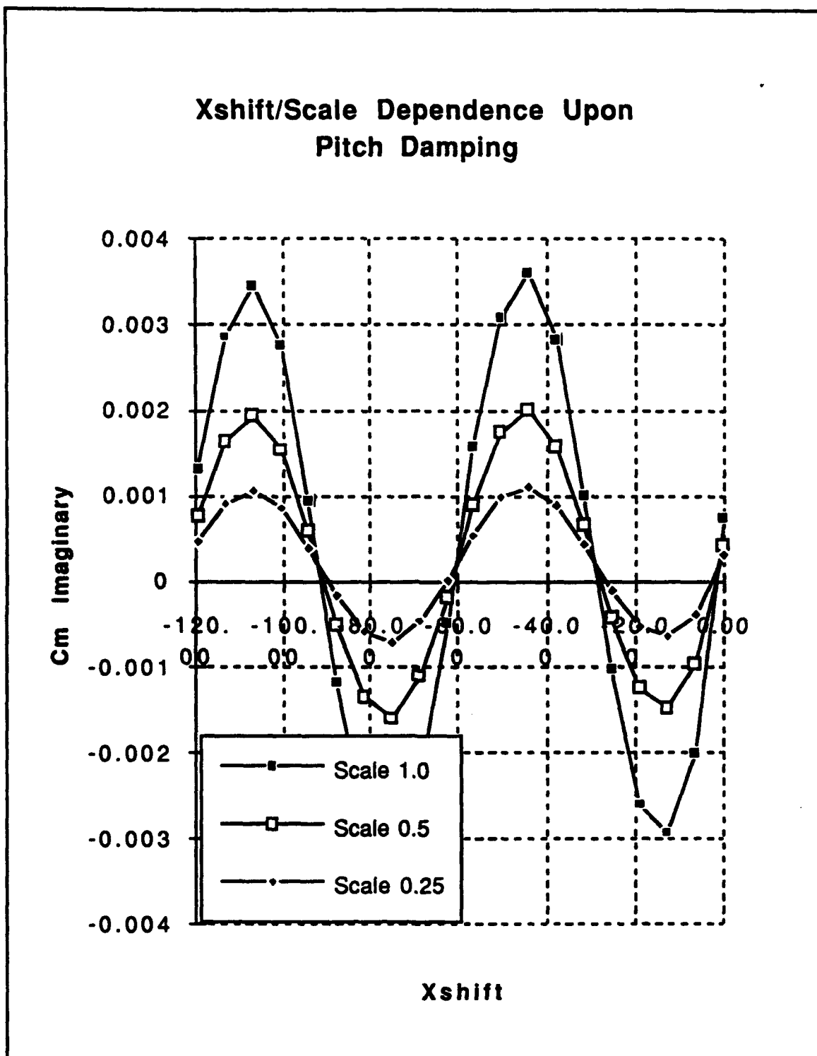
Figure 5.6 Xshift/Scale Dependence Upon Pitch Damping
