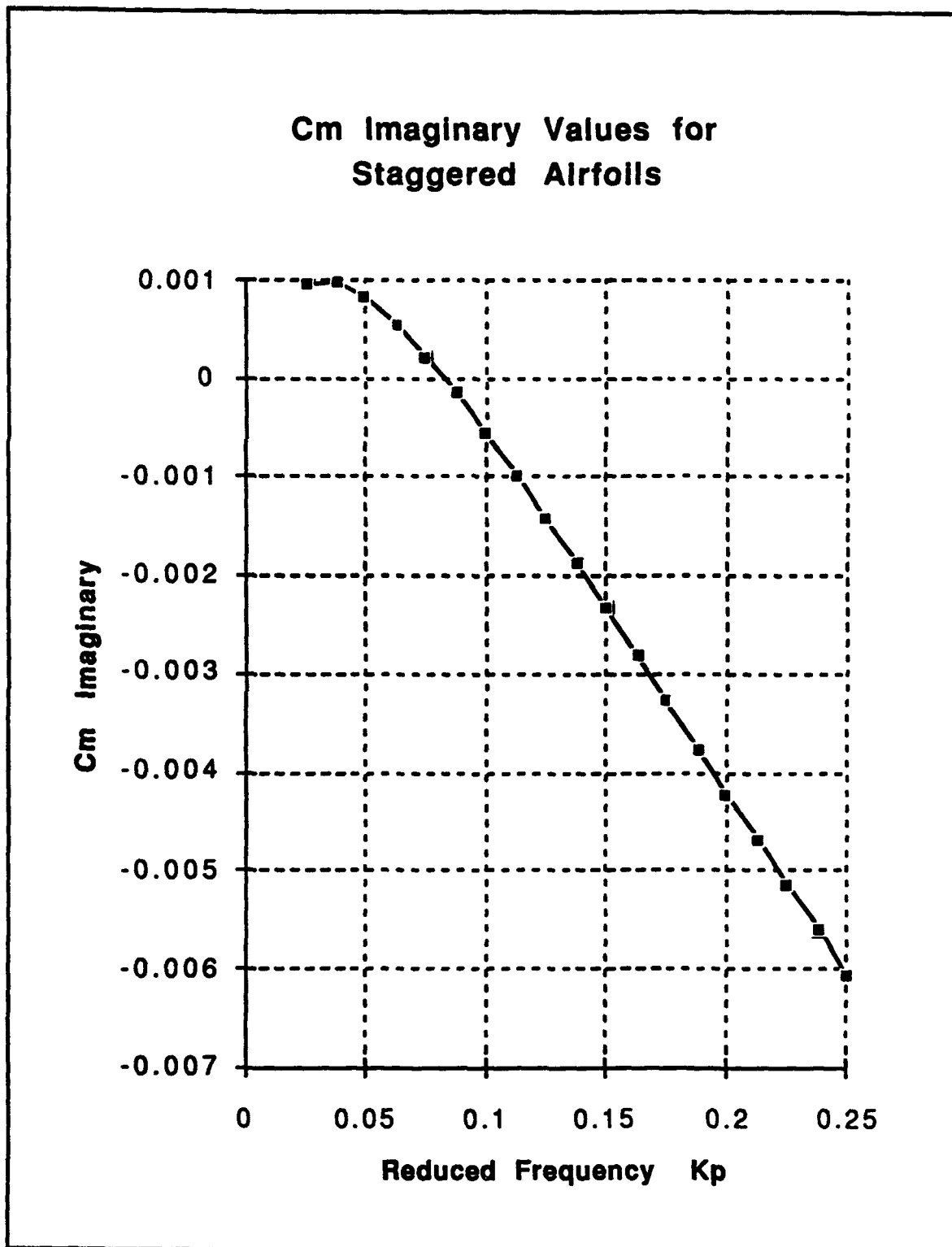
Figure 5.1 Frequency Dependence of Pitch Damping Xshift=-2, Yshift=-2
