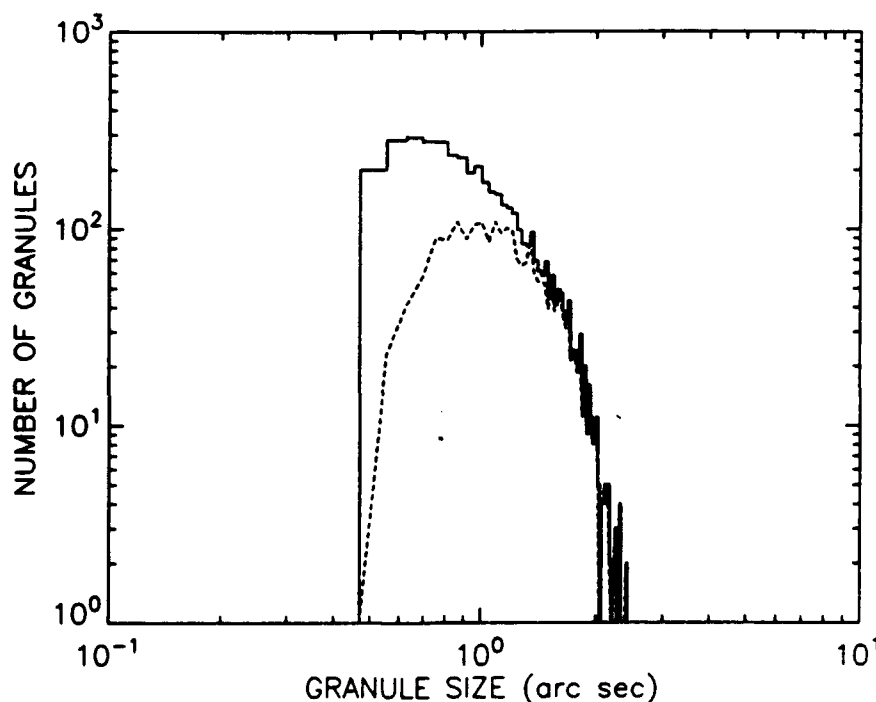
FIG. 17.—Histogram showing the size distributions of granules found by lane finding (solid lines), and by center finding (dashed lines)
