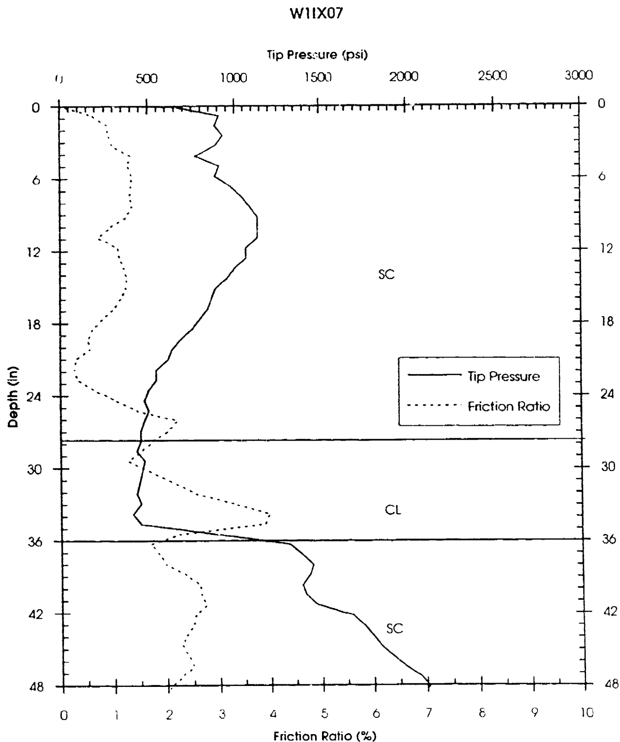
Figure D6. ECP TP and FR versus depth for W11X07
