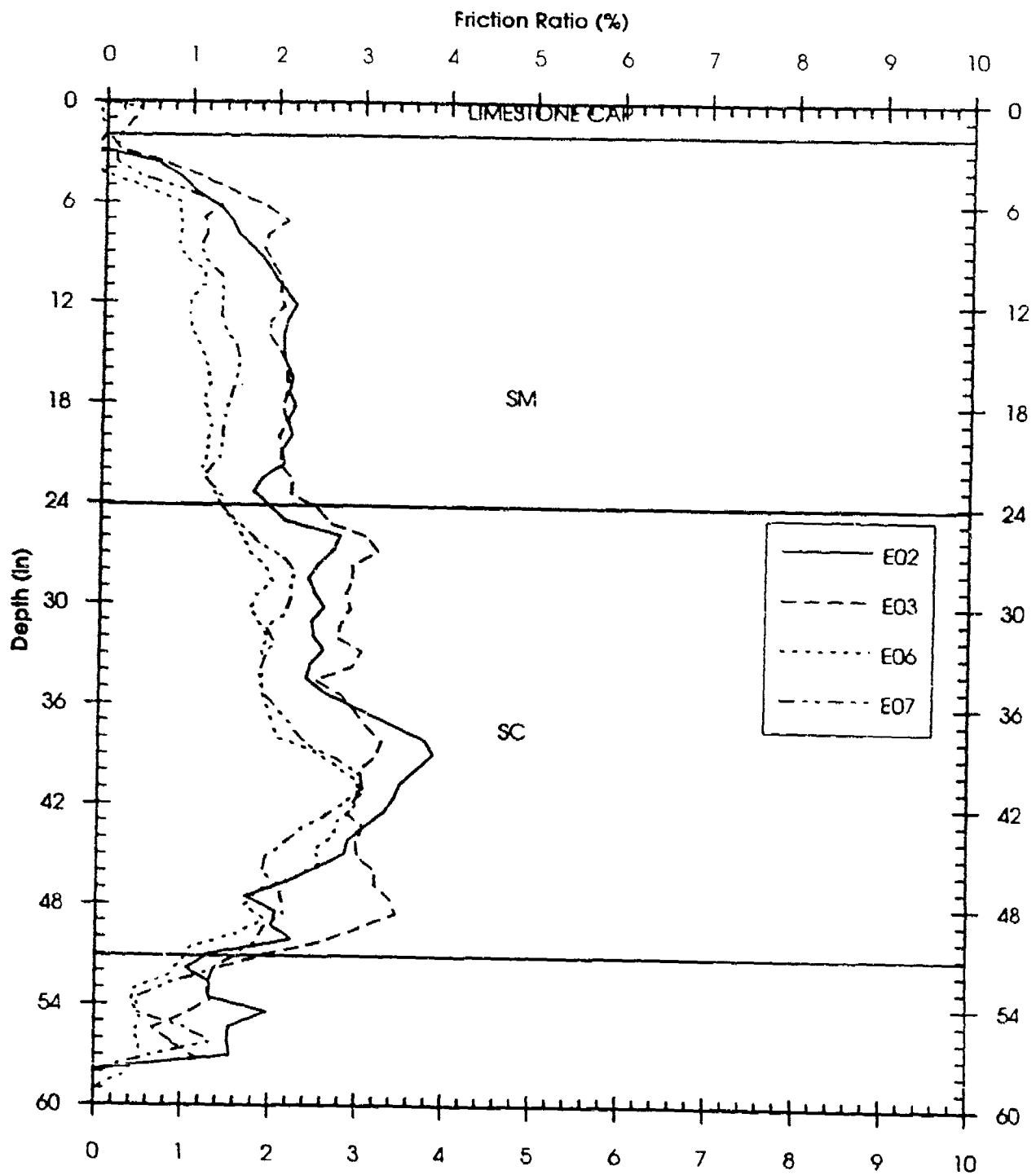
Figure F44. ECP FR versus depth for W4I10
