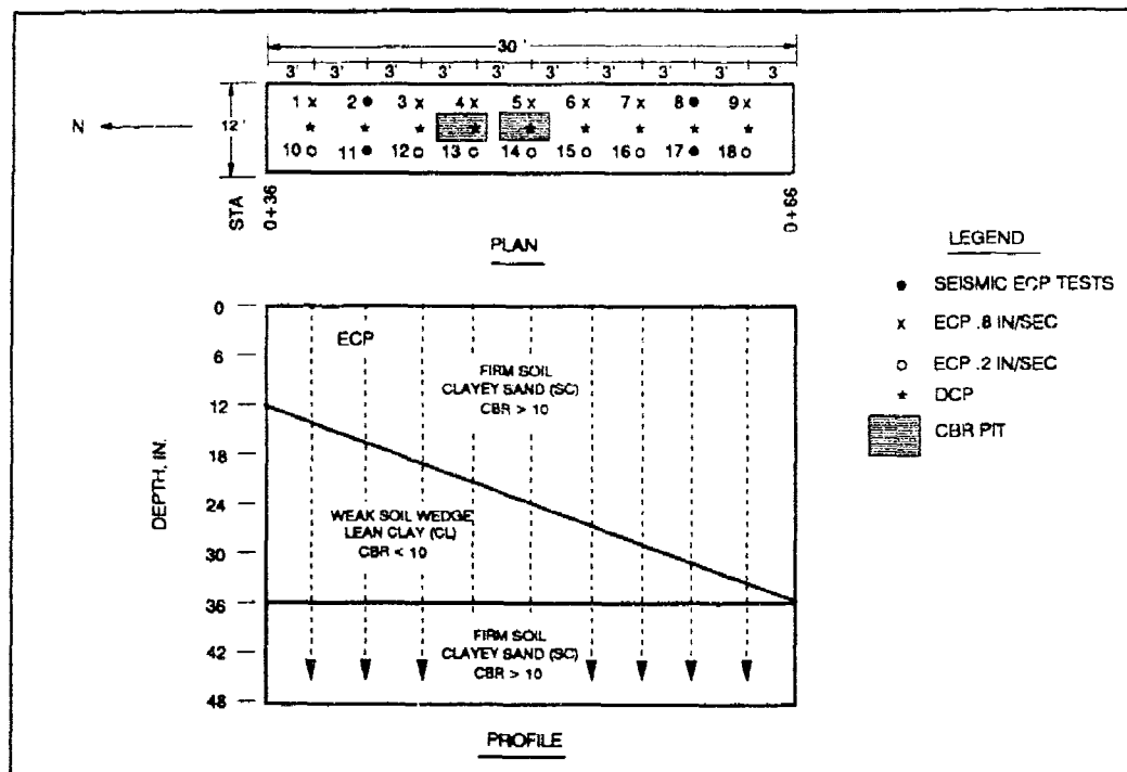
Figure 9. Plan and profile of test section 1 (soil wedge)
