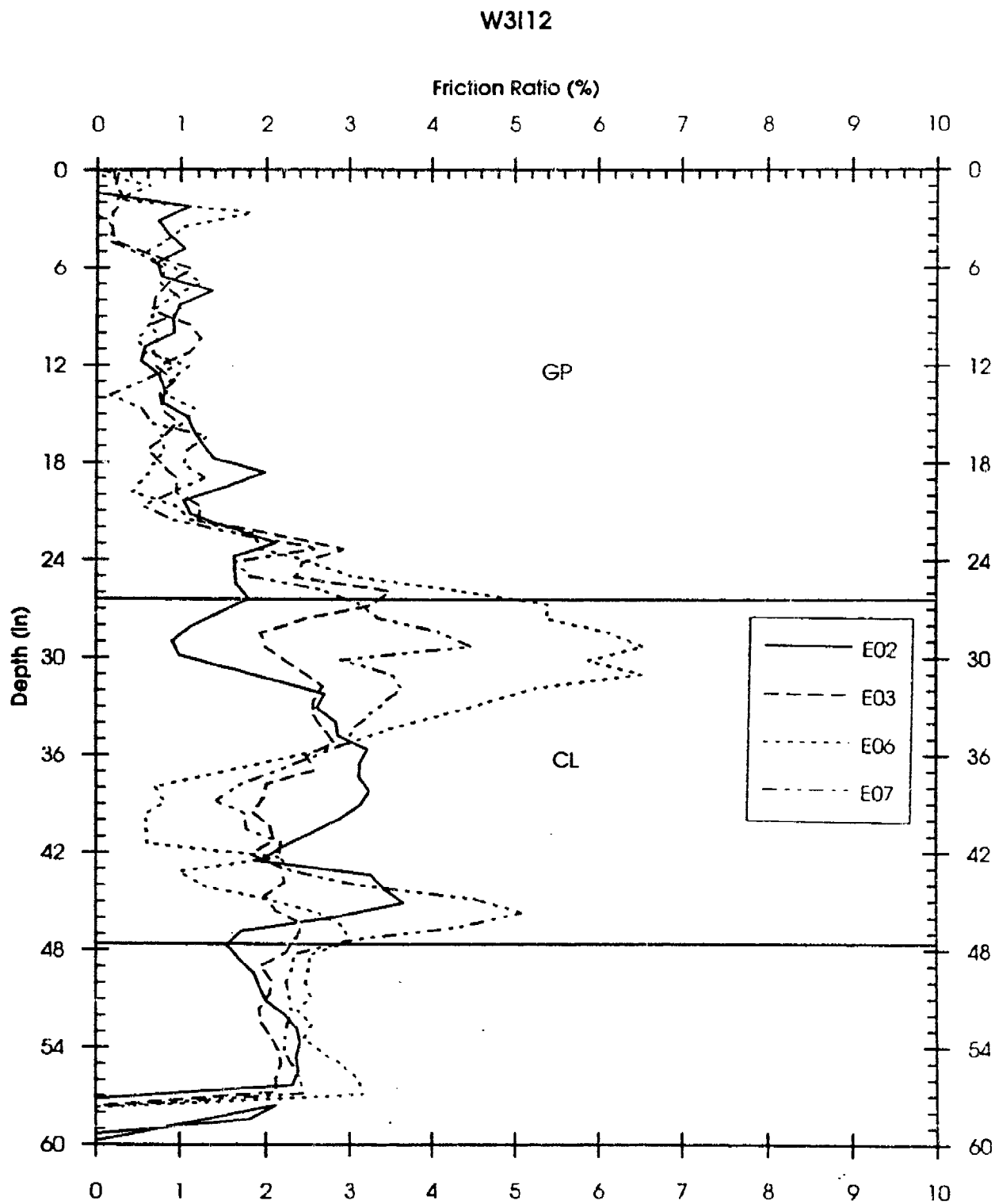
Figure F24. ECP FR versus depth for W3112
