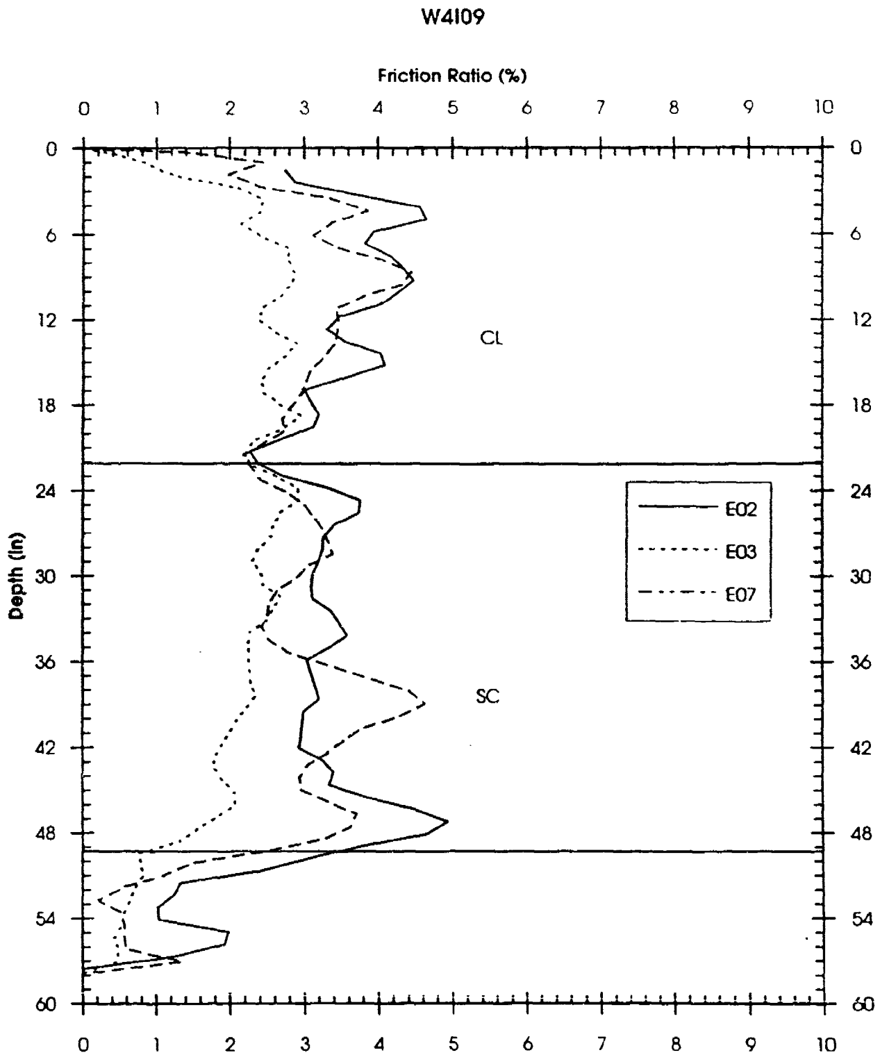
Figure F42. ECP FR versus depth for W409
