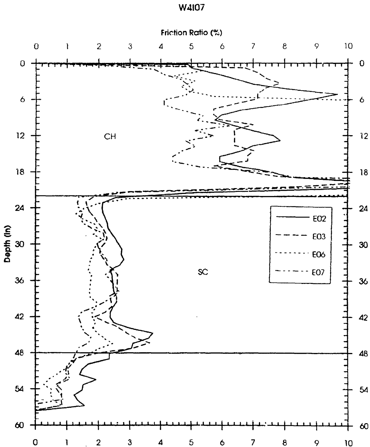
Figure F38. ECP FR versus depth for W4107
